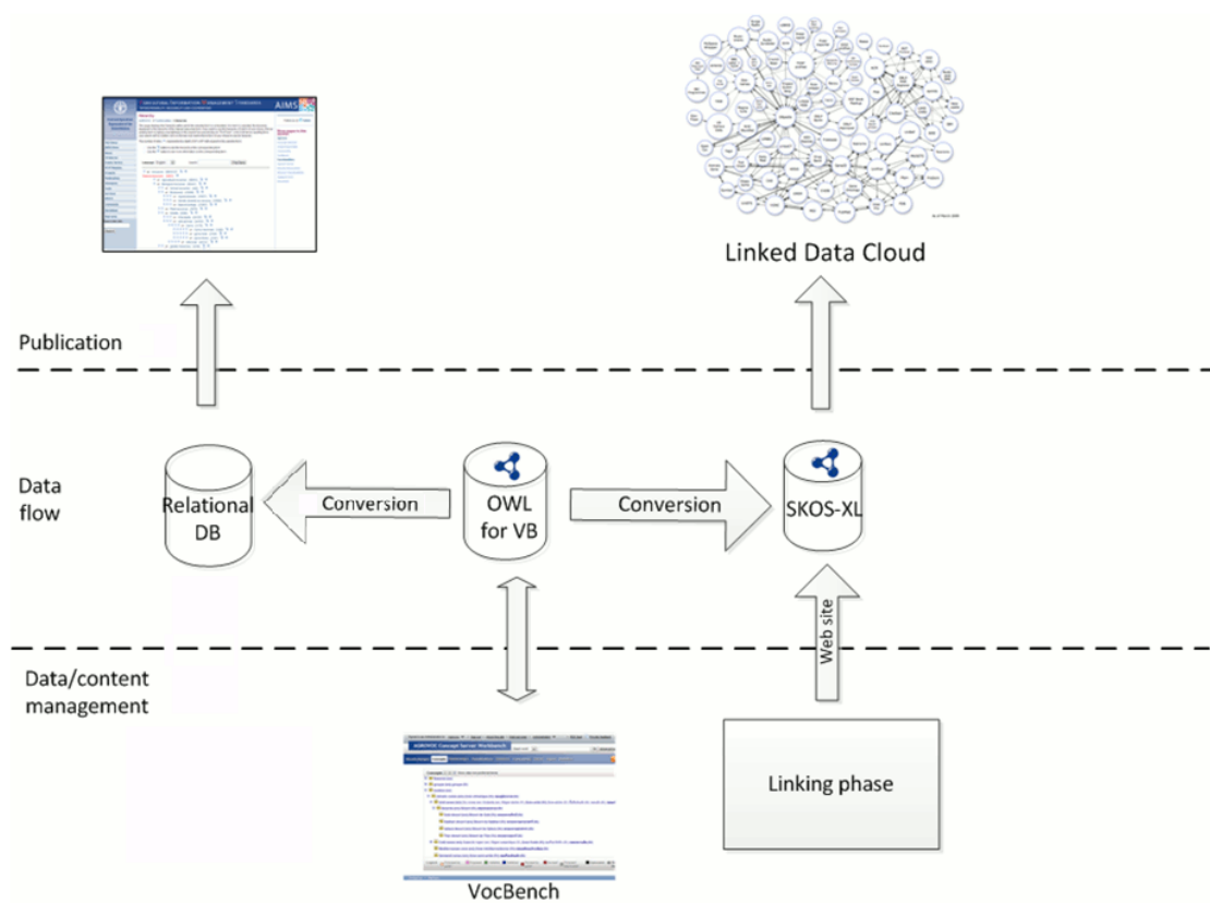
Figure 2. Overview of the process for publishing AGROVOC as linked data
