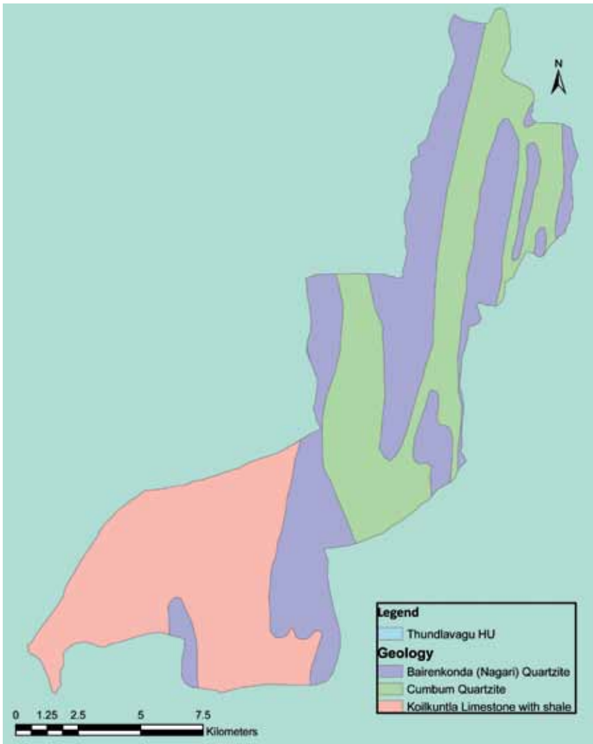
Geological map of Thundlavagu hydrological unit
