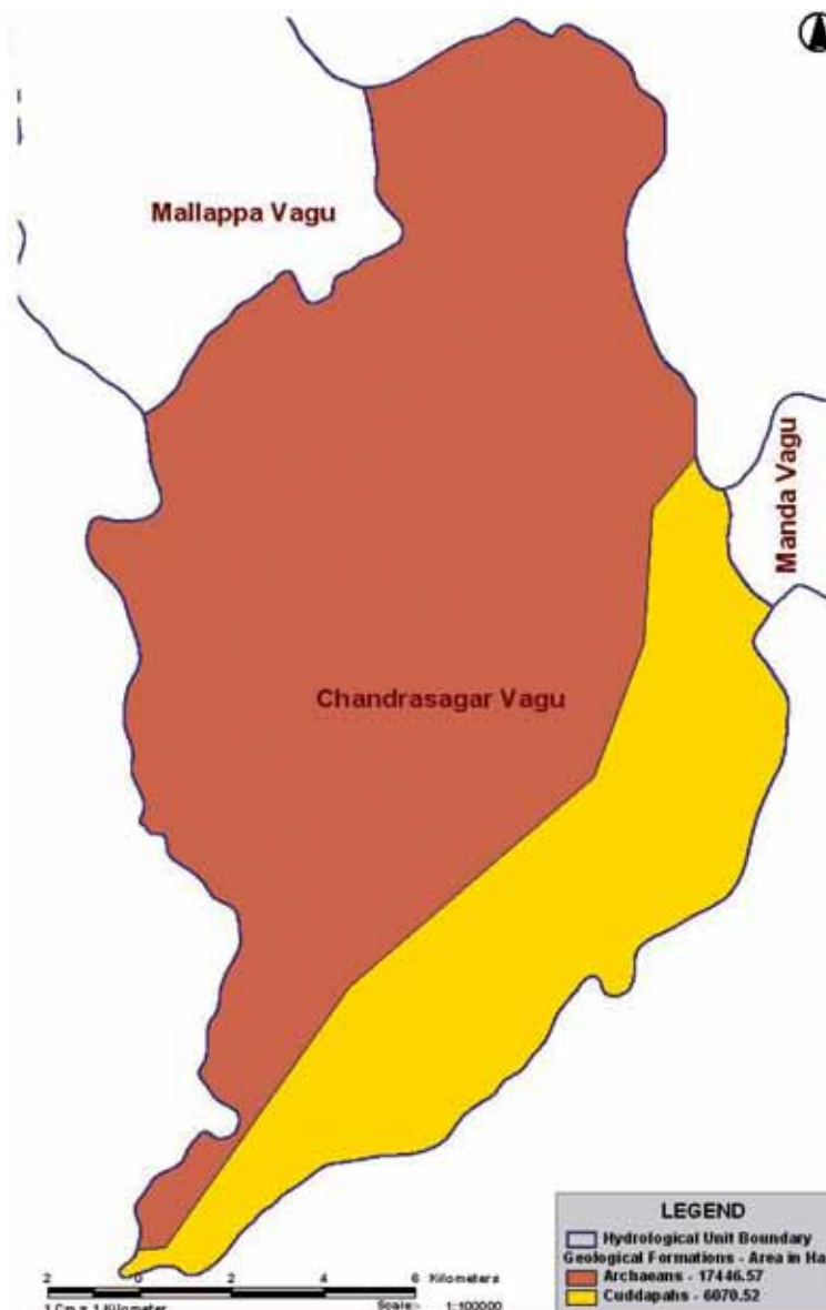
Geological map of Chandrasagarvagu hydrological unit
