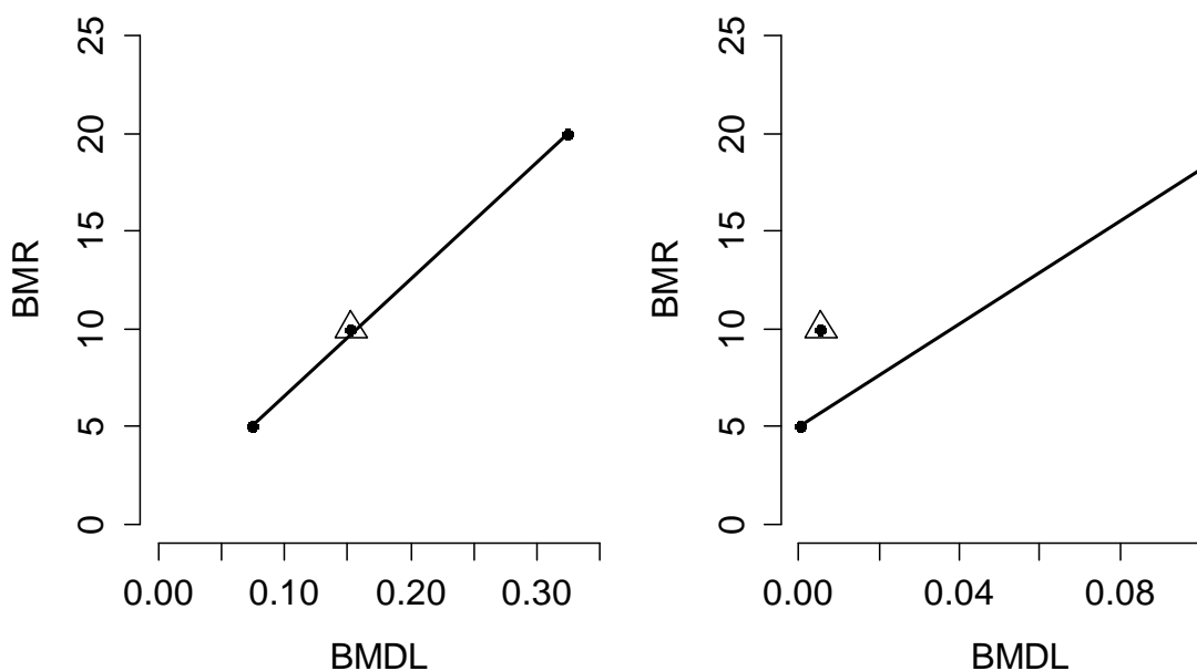
Fig. 2: Comparison of the BMDL computed across different BMRs for a model that is linear (left pane) and supralinear (right pane).
