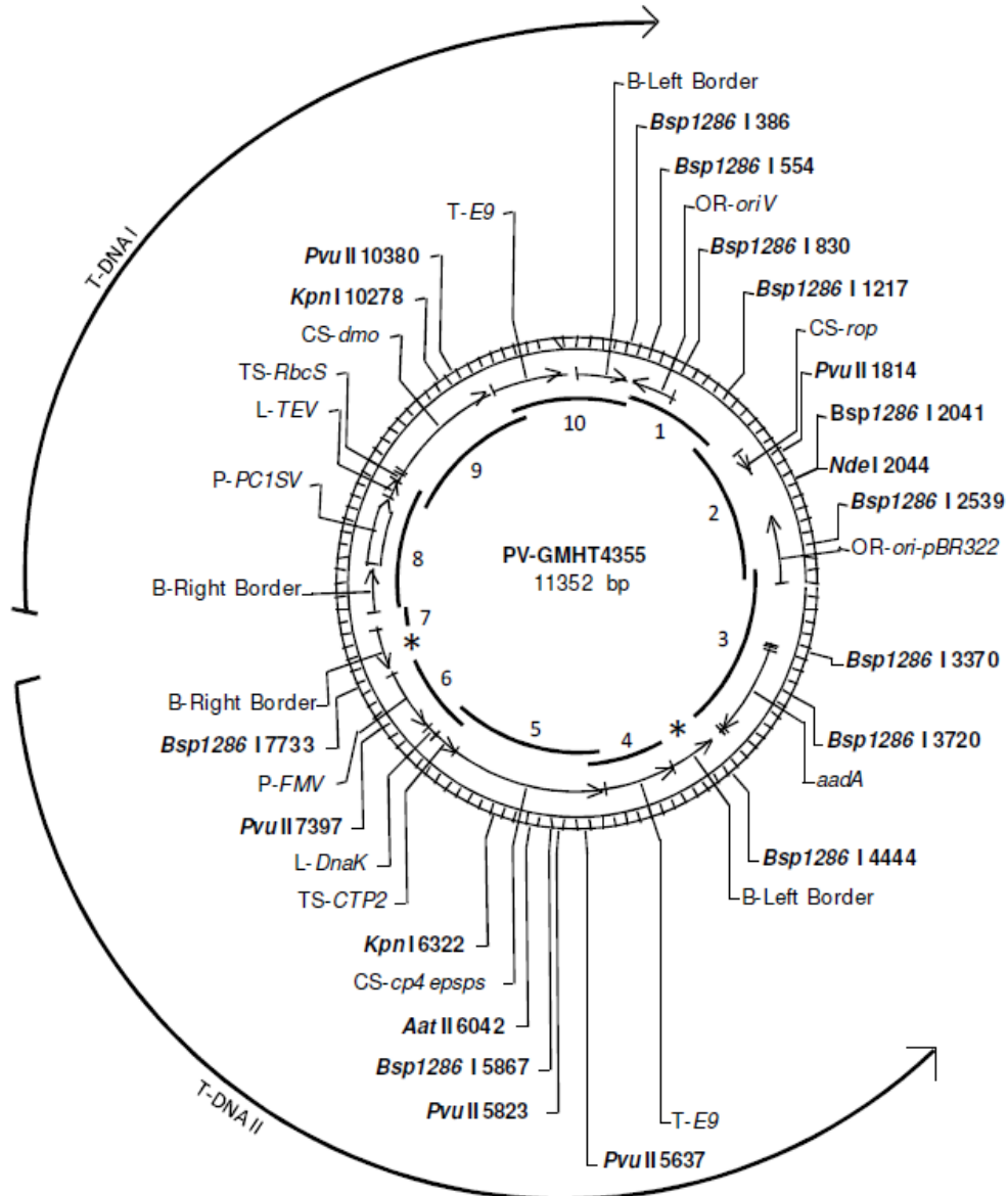
Figure 1: Genes and regulatory elements contained in plasmid PV-GMHT4355
