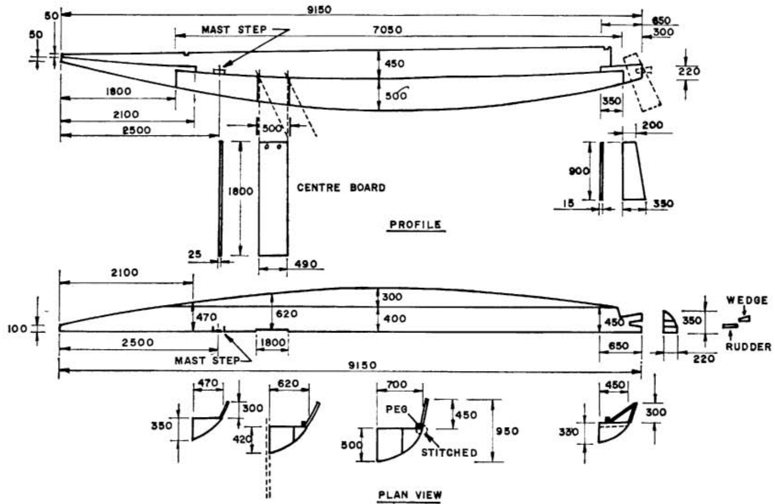
APPENDIX 2C BOAT KATTUMARAM, ANDHRA PRADESH TYPICAL DIMENSIONS OF PRINCIPAL COMPONENTS
