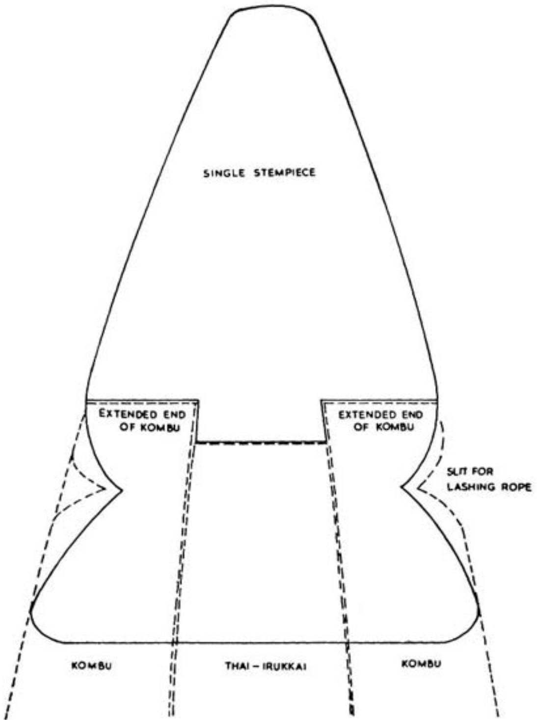
APPENDIX 3D DETAIL OF PROW PIECE FOR A 3-LOG RAFT KATTUMARAM
