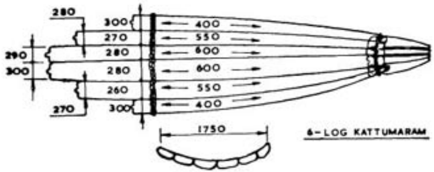
APPENDIX 3C: RAFT KATTUMARAMS-TYPICAL DIMENSIONS AND STRUCTURES
