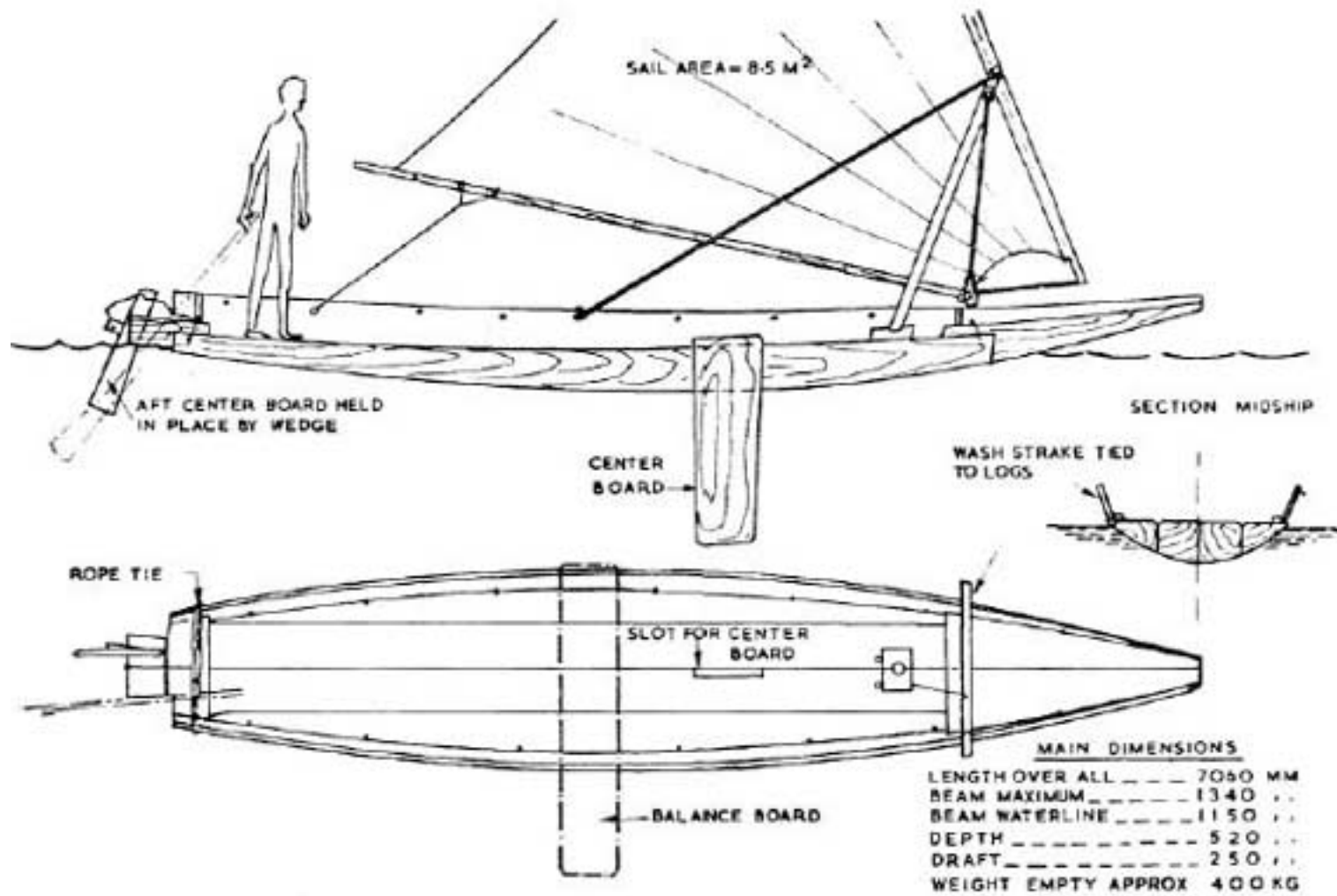
APPENDIX 2A : GENERAL ARRANGEMENT - ANDHRA PRADESH FOUR-LOG BOAT KATTUMARAM
