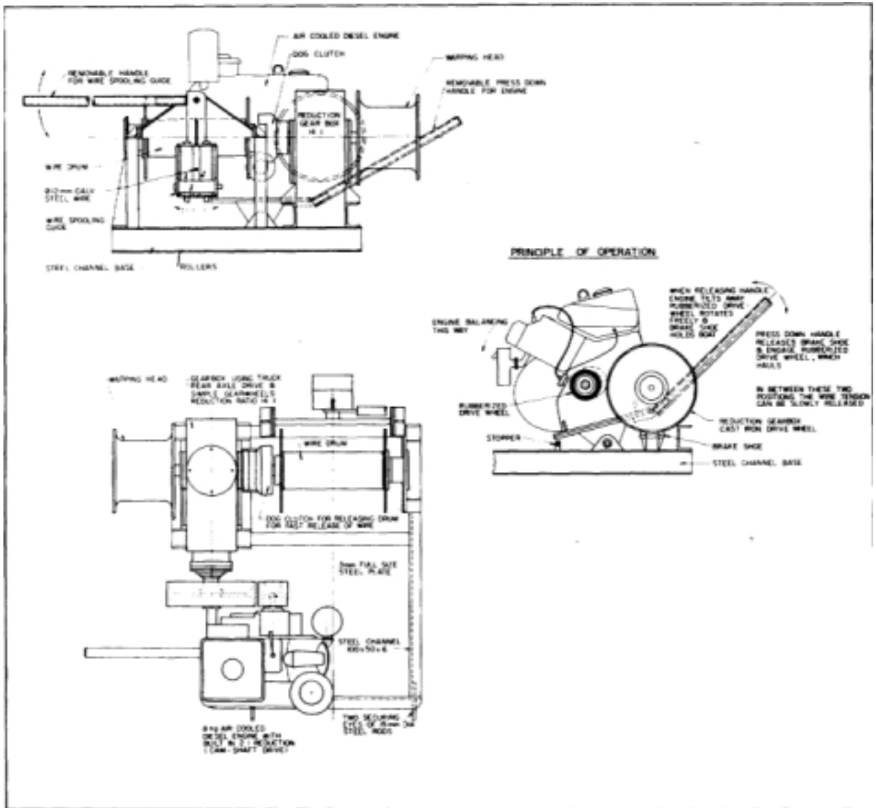
Figure 1 DIESEL ENGINE-DRIVEN WINCH
