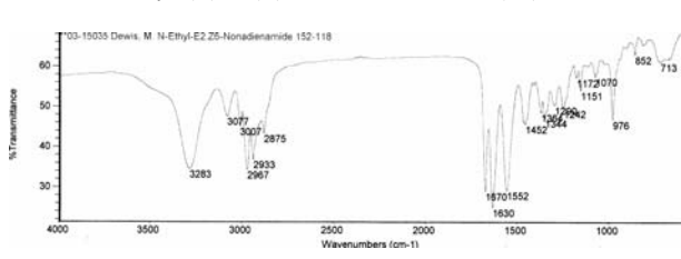
1596 N-Ethyl (E)-2,(Z)-6-nonadienamide (IR)
