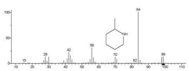
1608 2-Methylpiperidine
