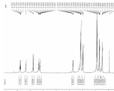
1597 N-Cyclopropyl (E)-2,(Z)-6-nonadienamide (IR)
