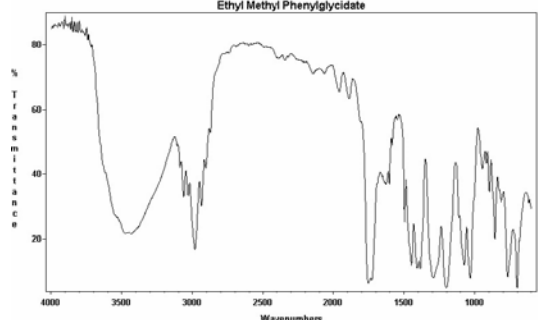
1578 Ethyl methyl-p-tolylglycidate
