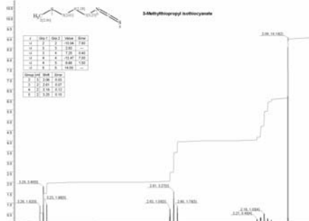
1564 3-Methylthiopropyl isothiocyanate
