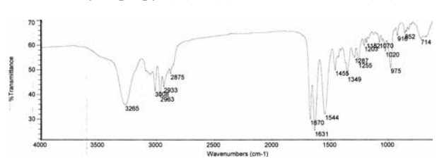
1597 N-Cyclopropyl (E)-2,(Z)-6-nonadienamide (IR)
