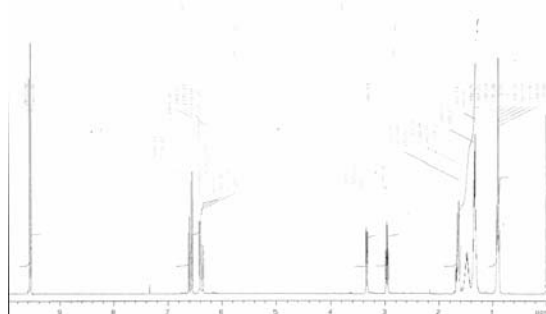
1570 4,5-Epoxy-(E)-2-decenal (NMR)
