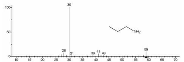
1580 Propylamine
