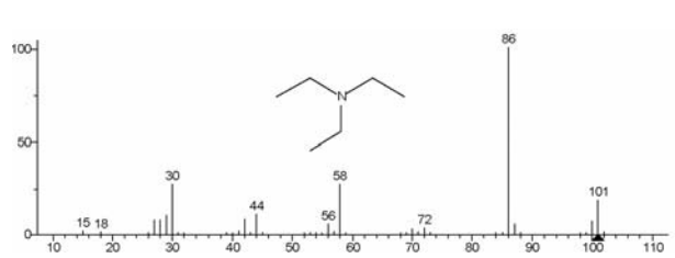
1611 Triethylamine
