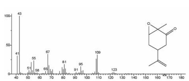
1572 cis-Carvone-5,6-oxide (MS)
