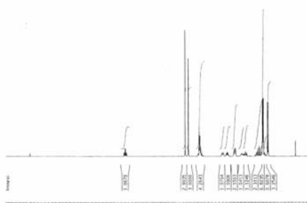
1603 1-Pyrroline
