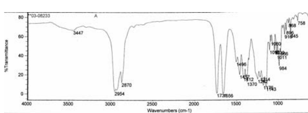
1602 (+/-)-N,N-Dimethyl menthyl succinamide (IR)
