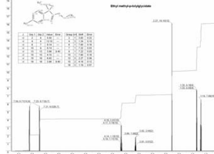
1579 Ethylamine
