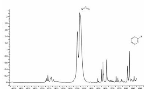
1564 3-Methylthiopropyl isothiocyanate
