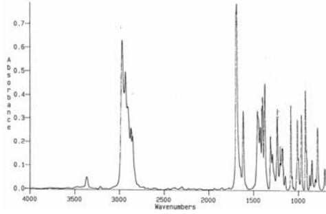
1606 Isopentylidene isopentylamine (IR)
