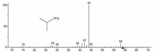
1581 Isopropylamine
