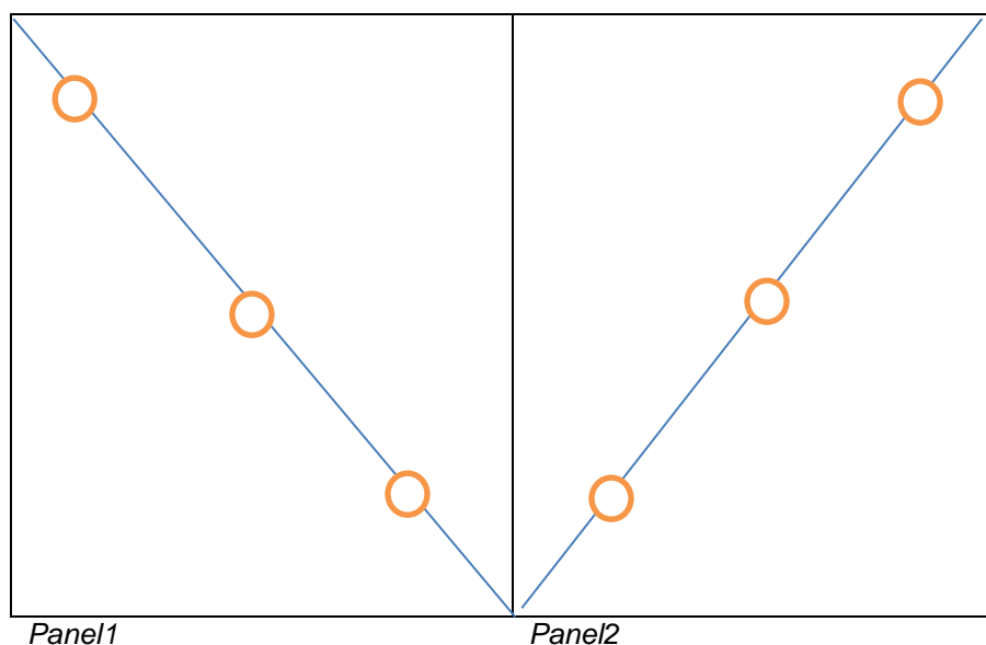
Figure 1 Recommended 6 positions, 3 from each side, cut along the diagonal with at least 10 cm from any edge to make up a representative sample for a product unit.
