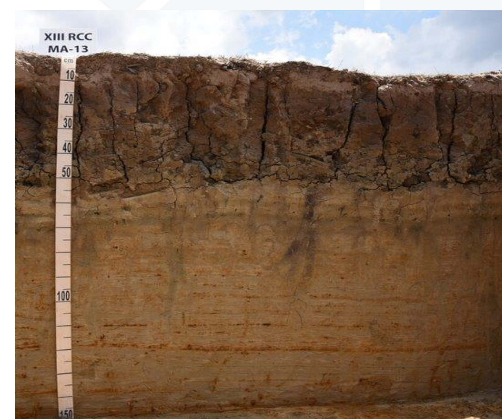
Fig 3. Soil profile of the Katoveritic Pantogleyic Epigeoabruptic Solonetz in Vitória do Mearim, Maranhão, Brazil.
