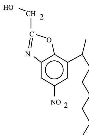
2-(hydroxymethyl)-5-nitro-7-(2-octyl) benzoxazole
