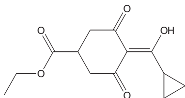
Trinexapac-ethyl
