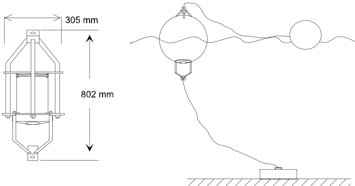
Figure 2.1./3 Buoy based Acoustic Doppler Current Profiler, model "Workhorse" and its installation in the lake.
