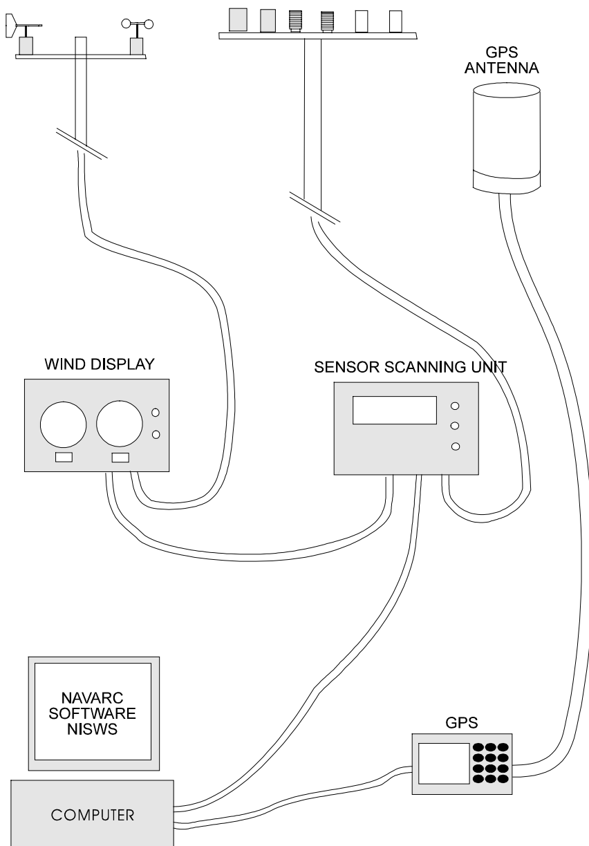
Figure 2.1./4 Installation meteorological station on R/V Tanganyika Explorer.
