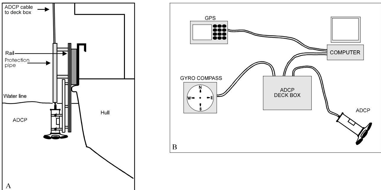
Figure 2.1./2 Acoustic Doppler Current Profiler (ADCP) installation on the side of R/V Tanganyika Explorer (a) and the interfacing of ADCP-Deckbox-Computer-DGPS (b).
