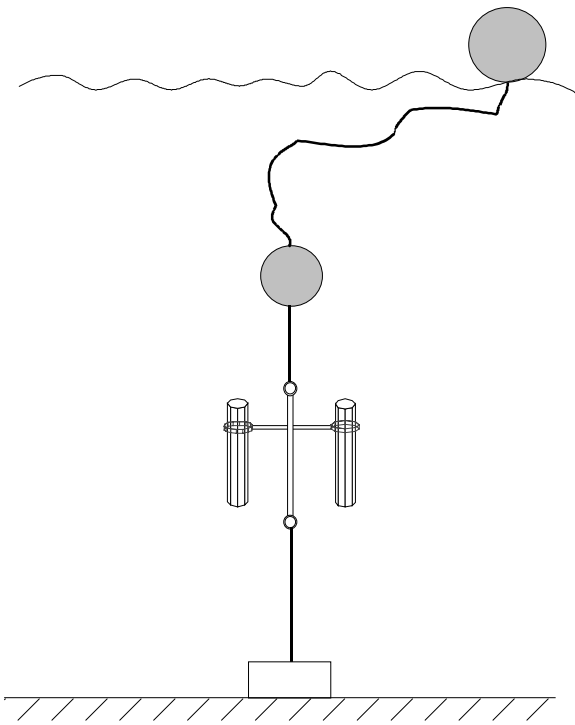
Figure 2.1./5 Sedimentation trap and its installation in the lake.
