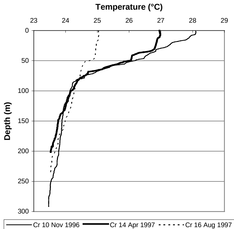
Figure 2.4.4./27 Water temperature profiles in the Mpulungu basin during expeditions 10, 14 and 16 measurements.
