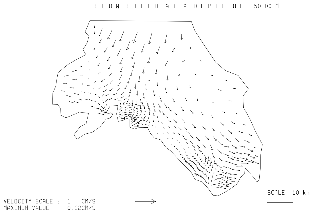
Fig. 3.5.2./62 Calculated flow at a depth of 50 m. Local time 20 h 24.08.97.
