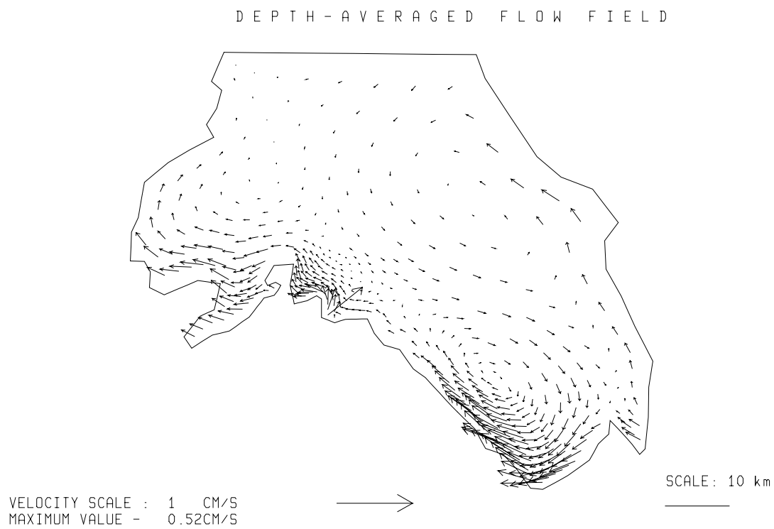
Fig. 3.5.2./65 Calculated depth-averaged flow. Local time 20 h 24.08.97.
