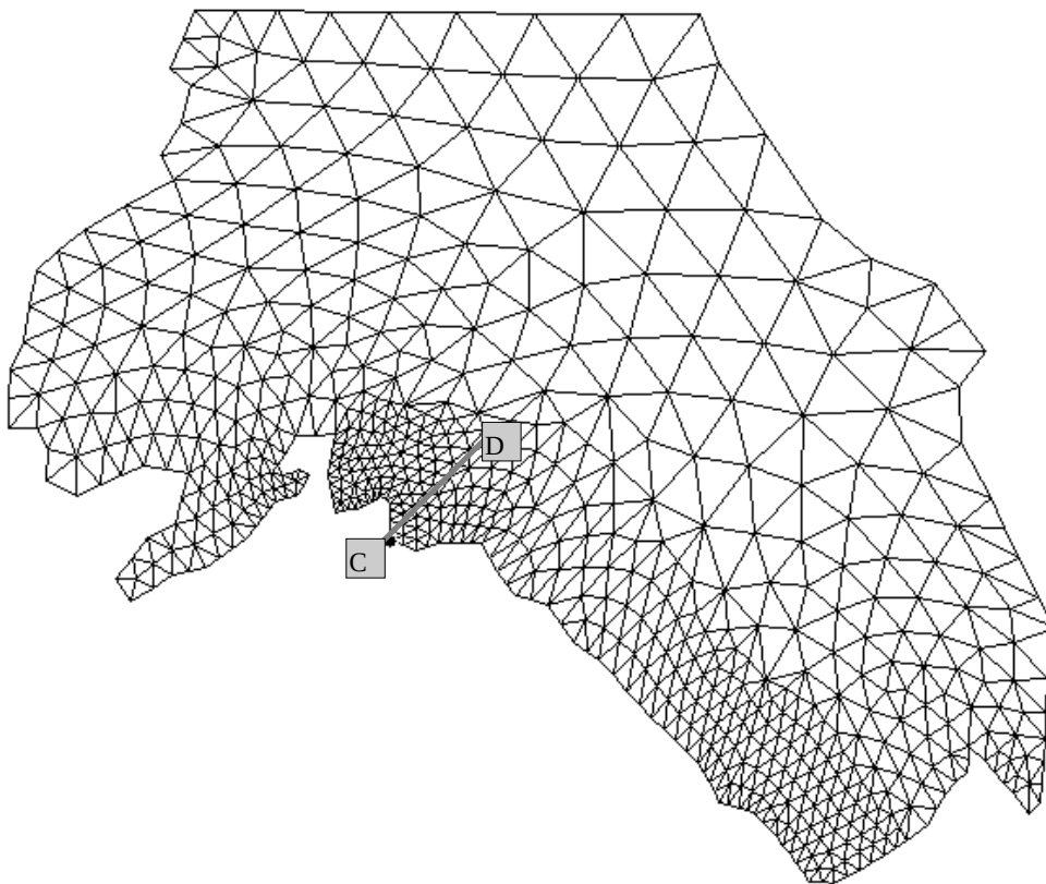
Fig. 3.5.2./4. Triangular grid of the Lufubu regional model.
