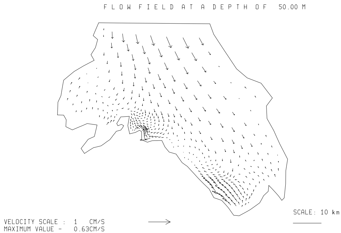
Fig. 3.5.2./47 Calculated flow at a depth of 50 m. Local time 20 h 05.04.97.
