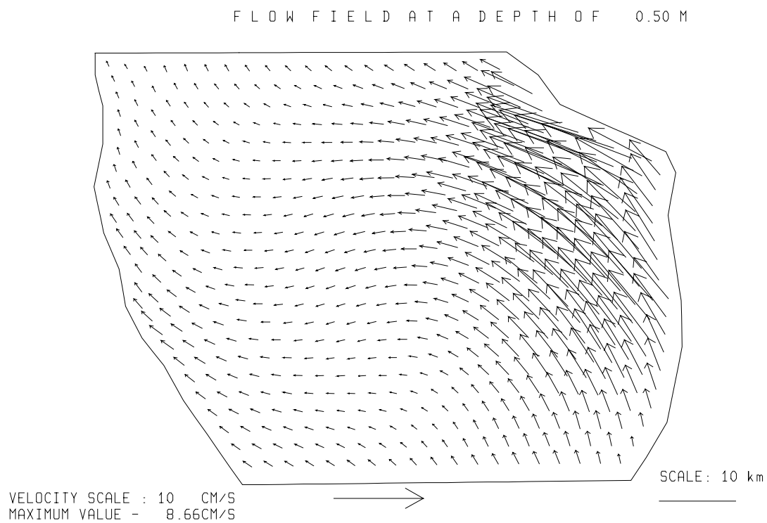
Fig. 3.5.2./26 Calculated flow at a depth of 0.5 m. Local time 12 h 24.08.97.
