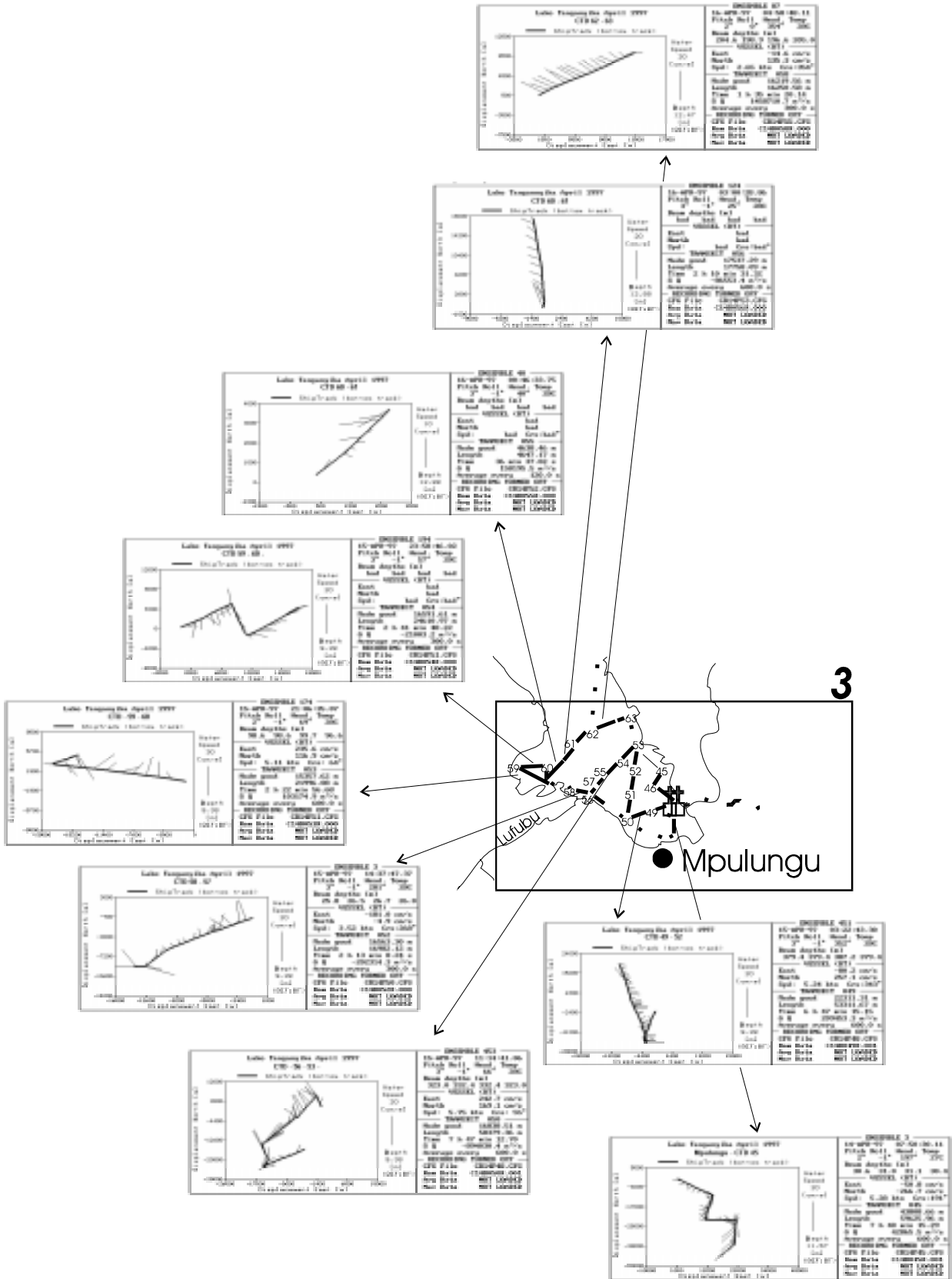
Figure 2.4.4./29 The currents from the uppermost observation layer along transects in the south end of Lake Tanganyika. Expedition 14, April 1997.
