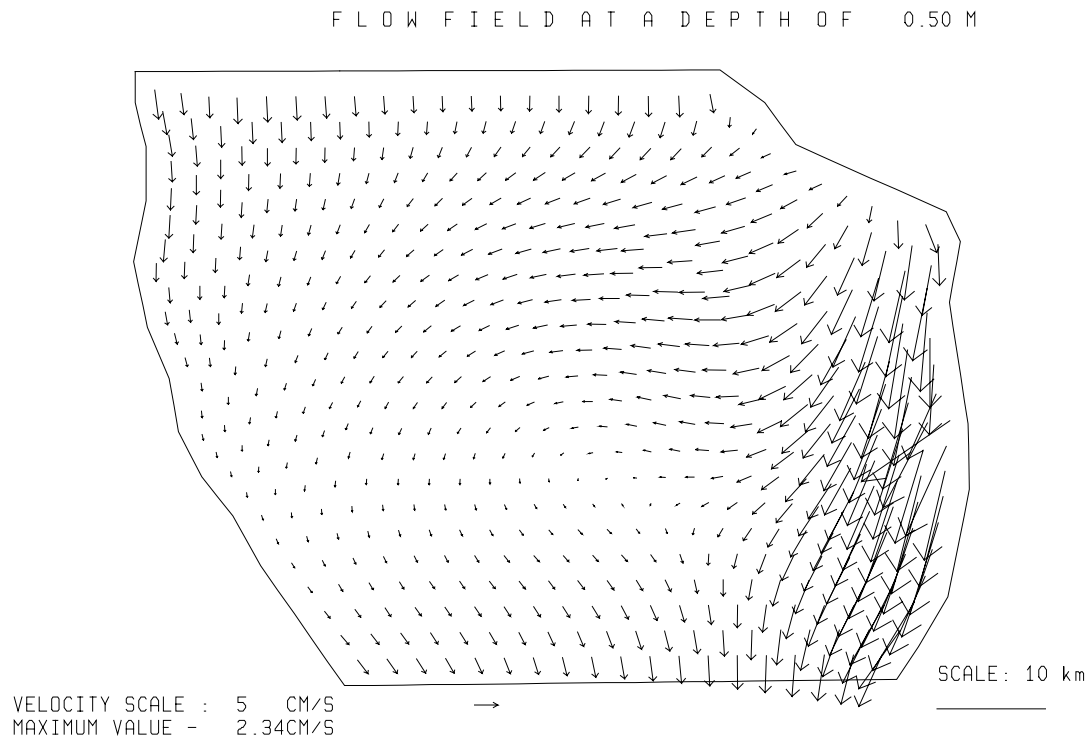
Fig. 3.5.2./16 Calculated flow at a depth of 0.5 m. Local time 20 h 05.04.97.
