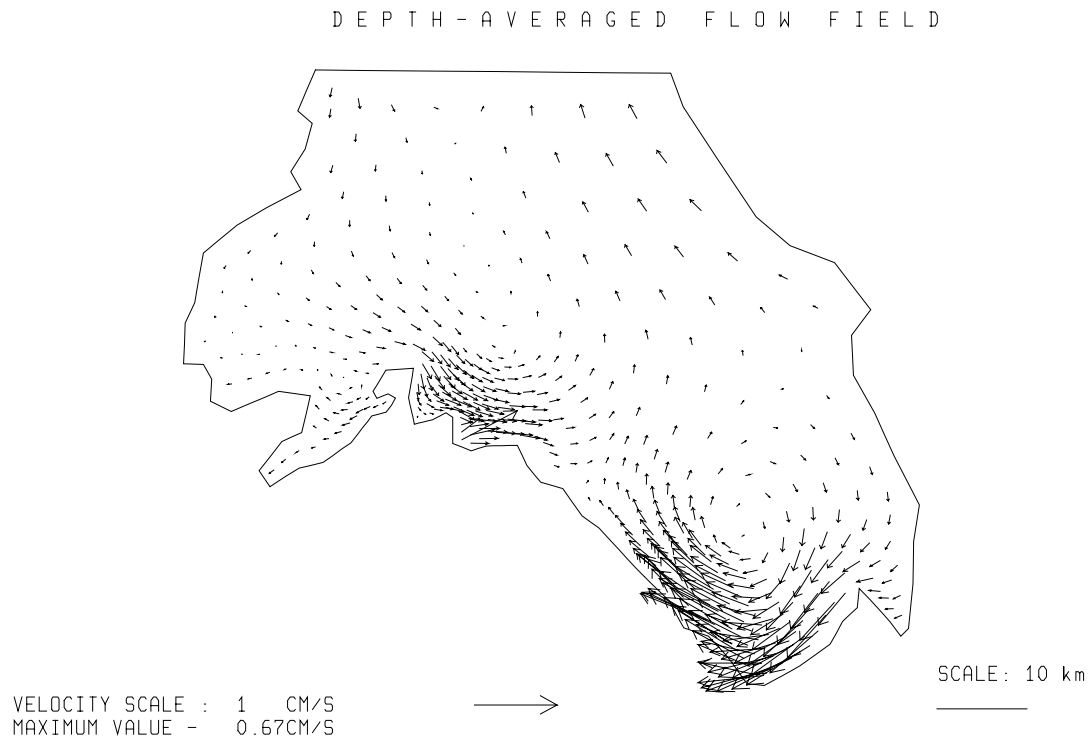
Fig. 3.5.2./60 Calculated depth-averaged flow. Local time 12 h 24.08.97.
