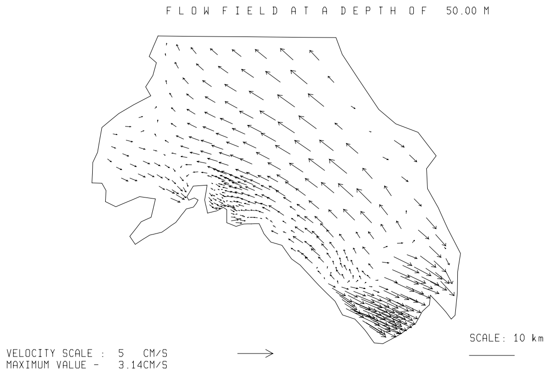
Fig. 3.5.2./52 Calculated flow at a depth of 50 m. Local time 04 h 24.08.97.
