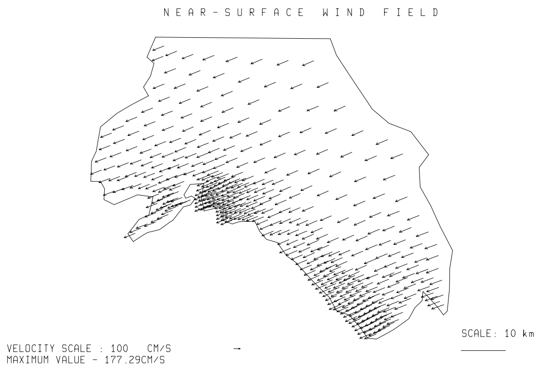
Fig. 3.5.2./59 Simulated near-surface wind. Local time 12 h 24.08.97.
