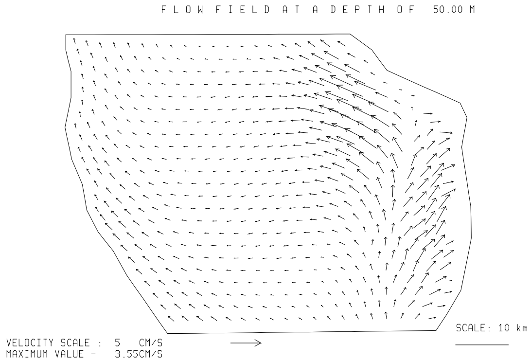
Fig. 3.5.2./22 Calculated flow at a depth of 50 m. Local time 04 h 24.08.97.
