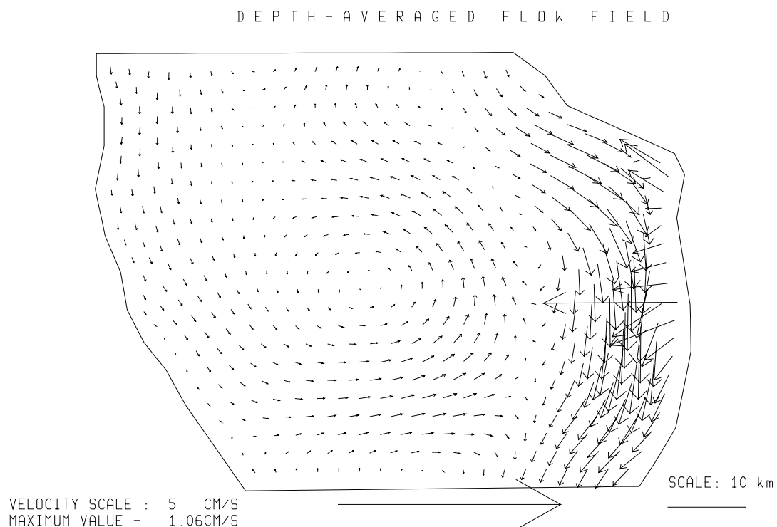
Fig. 3.5.2./35 Calculated depth-averaged flow. Local time 20 h 24.08.97.
