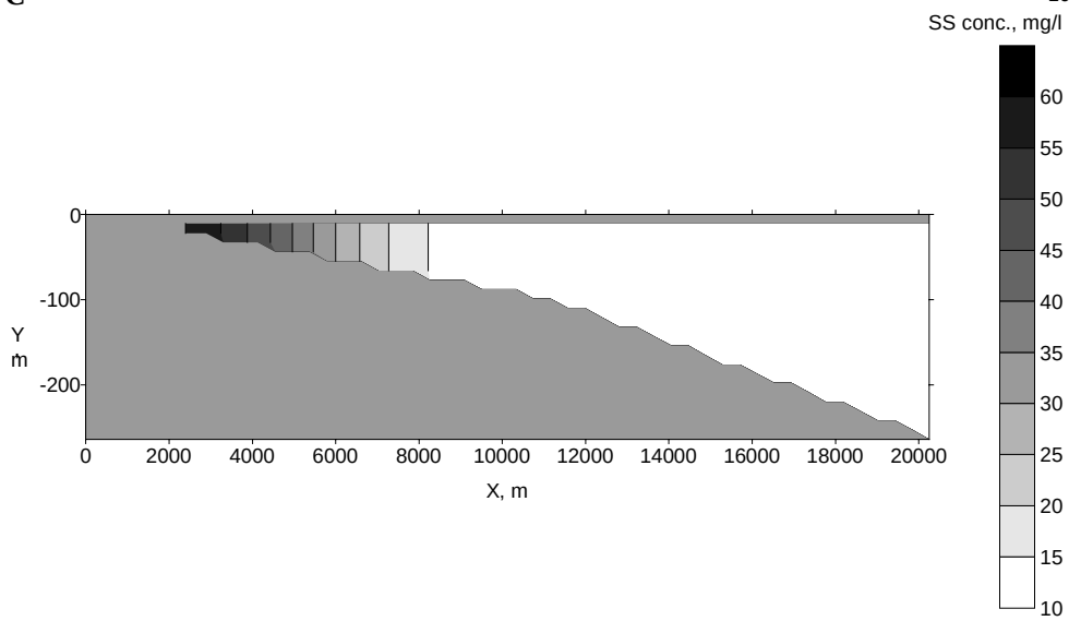
Fig. 3.5.3/6 Calculated SS concentration along a vertical section near river Malagarasi mouth at 0:00 22.08.97 (A), 12:00 24.08.97 (B) and 0:00 28.08.97 (C) after 22, 82 and 166 hours after the simulation start respectively.
