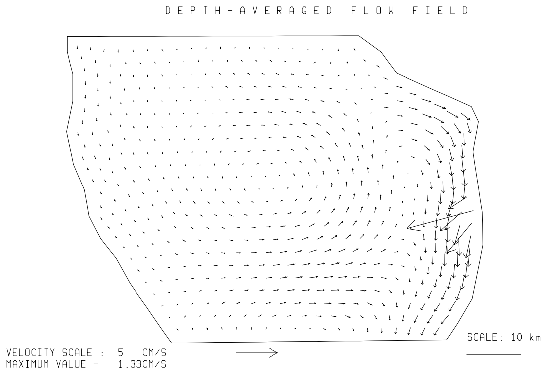
Fig. 3.5.2./20 Calculated depth-averaged flow. Local time 20 h 05.04.97.
