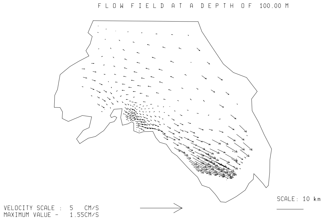
Fig. 3.5.2./38 Calculated flow at a depth of 100 m. Local time 04 h 05.04.97.
