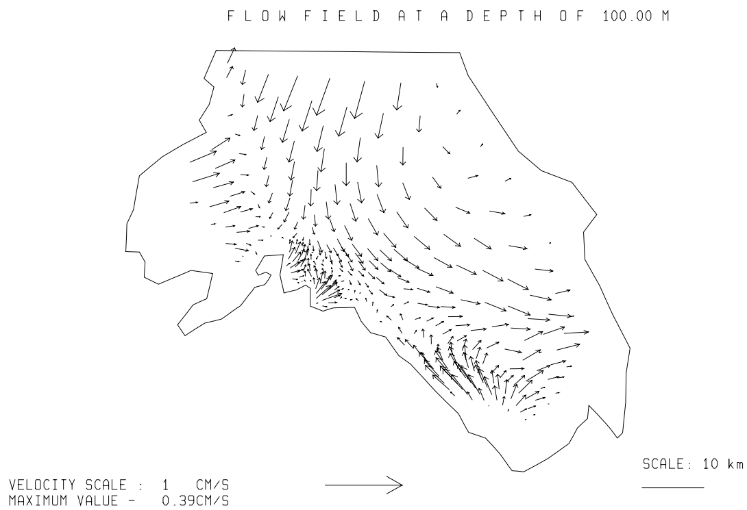
Fig. 3.5.2./63 Calculated flow at a depth of 100 m. Local time 20 h 24.08.97.
