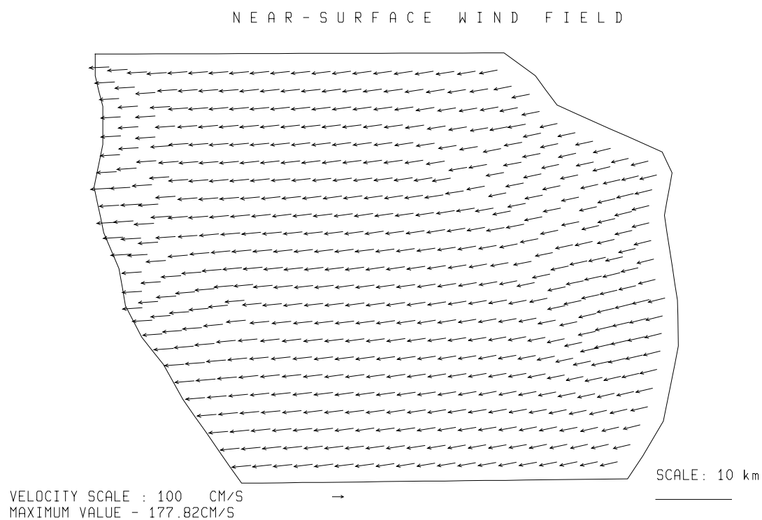
Fig. 3.5.2./29 Simulated near-surface wind. Local time 12 h 24.08.97.
