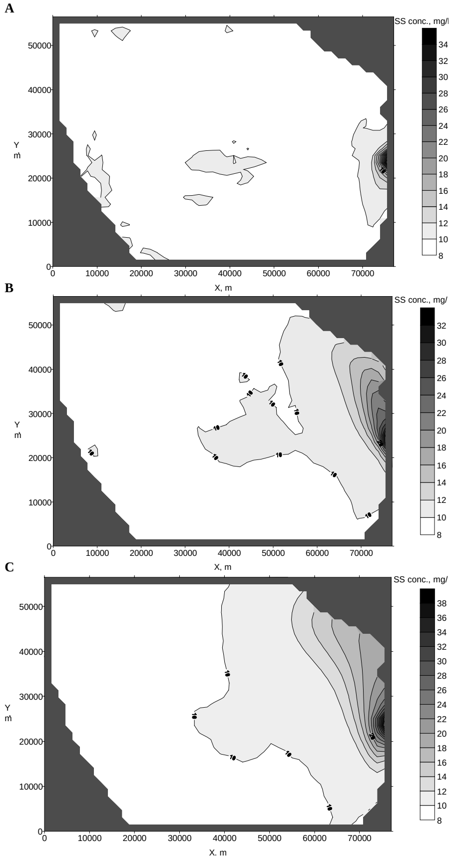
Fig. 3.5.3./2 Calculated SS concentration in the surface layer at 0:00 22.08.97 (A), 12:00 24.08.97 (B) and 0:00 28.08.97 (C) after 22, 82 and 166 hours after the simulation start respectively
