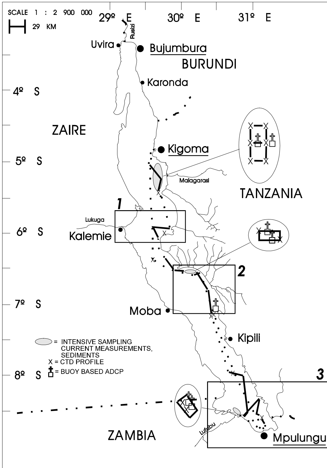
Figure 2.2/1 Schematic map of the transects and CTD profiles measured during the expedition 10 (15. - 27.11.96) on R/V TANGANYIKA EXPLORER. Data from the areas surrounded with boxes are discussed in results.
