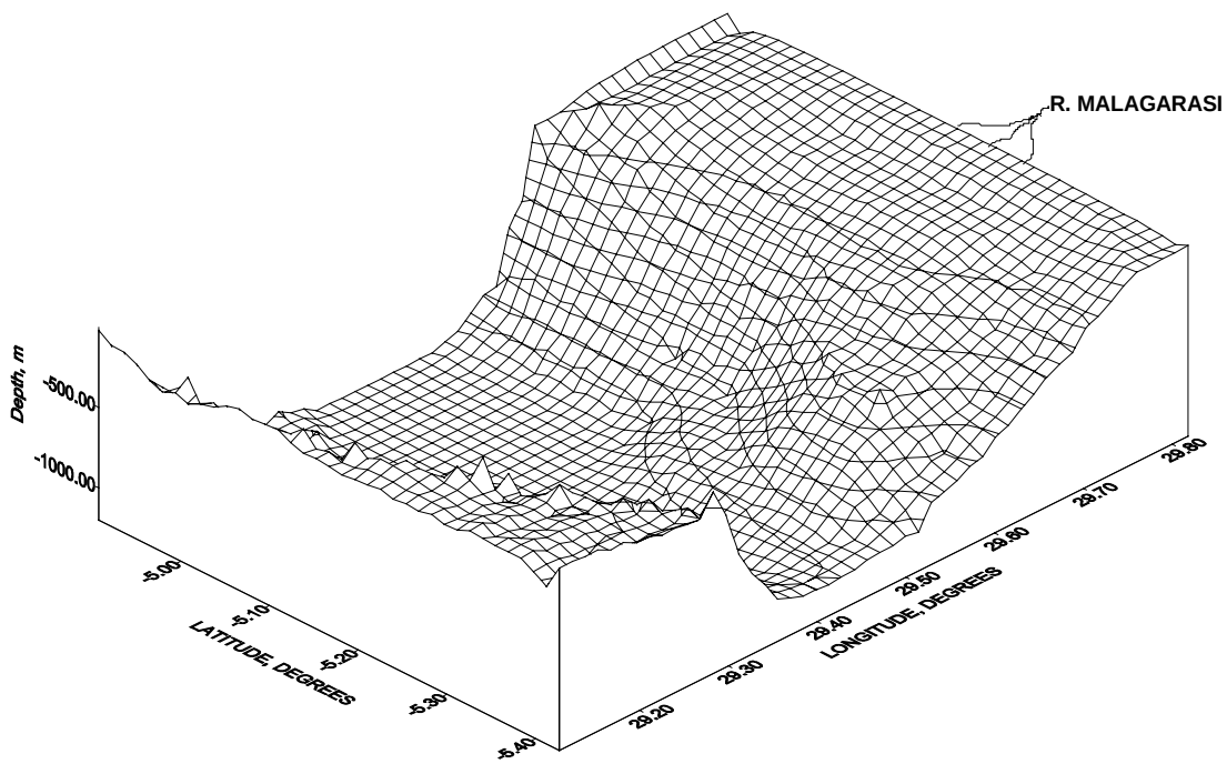
Fig.3.5.2./1 Lake Tanganyika bathymetry near River Malagarasi mouth.
