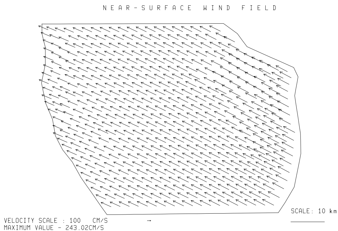
Fig. 3.5.2./9 Simulated near-surface wind. Local time 04 h 05.04.97.
