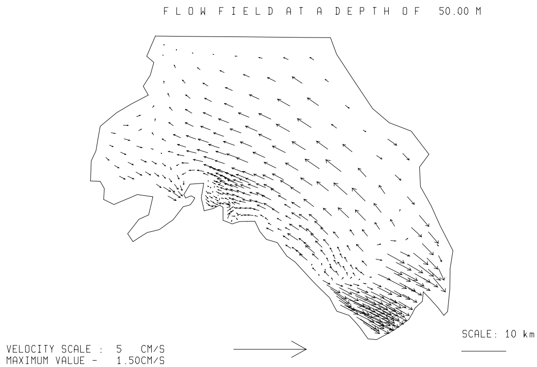
Fig. 3.5.2./37 Calculated flow at a depth of 50 m. Local time 04 h 05.04.97.
