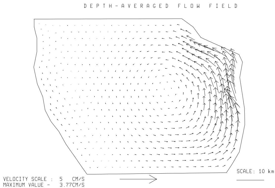
Fig. 3.5.2./10 Calculated depth-averaged flow. Local time 04 h 05.04.97.
