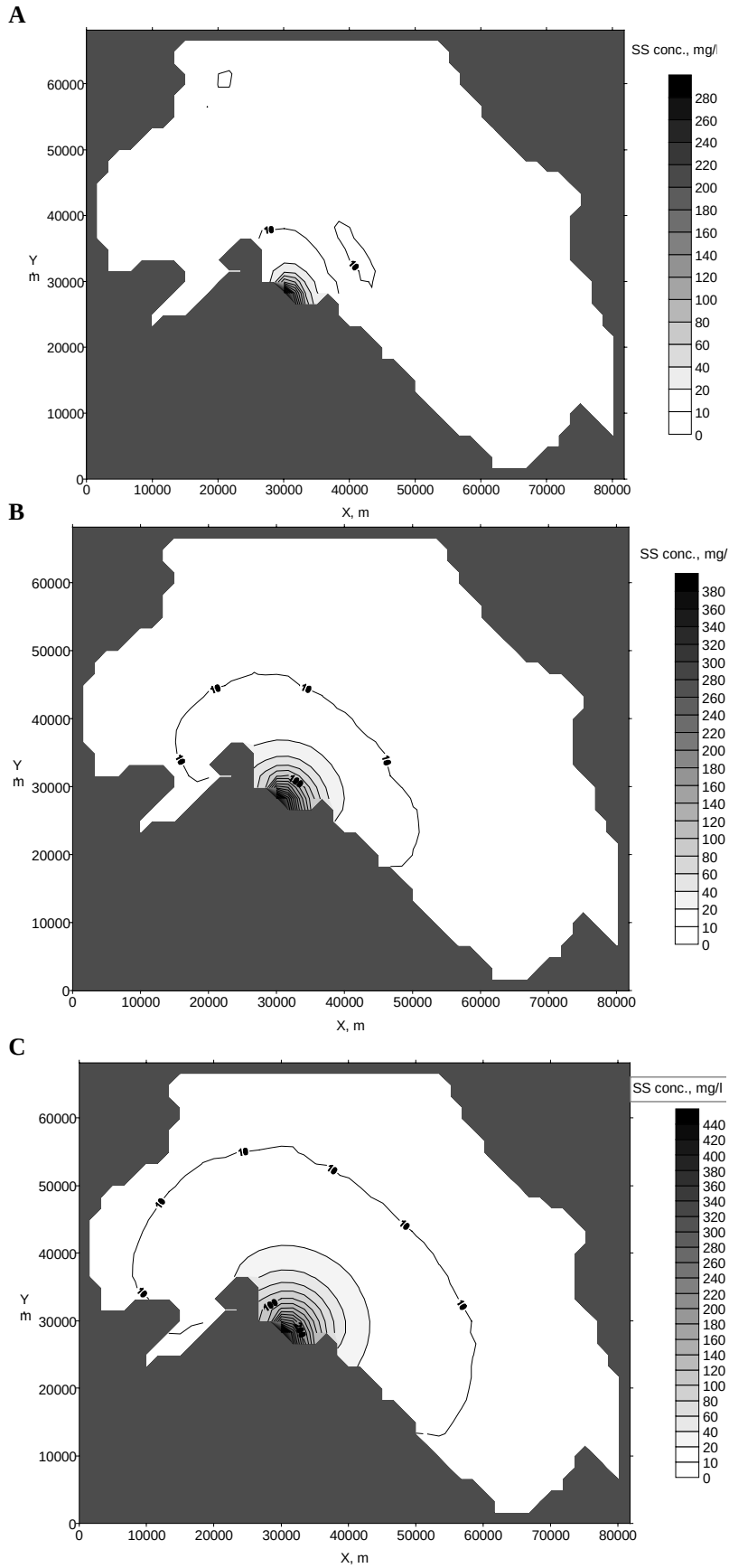
Fig. 3.5.3./3 Calculated SS concentration in the surface layer at 0:00 3.04.97 (A), 12:00 5.04.97 (B) and 0:00 9.04.97 (C) after 22, 82 and 166 hours after the simulation start respectively.
