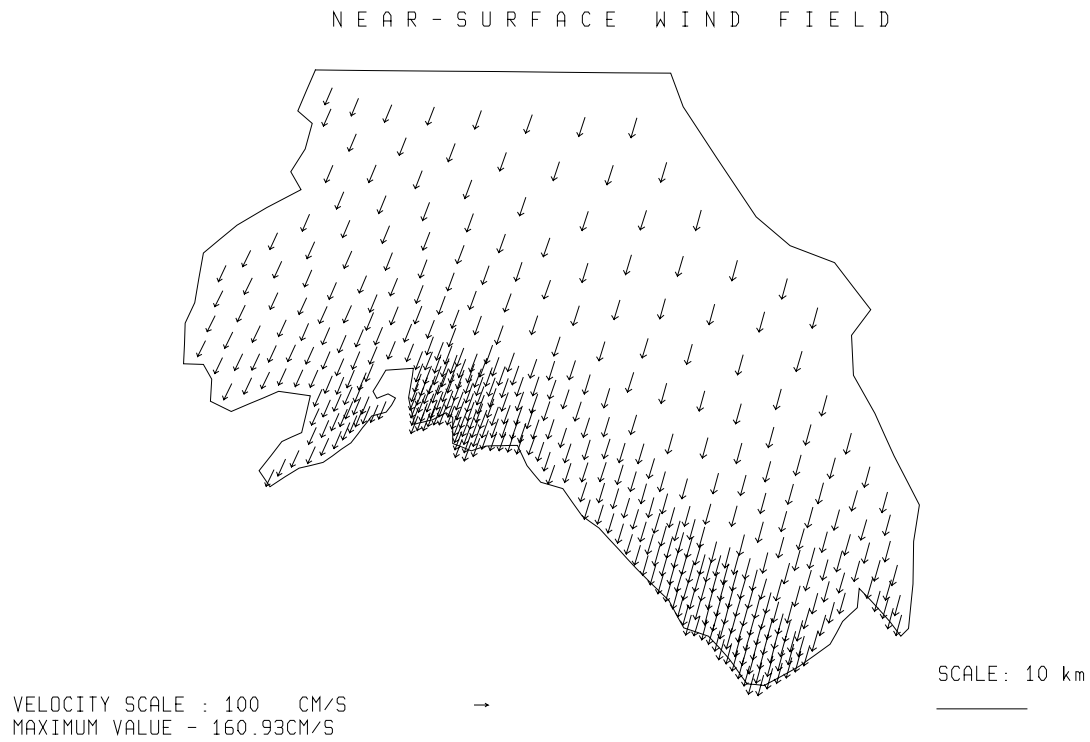
Fig. 3.5.2./44 Simulated near-surface wind. Local time 12 h 05.04.97.
