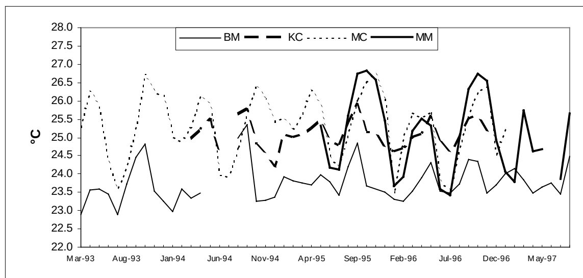
Figure 2.4.1./2 Monthly mean air temperature at Bujumbura (BM) and Mpulungu (MM), and offshore near Kigoma (KC) and Mpulungu (MC).
