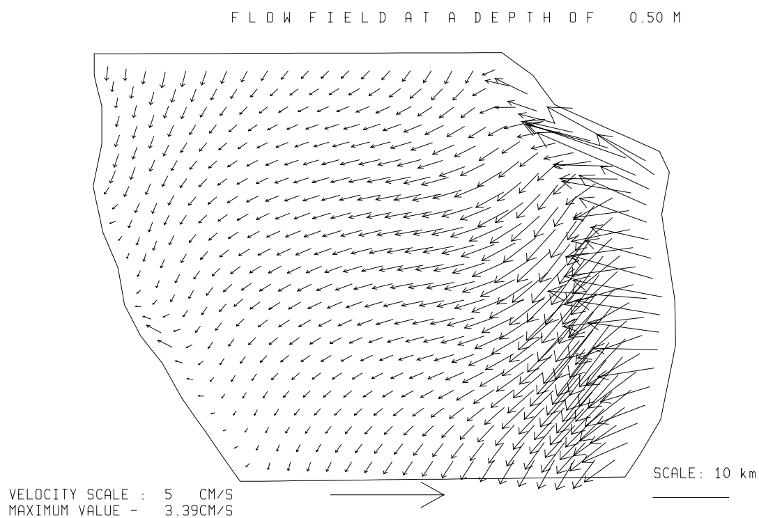
Fig. 3.5.2./31 Calculated flow at a depth of 0.5 m. Local time 20 h 24.08.97.
