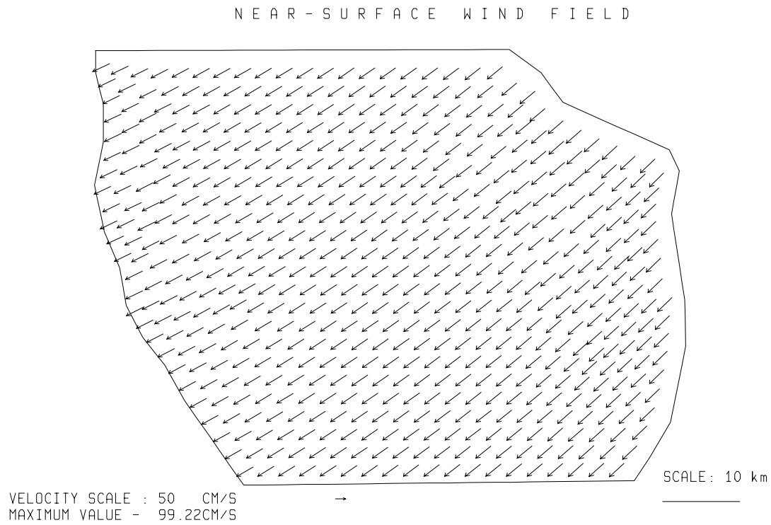
Fig. 3.5.2./14 Simulated near-surface wind. Local time 12 h 05.04.97.
