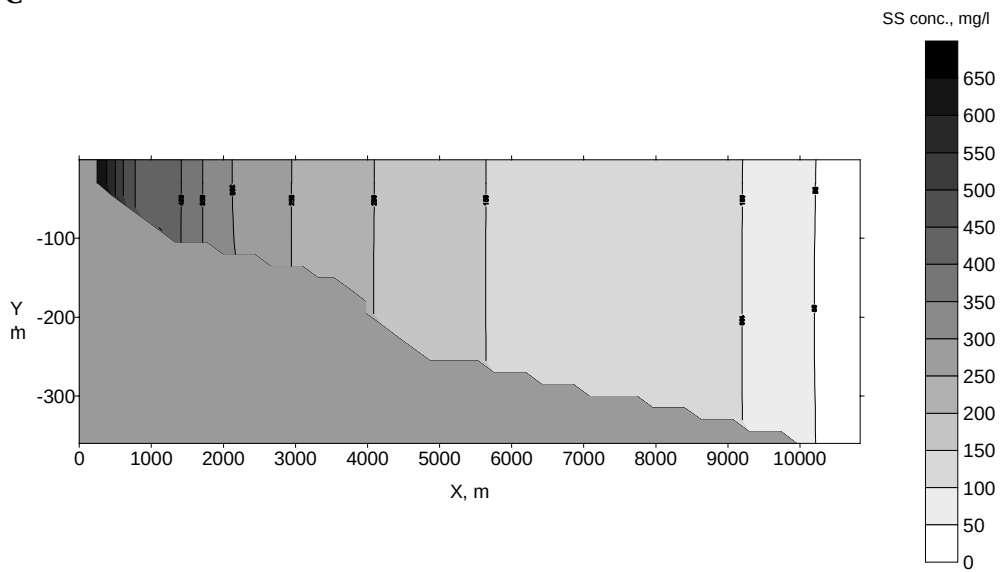
Fig. 3.5.3./7 Calculated SS concentration along a vertical section near river Lufubu mouth at 0:00 3.04.97 (A), 12:00 5.04.97 (B) and 0:00 9.04.97 (C) after 22, 82 and 166 hours after the simulation start respectively.
