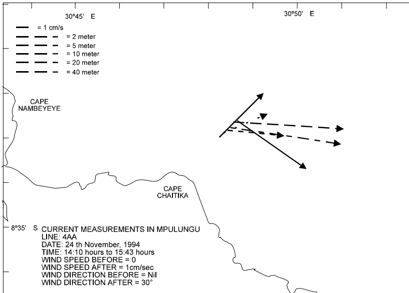
Figure 2.5./3 Water currents measured by flow cylinders (depth 2 m and 5 m) in the Mpulungu basin near Cape Chaitiga on Nov 24, 1994. The legend shows wind data before and after current measurements.
