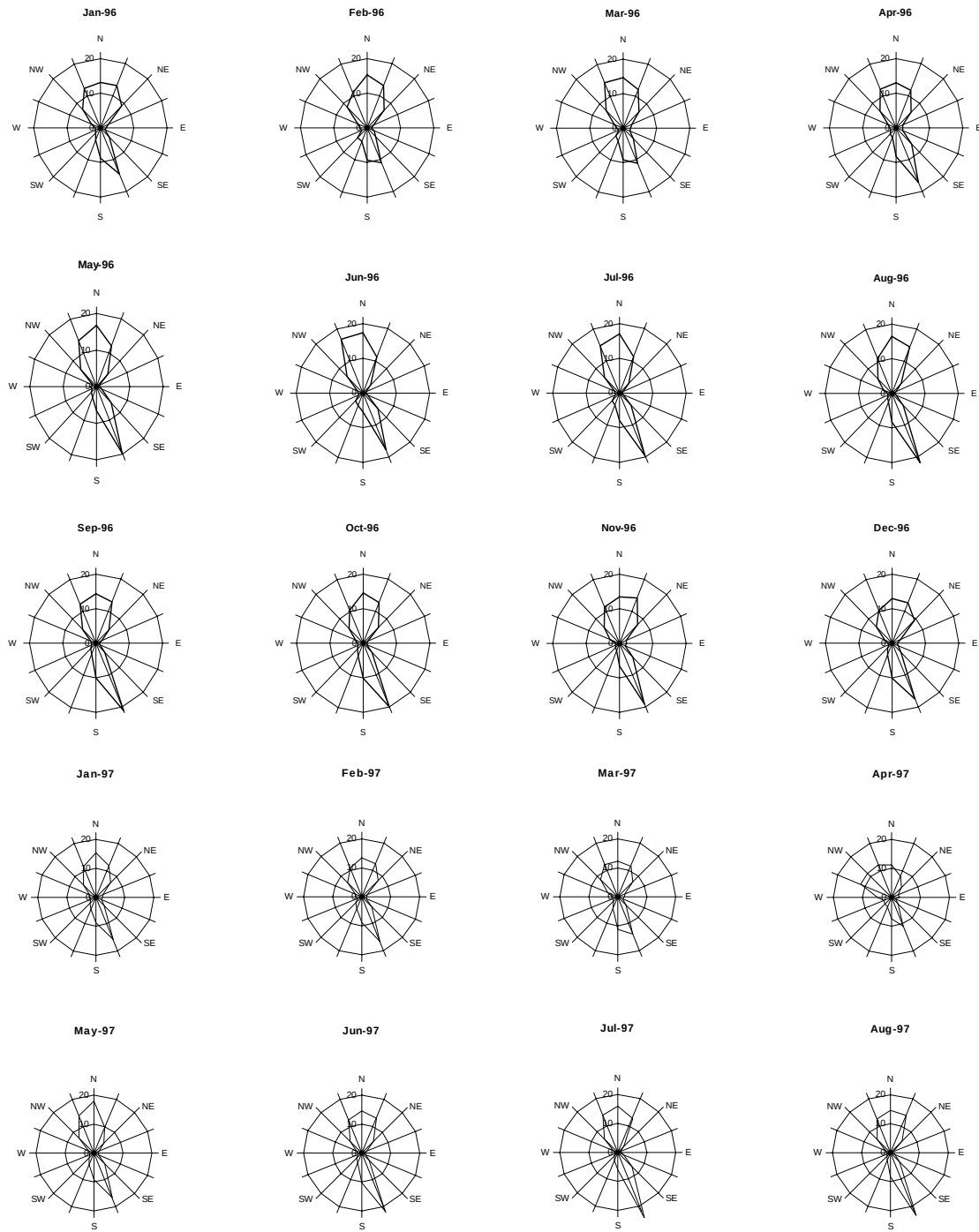
Figure 2.4.1/5 Wind direction distributions (%) on a monthly basis, at Bujumbura weather station.
