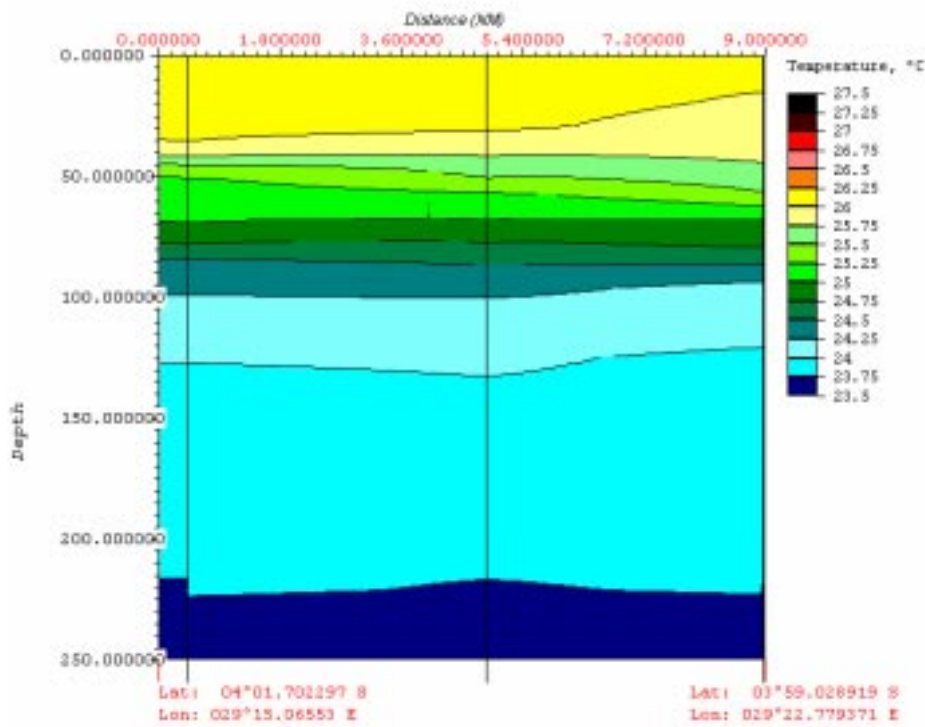
Figure 2.4.2./10. August 1997, temperature transect near Rumonge along transversal axis.
