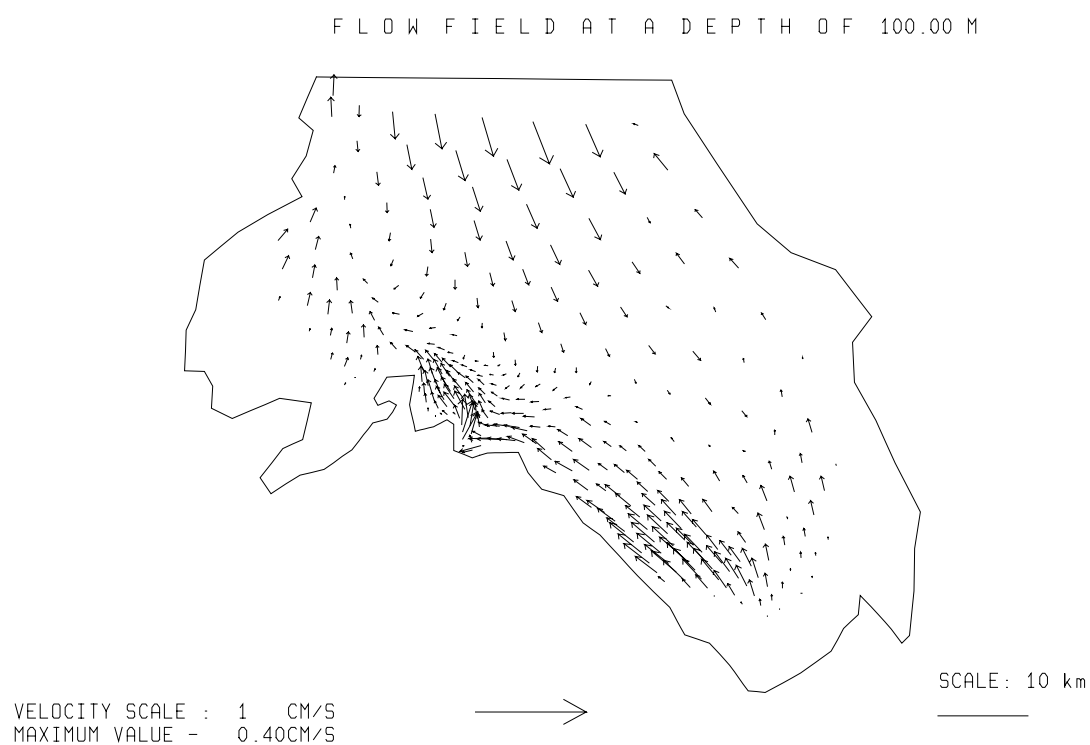
Fig. 3.5.2./48 Calculated flow at a depth of 100 m. Local time 20 h .
