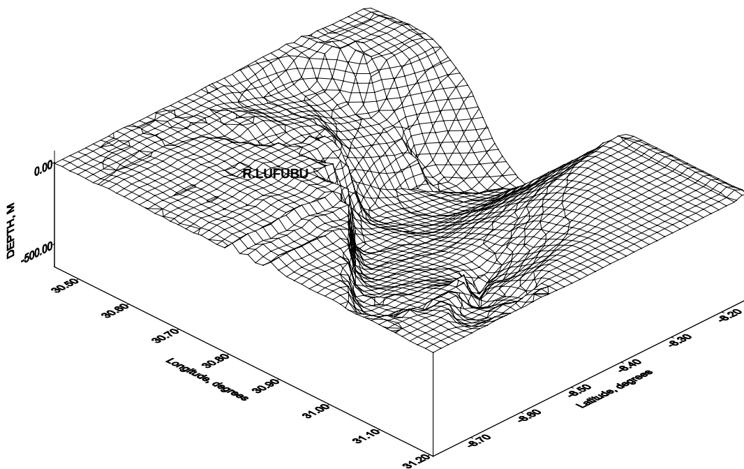
Fig.3.5.2./2 Lake Tanganyika bathymetry in the south part.
