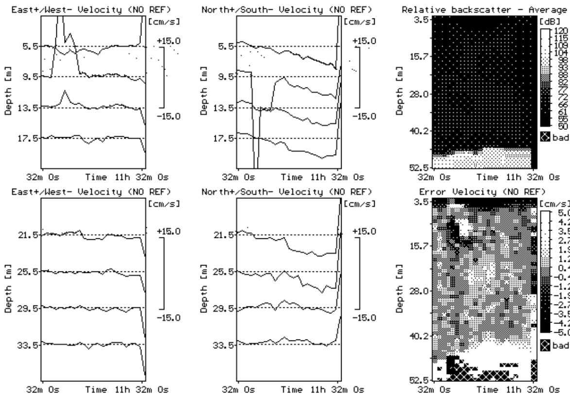
Figure 2.4.4./33 Time series of currents near the Kalambo River mouth in April 1997. Measurement period was 14.4. 06:00 - 17:15. Water depth at the observation site was 39 m.
