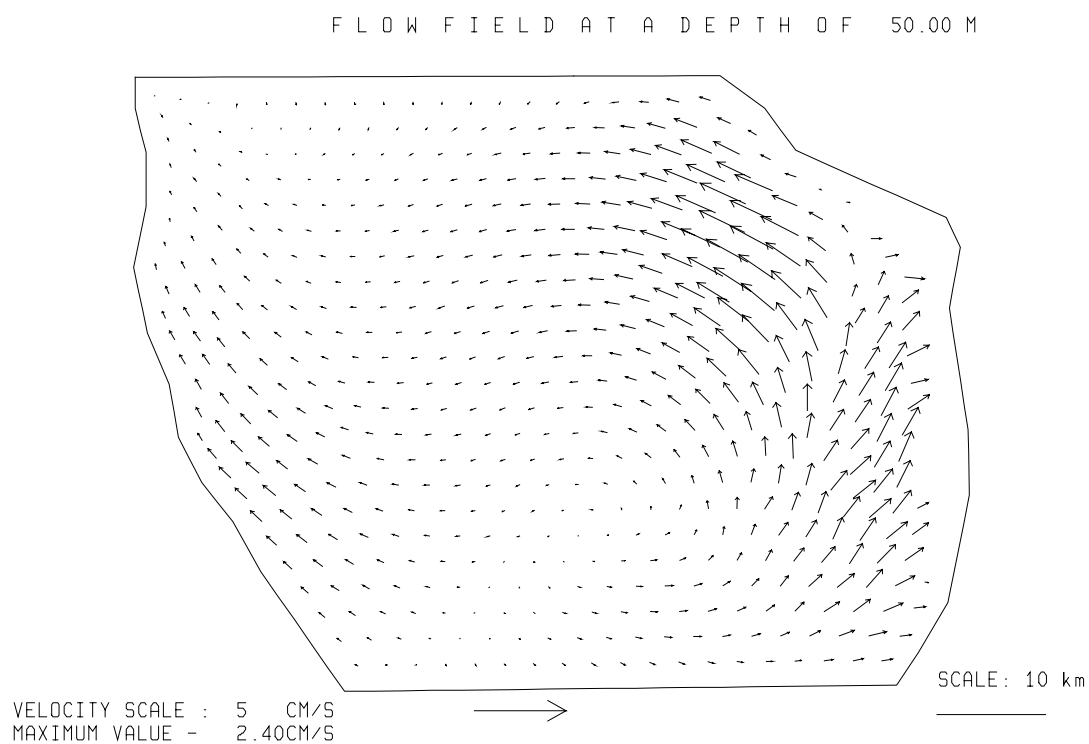
Fig. 3.5.2./7 Calculated flow at a depth of 50 m. Local time 04 h 05.04.97.
