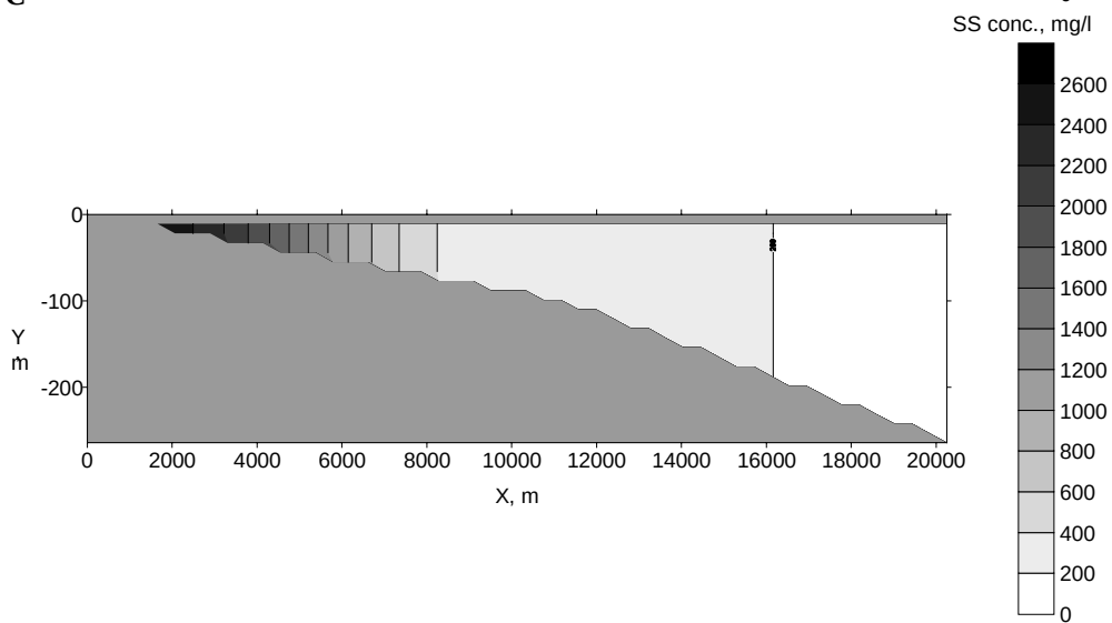
Fig. 3.5.3./5 Calculated SS concentration along a vertical section near river Malagarasi mouth at 0:00 3.04.97 (A), 12:00 5.04.97 (B) and 0:00 9.04.97 (C) after 22, 82 and 166 hours after the simulation start respectively.
