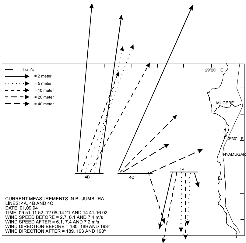
Figure 2.5./5 Water currents measured by flow cylinders (depth 2 - 40 m) near Bujumbura on Sep 01, 1994. The legend shows wind data before and after current measurements on each line.
