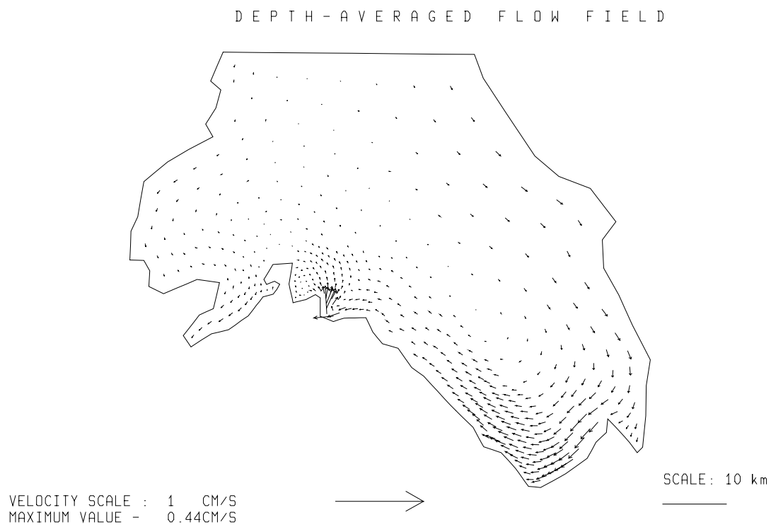
Fig. 3.5.2./45 Calculated depth-averaged flow. Local time 12 h 05.04.97.
