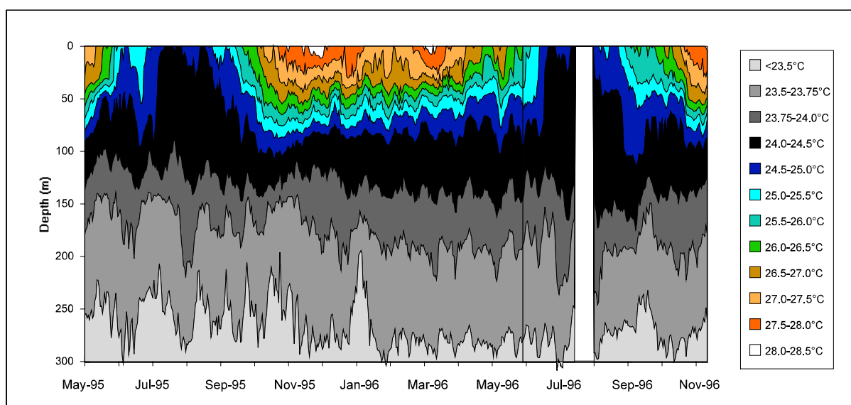
Figure 2.4.1./13 Water temperature isolines (°C) based on daily means. Period from May 1995 to November 1996 at the Mpulungu buoy.
