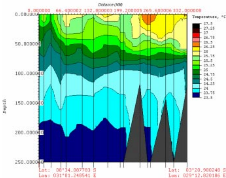
Figure 2.4.2./6. August 1997, temperature isolines along the main axis of the lake.
