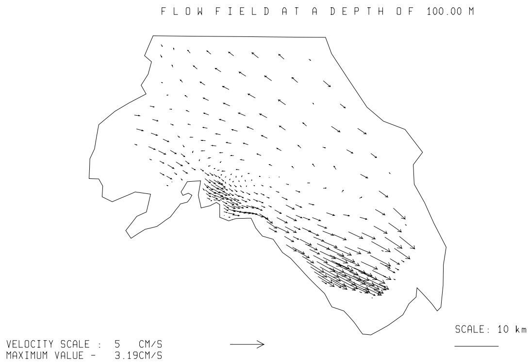
Fig. 3.5.2./53 Calculated flow at a depth of 100 m. Local time 04 h 24.08.97.
