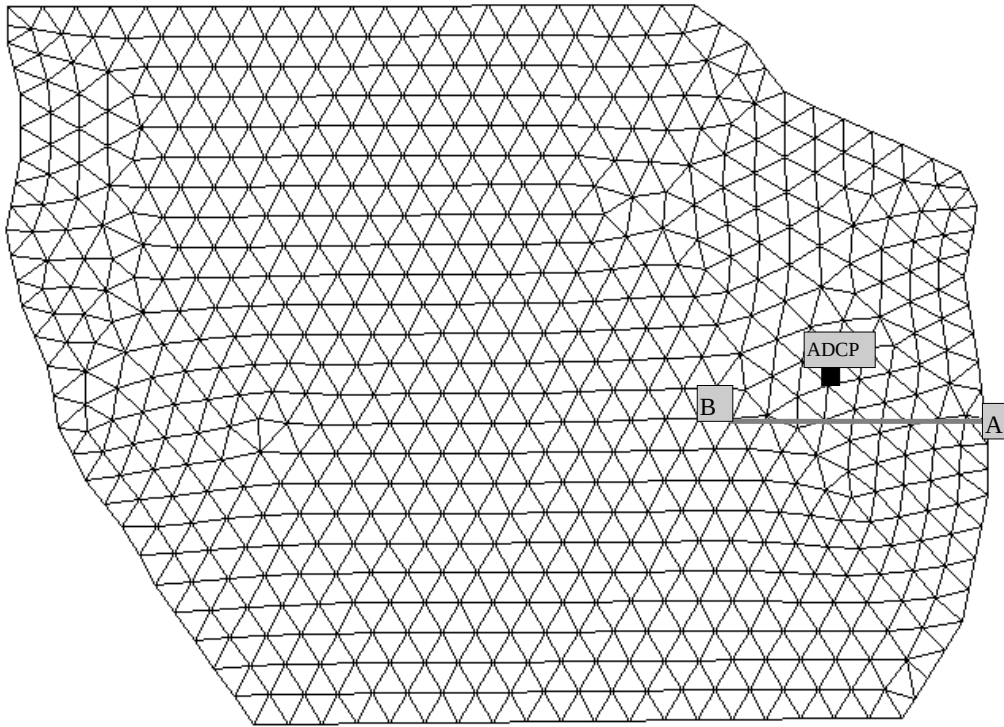
Fig. 3.5.2./3. Triangular grid of the Malagarasi regional model. Black box marks the location of the moored ADCP installed during the last expedition in August, 1997.
