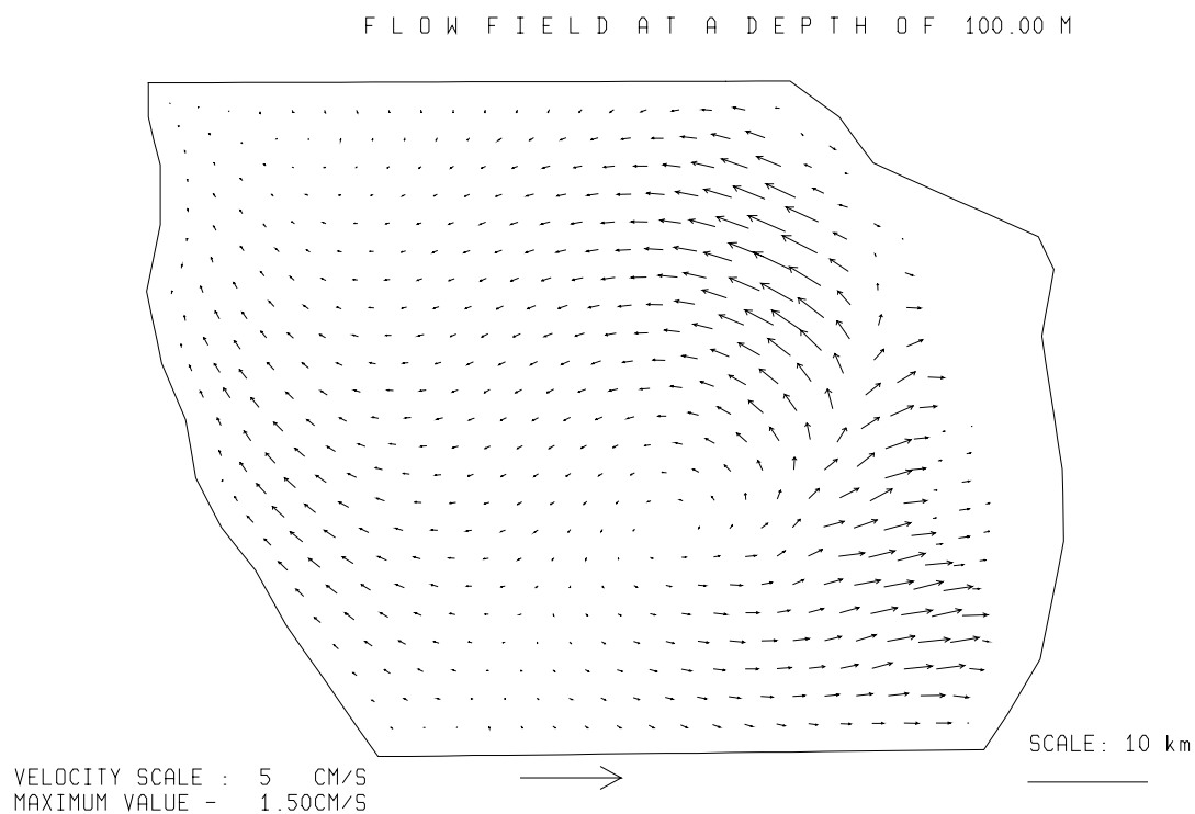
Fig. 3.5.2./8 Calculated flow at a depth of 100 m. Local time 04 h 05.04.97.
