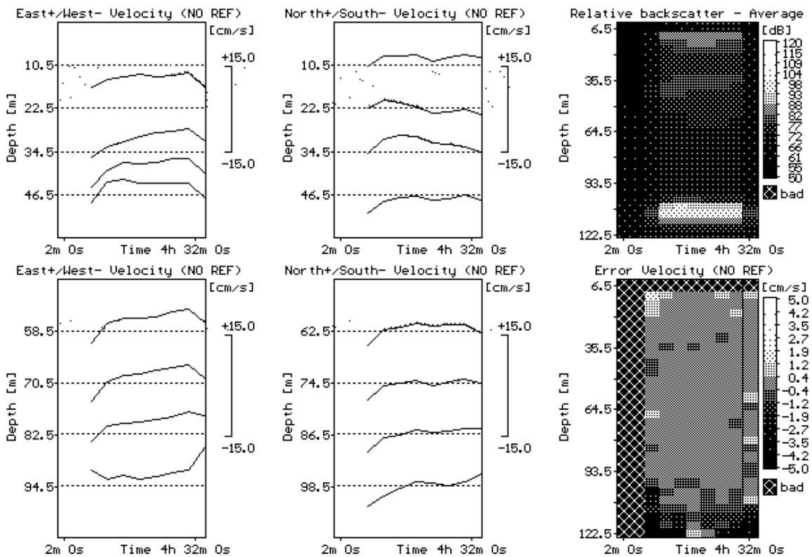
Figure 2.4.4./23 Time series of currents near Kibwesa in November 1996. Measurement period was 22.11. 14:28 - 22.11. 18:02. Water depth at the observation site was 128 m.
