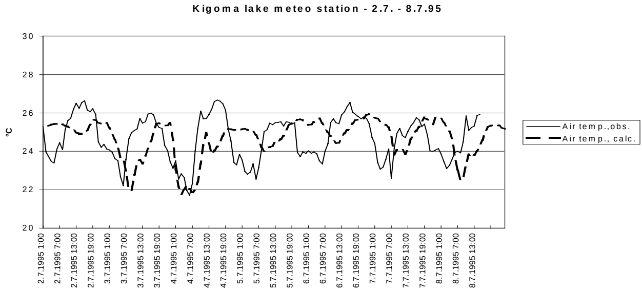
Fig.3.5.1./2. Comparison of one hour mean observed and calculated air temperature at Kigoma lake meteo station.
