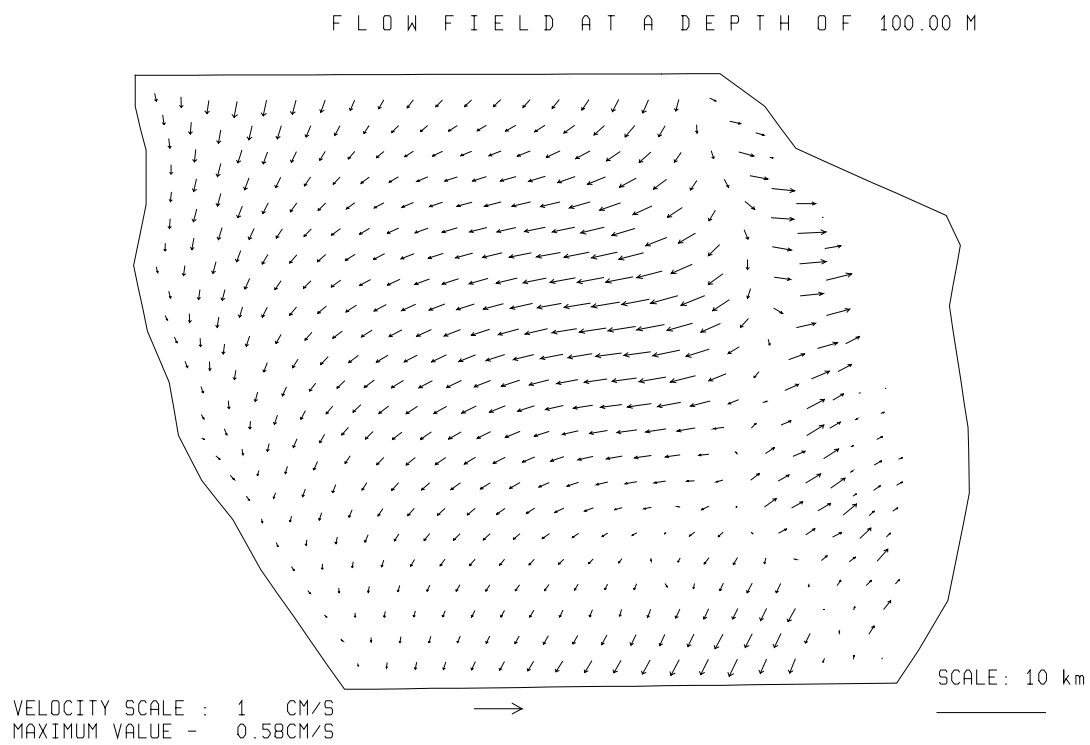
Fig. 3.5.2./33 Calculated flow at a depth of 100 m. Local time 20 h 24.08.97.
