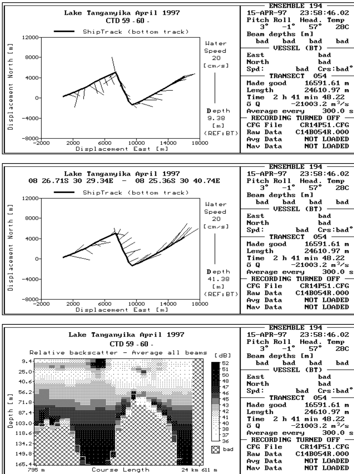
Figure 2.4.4./31 Water currents and echo intensity (lower panel) along the transect in Sumbu bay during April 1997 measurements.
