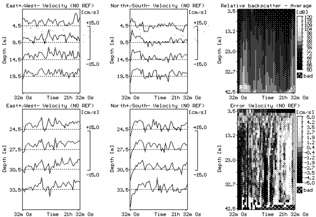
Figure 2.4.4./3 Time series of currents near Ruzisi during August 1997 Measurement period was 21.8. 14:43 - 22.8. 12:26. Water depth at the observation site was 46 m.
