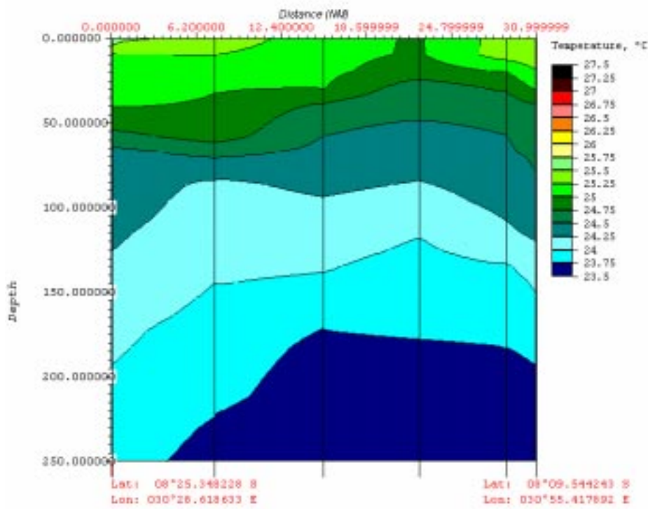
Figure 2.4.2./7. August 1997, temperature transect in the south basin in west - east direction.
