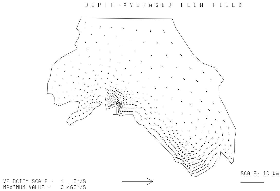
Fig. 3.5.2./50 Calculated depth-averaged flow. Local time 20 h 05.04.97.
