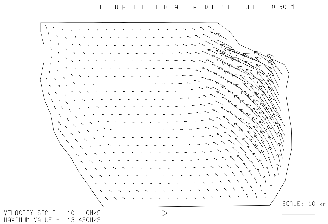
Fig. 3.5.2./21 Calculated flow at a depth of 0.5 m. Local time 04 h 24.08.97.
