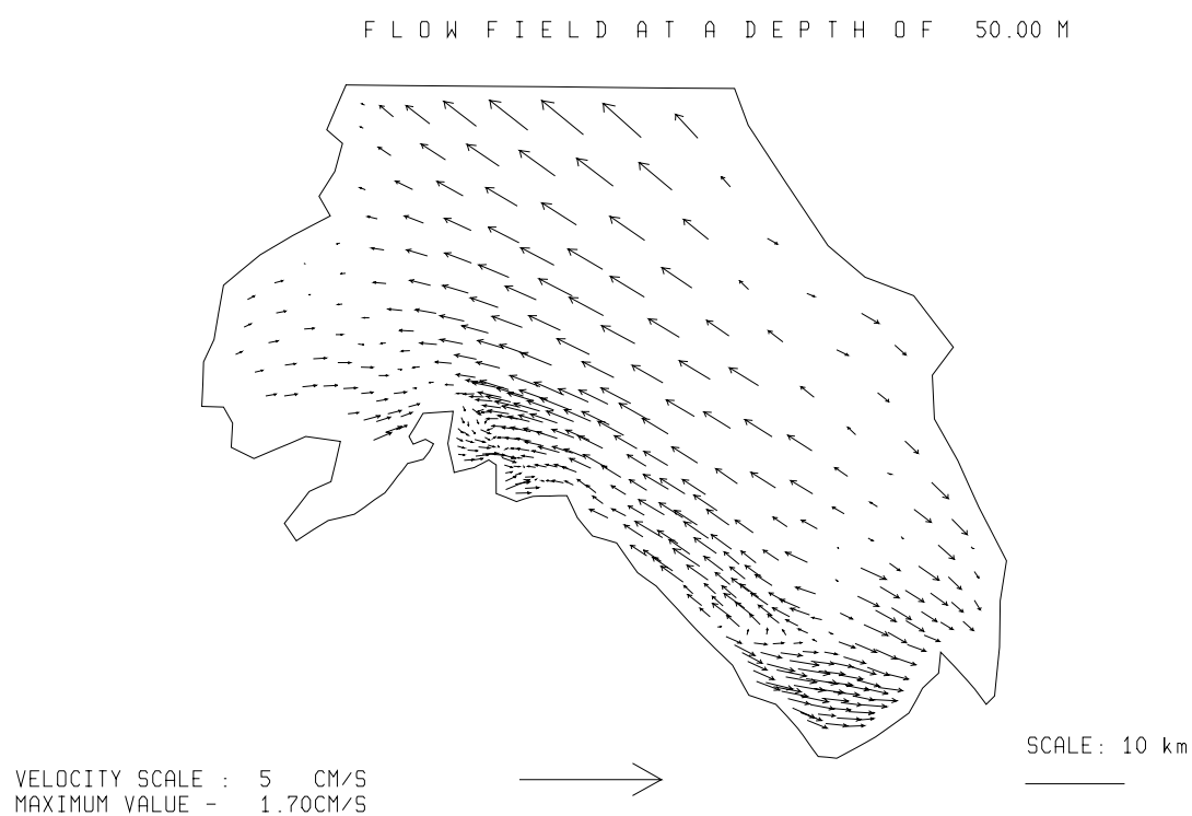
Fig. 3.5.2./57 Calculated flow at a depth of 50 m. Local time 12 h 24.08.97.
