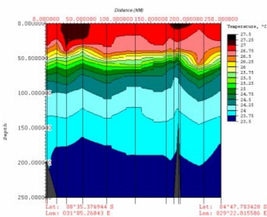
Figure 2.4.2./2. April 1997, temperature isolines based on CTD observations along the main axis of the lake.
