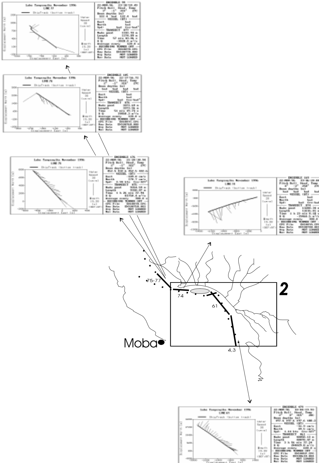
Figure 2.4.4/21 The surface currents along the transects in the Kibwesa - Utinta region of Lake Tanganyika. Expedition 10, November 1996.
