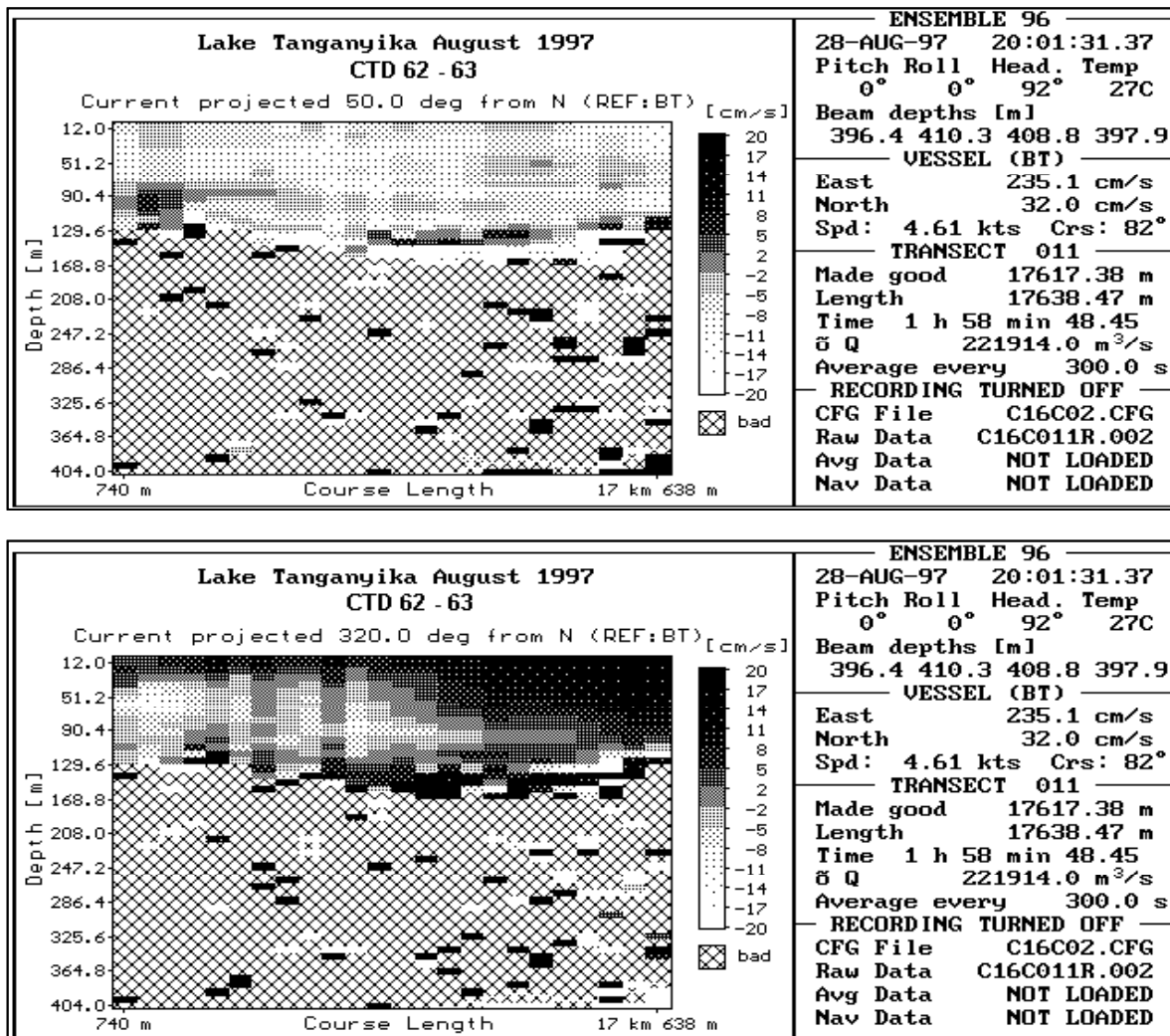
Fig. 2.4.4./26 Water currents in along transect 62 - 63 in Karema region on Lake Tanganyika. Expedition 16, August 1997. The currents are presented as components along the shore (upper panel) and perpendicular to the shore (lower panel).
