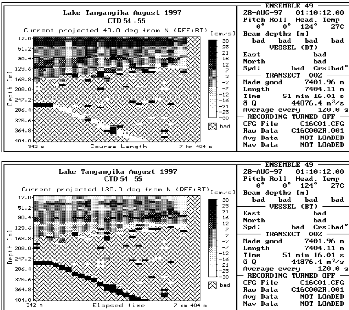
Fig 2.4.4./20 Water currents along the transect 54-55 in the strait between Kungwe and Kalemie on Lake Tanganyika. Expedition 16, August 1997. The currents are presented as components along the coast (upper panel) and components towards the coast (lower panel).
