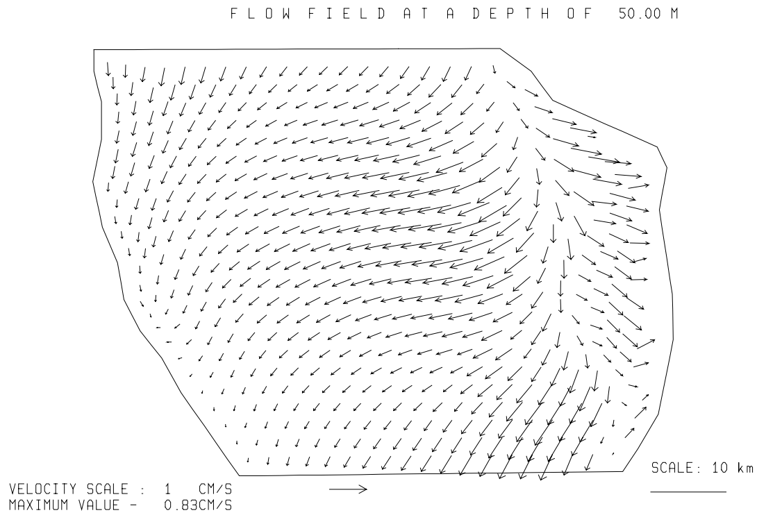
Fig. 3.5.2./32 Calculated flow at a depth of 50 m. Local time 20 h 24.08.97.
