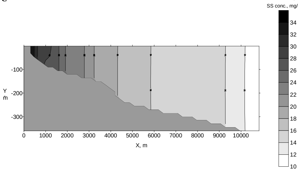
Fig. 3.5.3./8 Calculated SS concentration along a vertical section near river Lufubu mouth at 0:00 22.08.97 (A), 12:00 24.08.97 (B) and 0:00 28.08.97 (C) after 22, 82 and 166 hours after the simulation start respectively.
