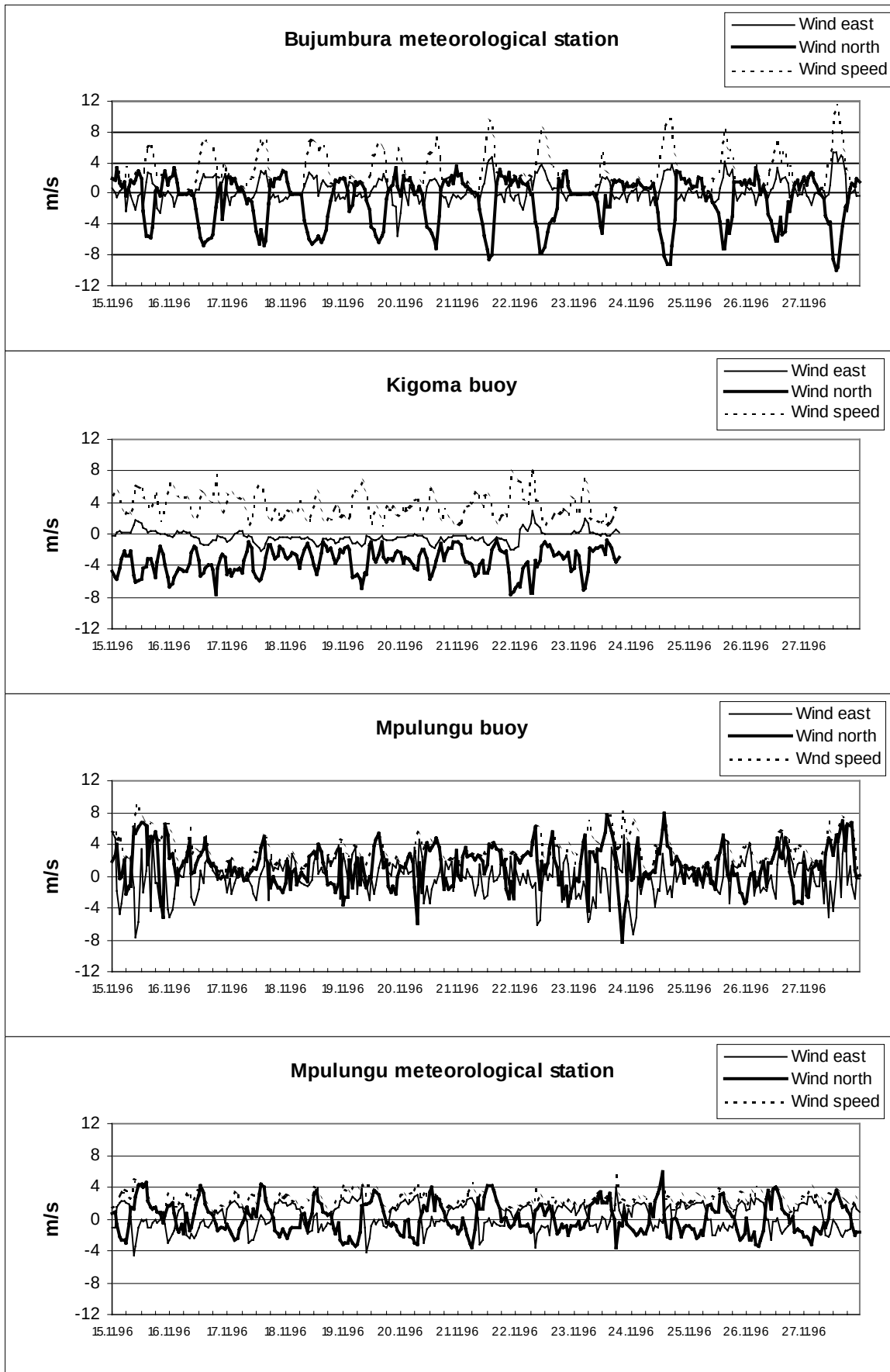
Figure 2.2./2 Hourly means of wind speed and wind components at the LTR stations during expedition 10.
