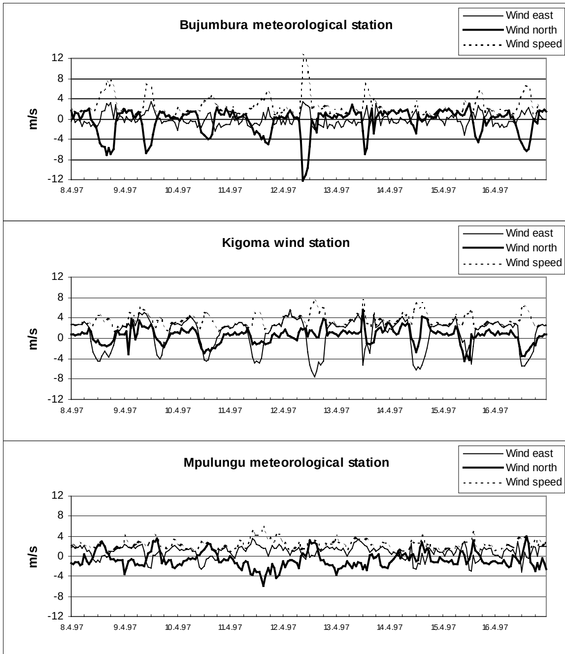
Figure 2.2./4 Hourly means of wind speed and wind components at LTR stations during expedition 14.
