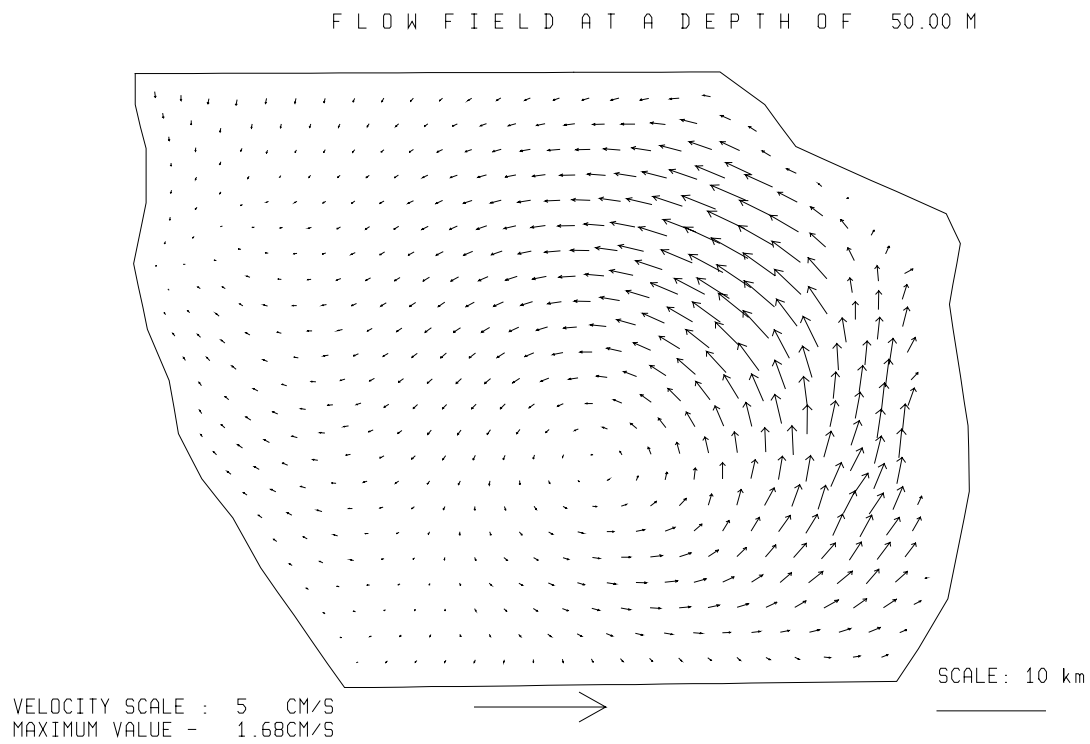
Fig. 3.5.2./12 Calculated flow at a depth of 50 m. Local time 12 h 05.04.97.
