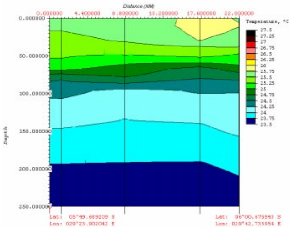
Figure 2.4.2./9. August 1997, temperature transect near Kungwe in west - east direction.
