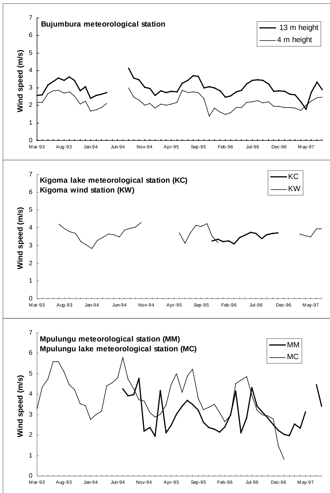
Figure 2.4.1./3 Mean monthly wind speed for Bujumbura, Kigoma, and Mpulungu meteorological stations (the latter two both on land and offshore) in 1993 - 97.
