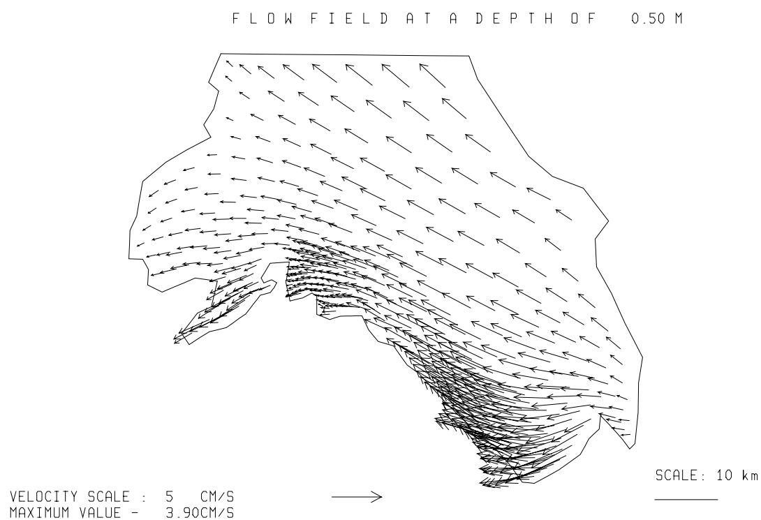
Fig. 3.5.2./56 Calculated flow at a depth of 0.5 m. Local time 12 h 24.08.97.
