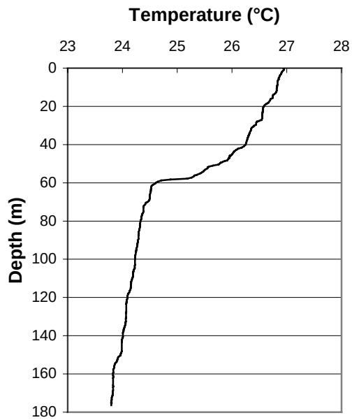
Figure 2.4.4./22 Water temperature profile near Utinta in the morning during November 1996 measurements.
