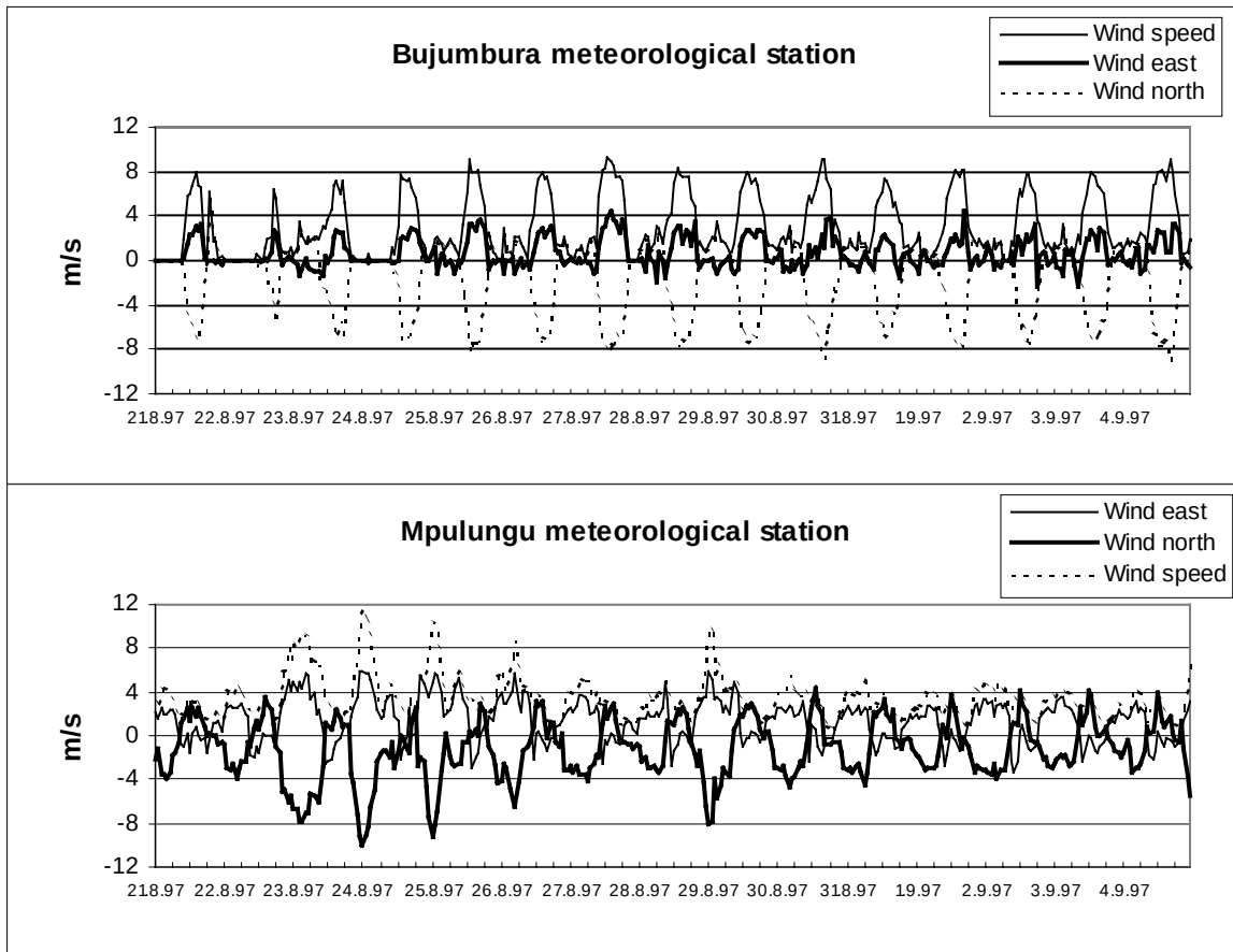
Figure 2.2./6 Hourly means of wind speed and wind components at LTR stations during expedition 16.
