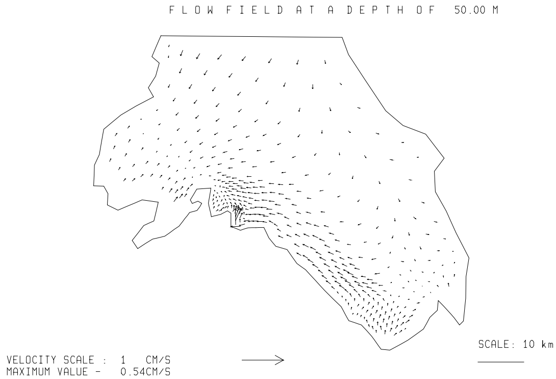
Fig. 3.5.2./42 Calculated flow at a depth of 50 m. Local time 12 h 05.04.97.
