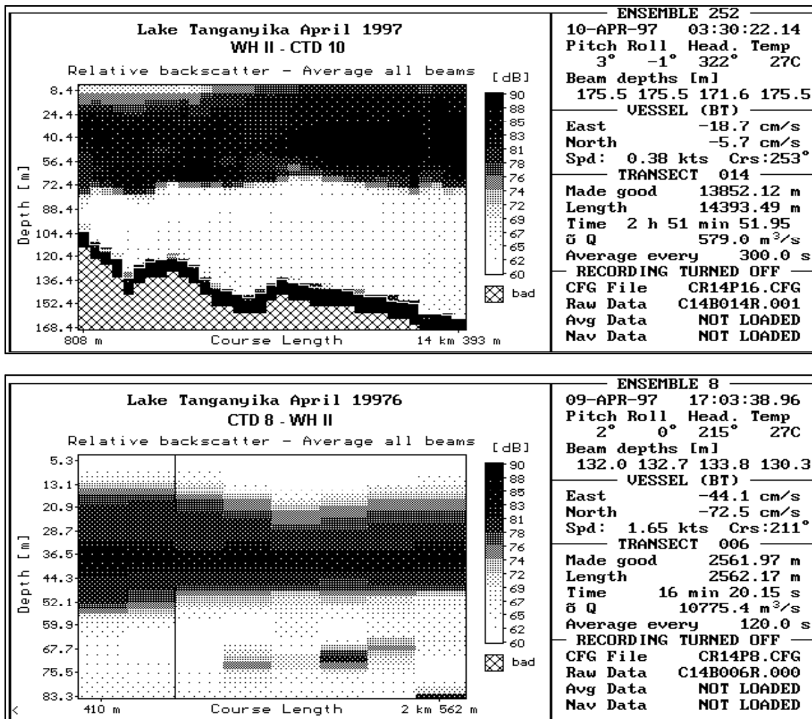
Figure 2.4.4./13 Echo intensity as recorded with the ship ADCP on a transect following the shore extending north from the Malagarasi river mouth (upper picture) and south (lower picture).
