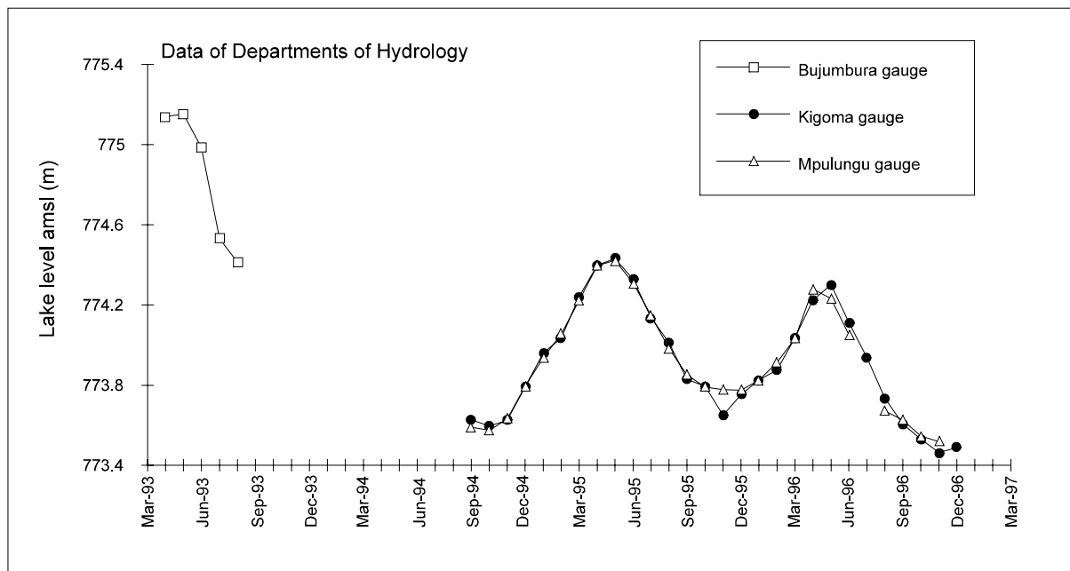
Figure 2.4.1./9 Monthly means of lake water level at Bujumbura, Kigoma and Mpulungu harbours. Data from the conventional gauge plates (A) and gauge plates of the Kigoma Department of Hydrology (B).
