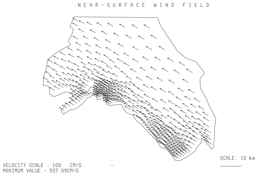
Fig. 3.5.2./54 Simulated near-surface wind. Local time 04 h 24.08.97.
