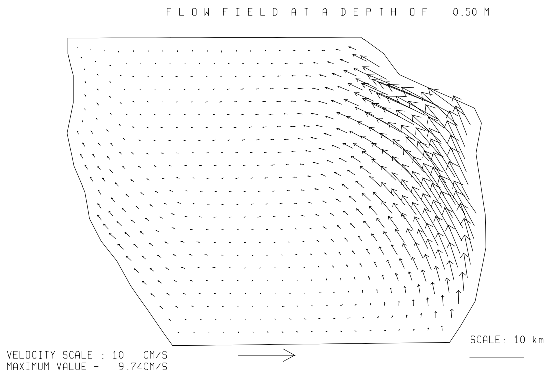
Fig.3.5.2./6 Calculated flow at a depth of 0.5 m. Local time 04 h 05.04.97.
