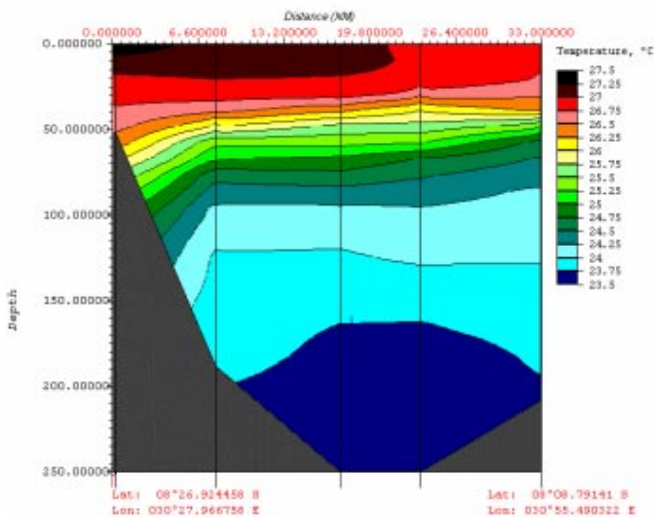
Figure 2.4.2./2. April 1997, temperature isolines based on CTD observations along the main axis of the lake.
