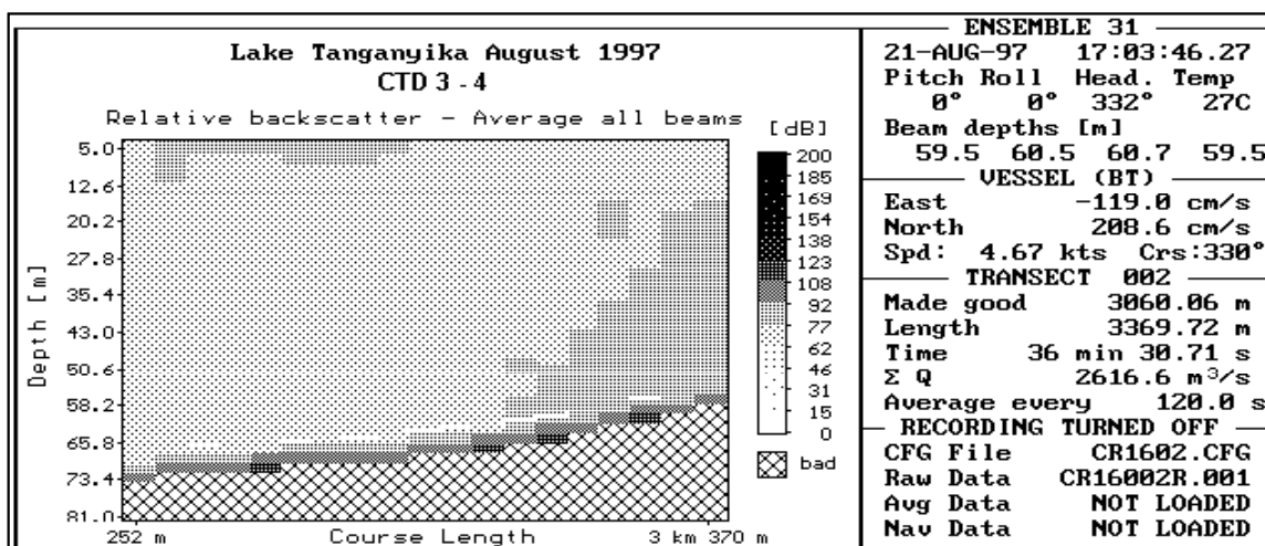
Figure 2.4.4./6 Echo intensity as recorded by ship ADCP on a transect extending south from the northern shore of the lake (eastern side of measurement rectangular).
