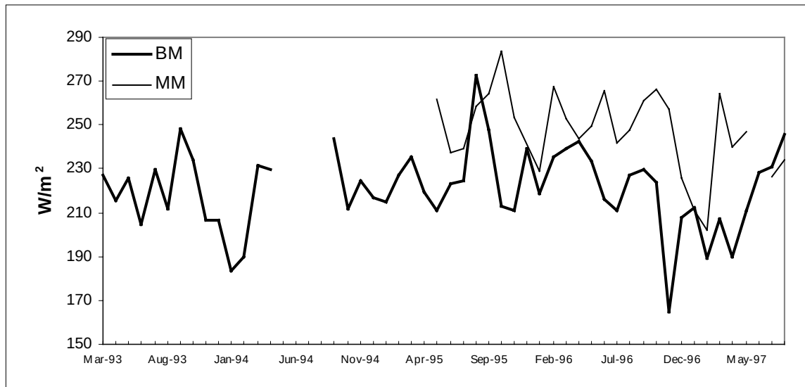
Figure 2.4.1/1 One month averages of solar radiation ( \text{Wm}^{-2} ) at the Bujumbura (BM) and Mpulungu (MM) weather stations.
