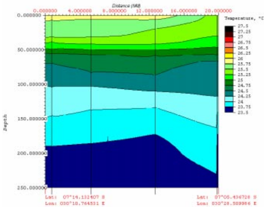
Figure 2.4.2./8. August 1997, temperature transect near Utinta along transversal axis.
