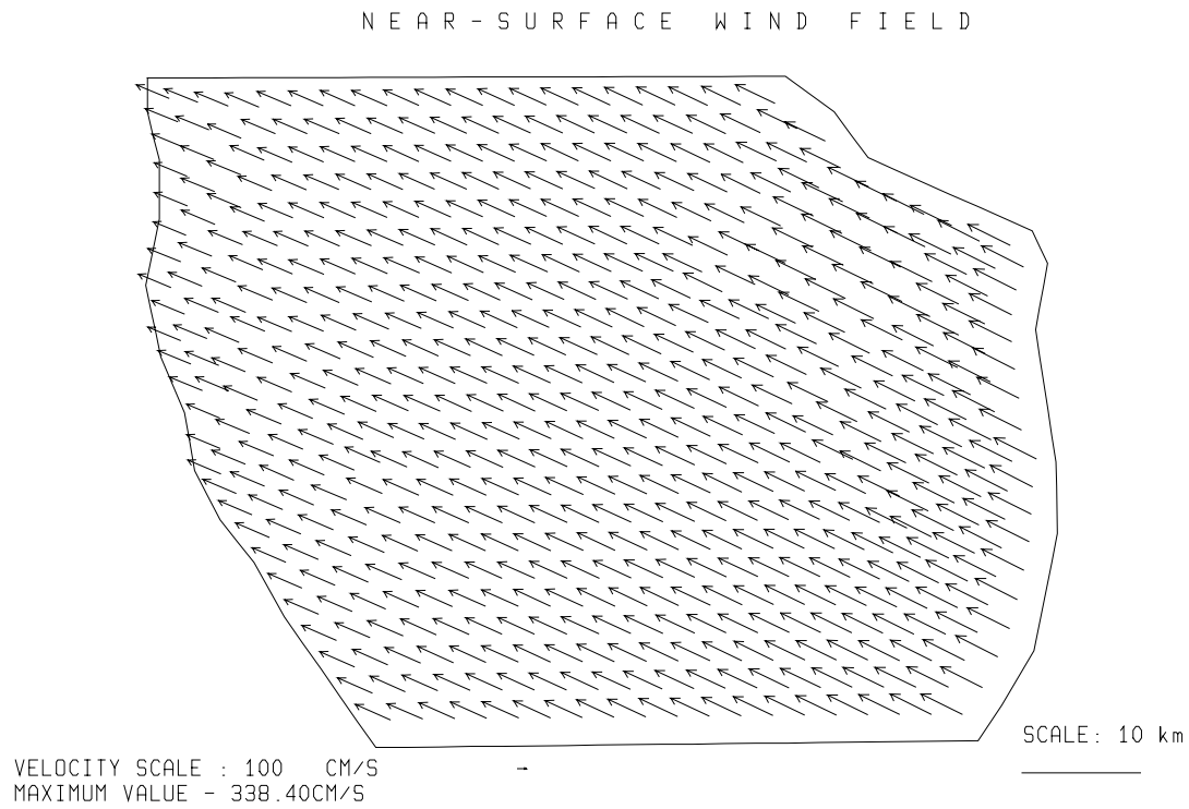
Fig. 3.5.2./24 Simulated near-surface wind. Local time 04 h 24.08.97.
