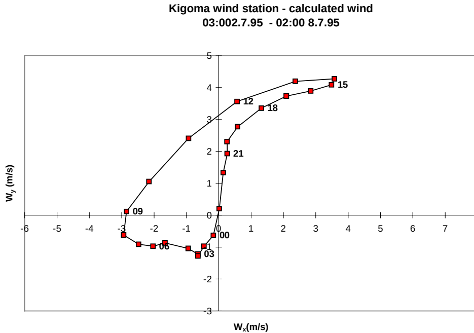
Fig.3.5.1./3B. Calculated hodographs at Kigoma wind stations. Numbers near boxes denote a time of the day.
