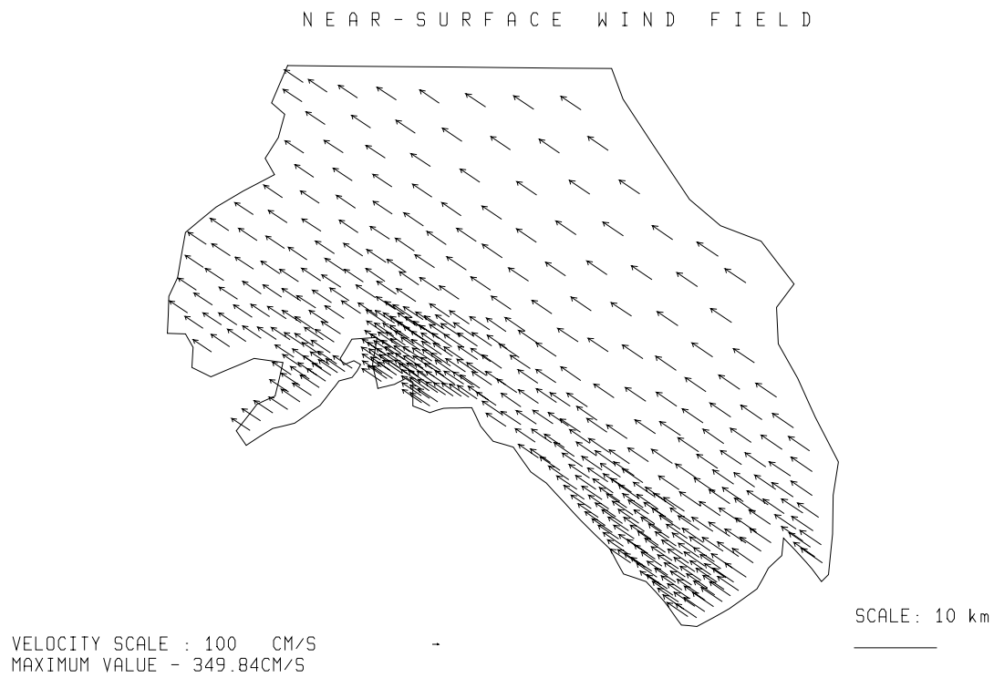
Fig. 3.5.2./64 Simulated near-surface wind. Local time 20 h 24.08.97.
