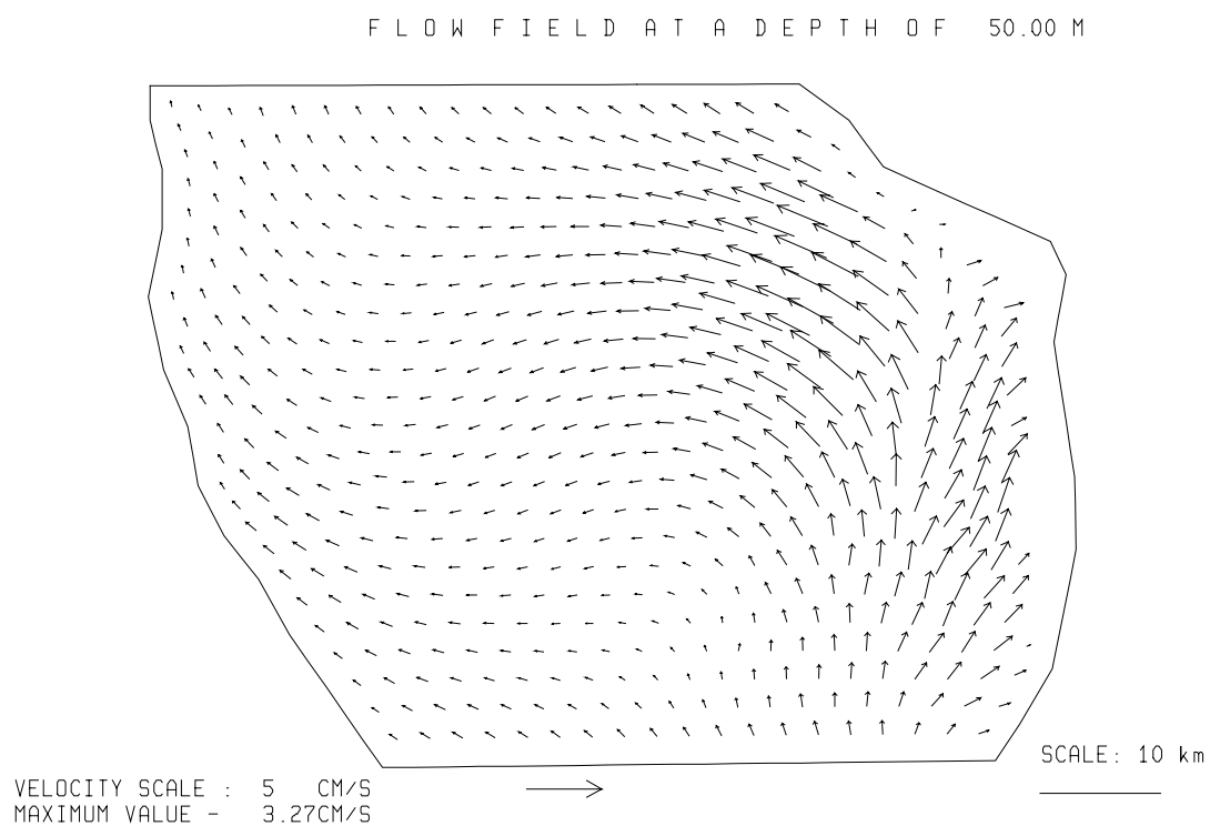
Fig. 3.5.2./27 Calculated flow at a depth of 50 m. Local time 12 h 24.08.97.
