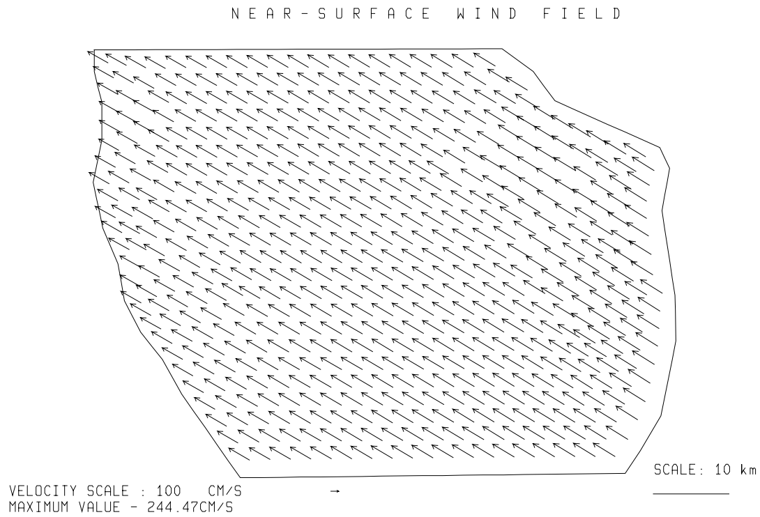
Fig. 3.5.2./34 Simulated near-surface wind. Local time 20 h 24.08.97.
