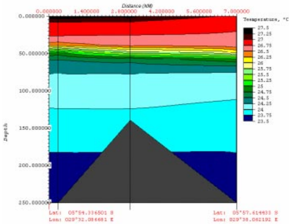
Figure 2.4.2./4. April 1997, temperature transect near Kungwe along transversal axis.
