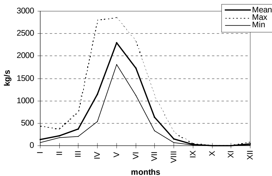
Figure 2.4.3./2 Sediment load of the River Malagarasi in 1975-80.
