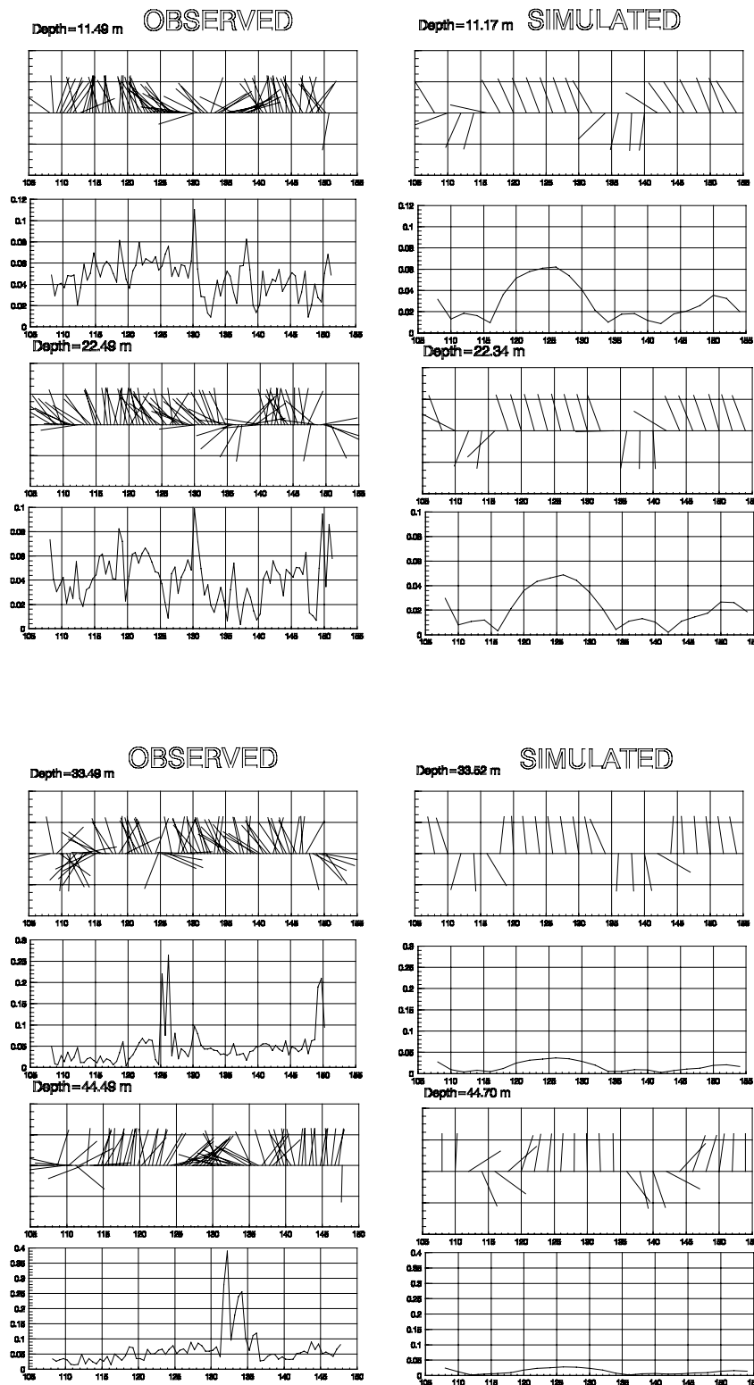
Fig. 3.5.2./5. Observed and simulated currents ( \text{ms}^{-1} ) near River Malagarasi mouth at different depths vs. time (hours) from 14:00 25.08.97 till 10:00 27.08.97. The site represents the deeper of two ADCP moorings.
