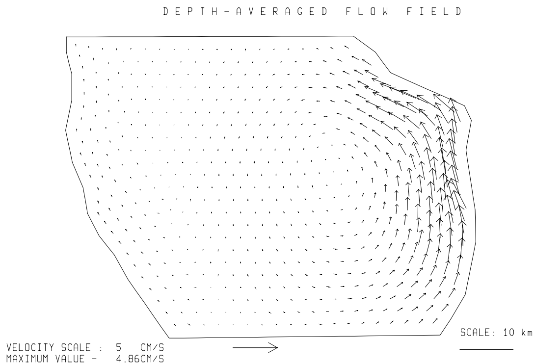
Fig. 3.5.2./25 Calculated depth-averaged flow. Local time 04 h 24.08.97.
