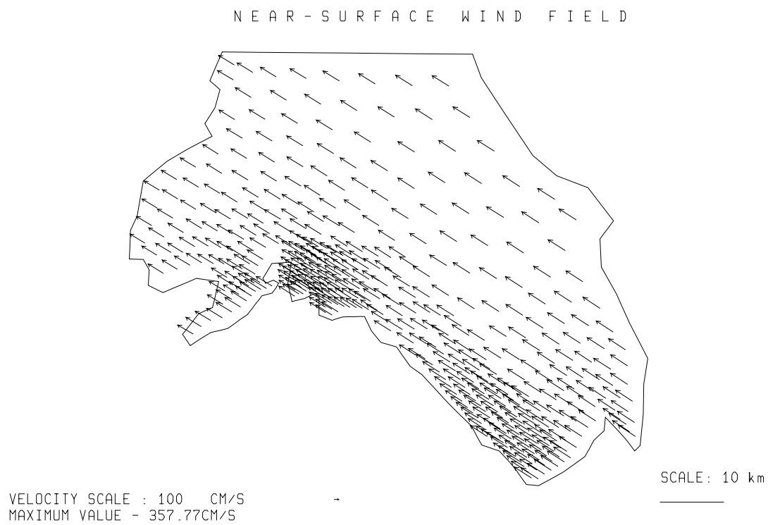
Fig. 3.5.2./39 Simulated near-surface wind. Local time 04 h 05.04.97.
