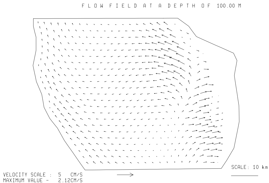
Fig. 3.5.2./23 Calculated flow at a depth of 100 m. Local time 04 h 24.08.97.
