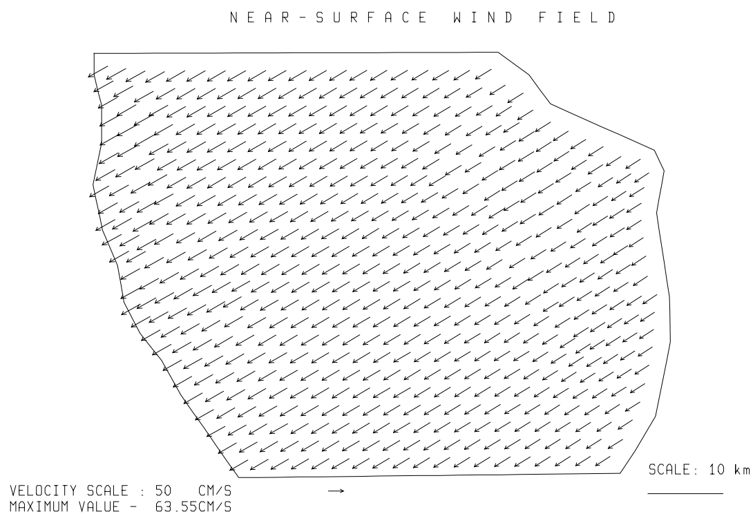
Fig. 3.5.2./19 Simulated near-surface wind. Local time 20 h 05.04.97.
