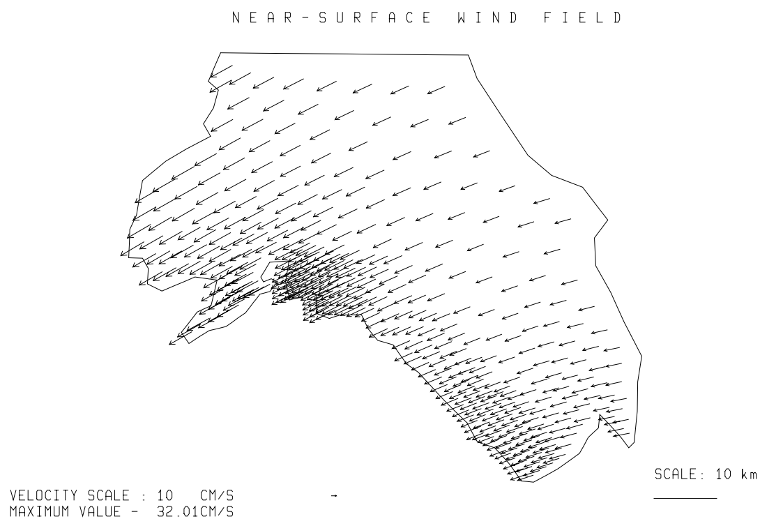
Fig. 3.5.2./49 Simulated near-surface wind. Local time 20 h 05.04.97.
