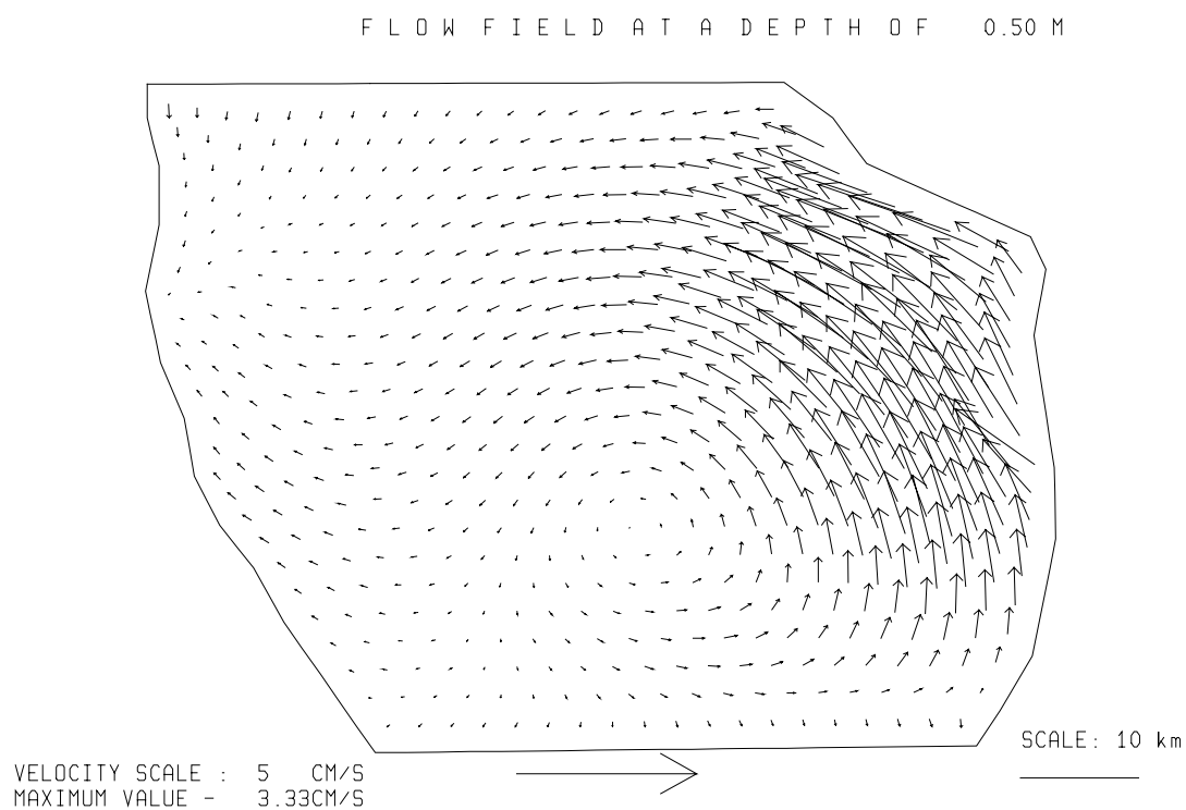
Fig. 3.5.2./11 Calculated flow at a depth of 0.5 m. Local time 12 h 05.04.97.
