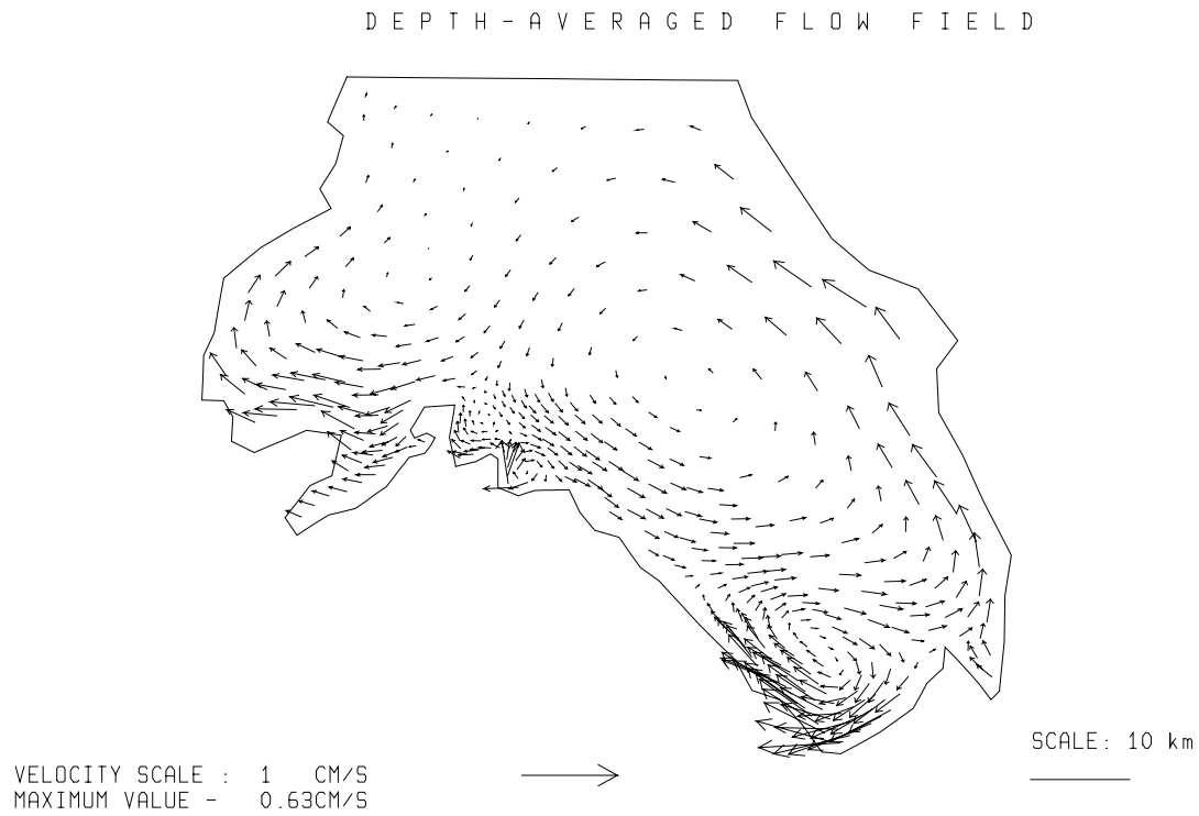
Fig. 3.5.2./40 Calculated depth-averaged flow. Local time 04 h 05.04.97.
