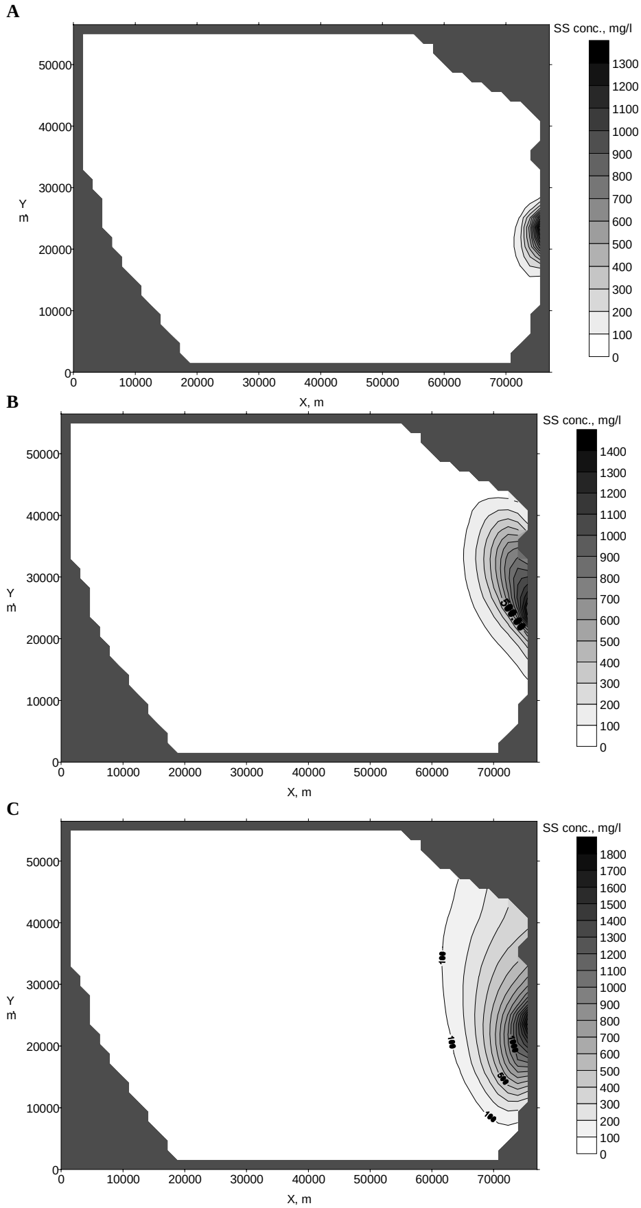
Fig. 3.5.3./1 Calculated SS concentration in the surface layer at 0:00 3.04.97 (A), 12:00 5.04.97 (B) and 0:00 9.04.97 (C) after 22, 82 and 166 hours after the simulation start respectively.
