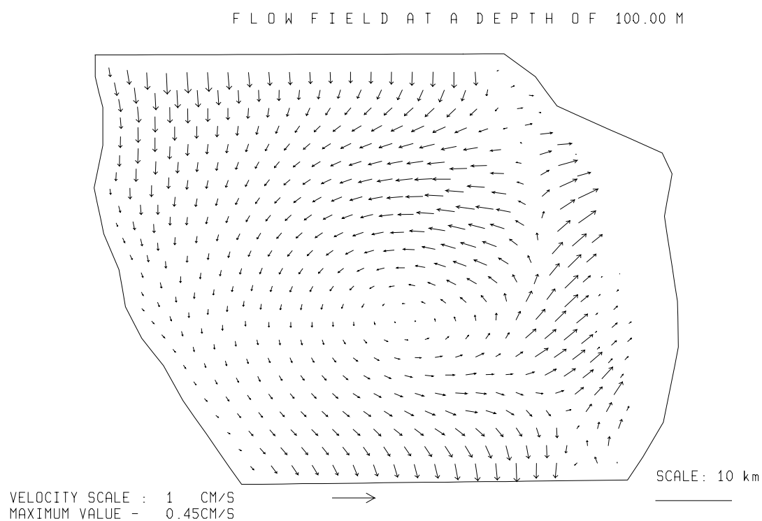
Fig. 3.5.2./18 Calculated flow at a depth of 100 m. Local time 20 h 05.04.97.
