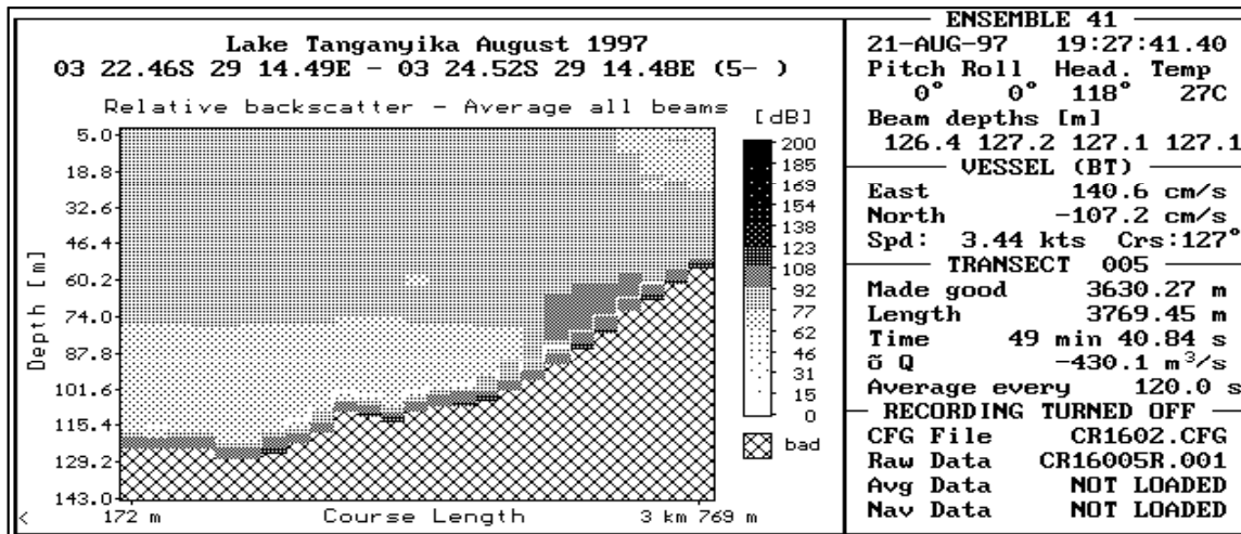
Fig. 2.4.4./5 Echo intensity as recorded by ship ADCP on a transect extending south from the northern shore of the lake (western side of measurement rectangular).
