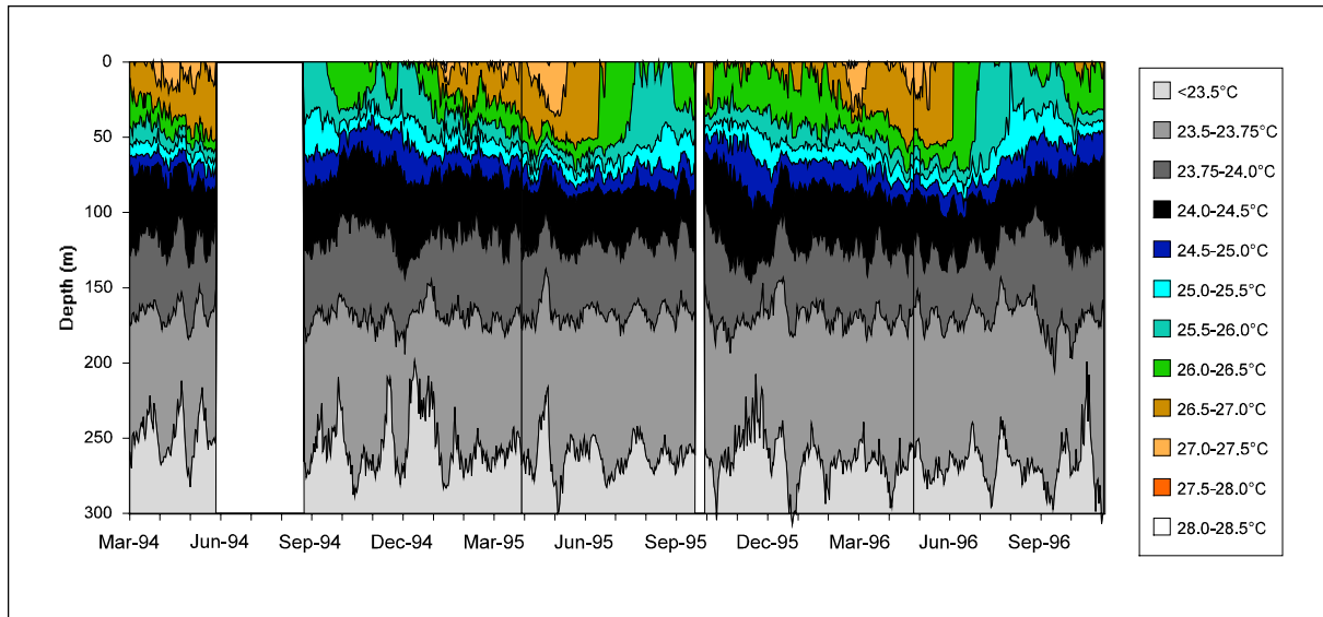
Figure 2.4.1./14 Water temperature isolines (°C) based on daily means. Period from March 1994 to November 1996 at the Kigoma buoy.
