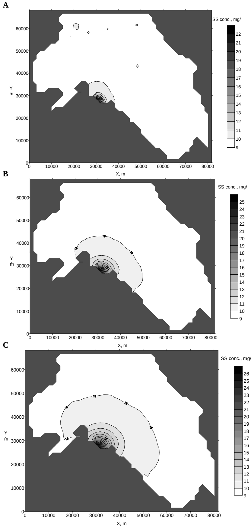
Fig. 3.5.3./4 Calculated SS concentration in the surface layer at 0:00 22.08.97 (A), 12:00 24.08.97 (B) and 0:00 28.08.97 (C) after 22, 82 and 166 hours after the simulation start respectively.
