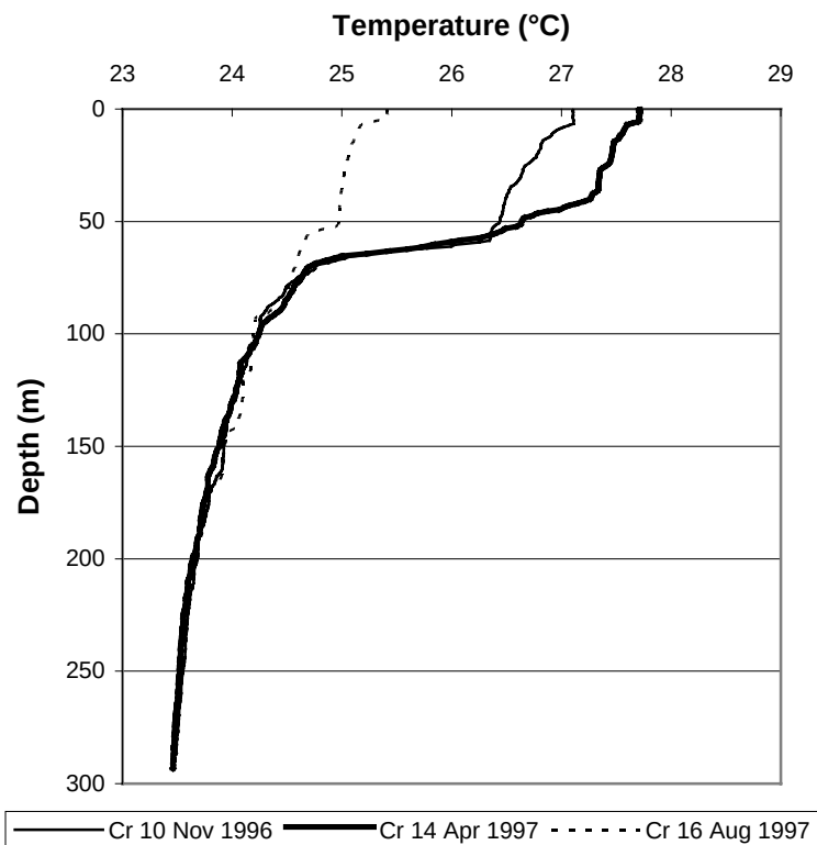
Figure 2.4.4./35 Water temperature profiles near the Lufubu River mouth during expeditions 10, 14 and 16 measurements.
