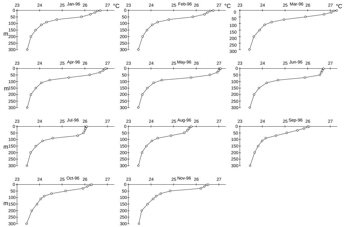
Figure 2.4.1./10 Monthly mean water temperature at the observation depths at the Kigoma buoy.
