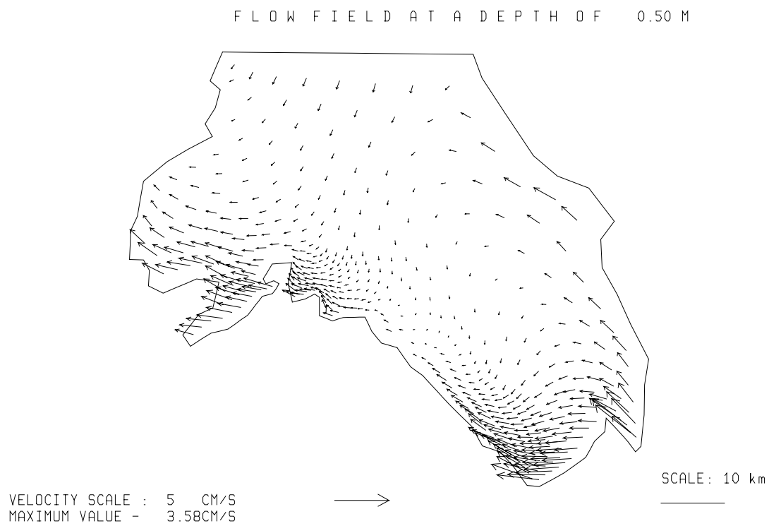
Fig. 3.5.2./61 Calculated flow at a depth of 0.5 m. Local time 20 h 24.08.97.
