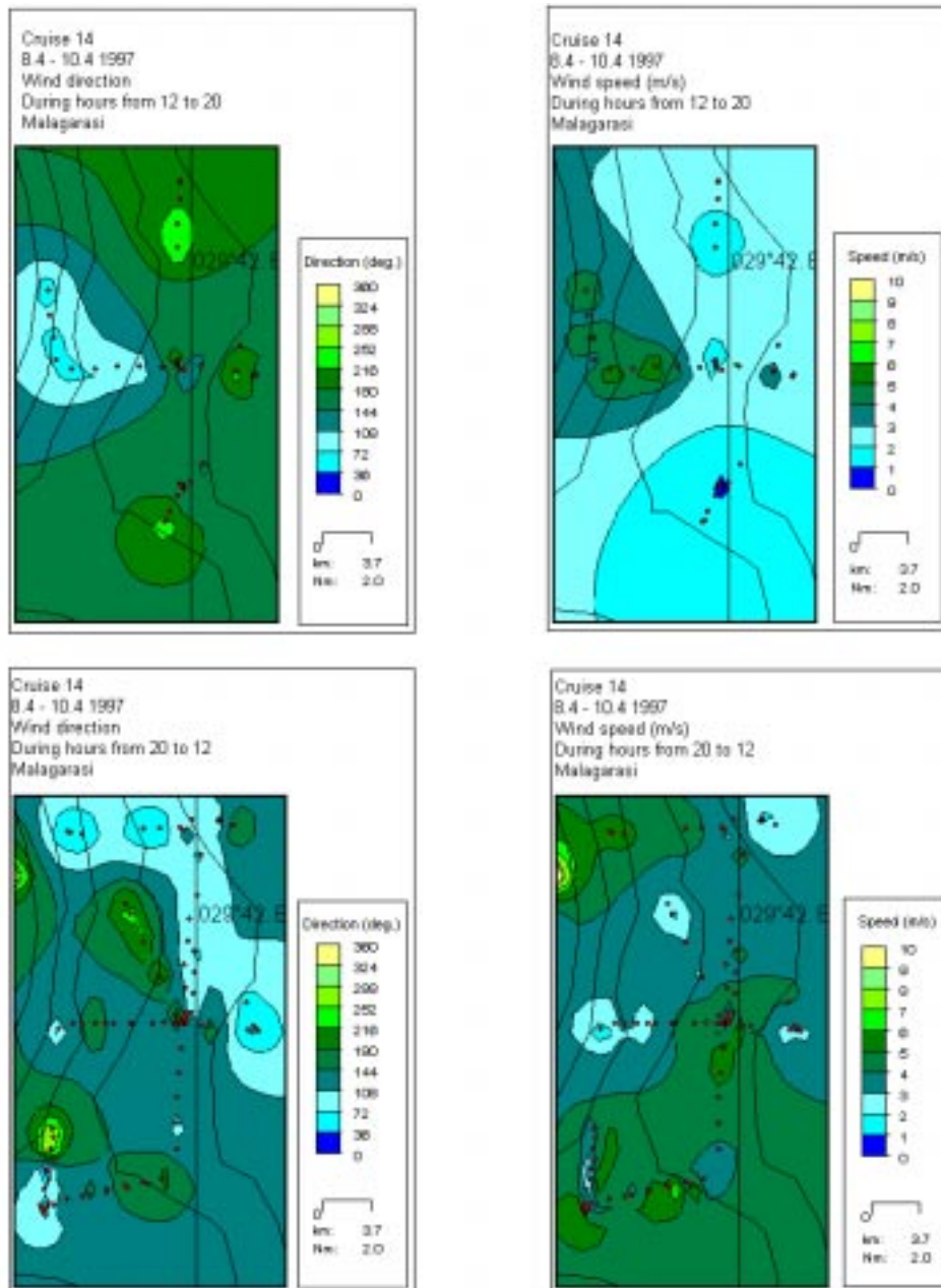
Figure 2.4.4./11 Spatial distribution of wind speed and direction near Malagarasi during April 1997 expedition. Upper figures afternoon and evening winds (noon - 8 p.m.) and lower figures night and morning winds (8 p.m. - noon).
