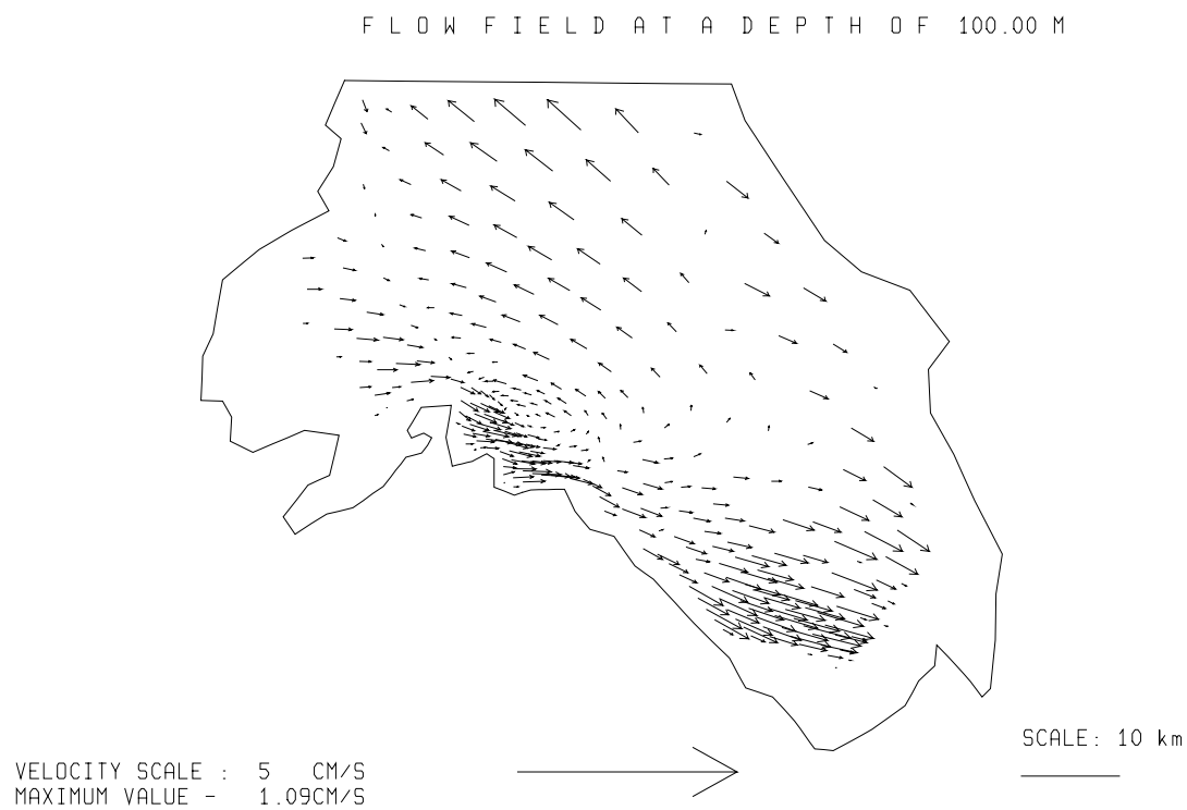
Fig. 3.5.2./58 Calculated flow at a depth of 100 m. Local time 12 h 24.08.97.
