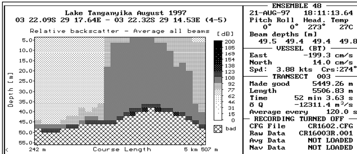
Fig. 2.4.4./4 Echo intensity as recorded by ship ADCP on a transect along the northern shore of the lake in the evening of August 21 (northern side of measurement rectangular).
