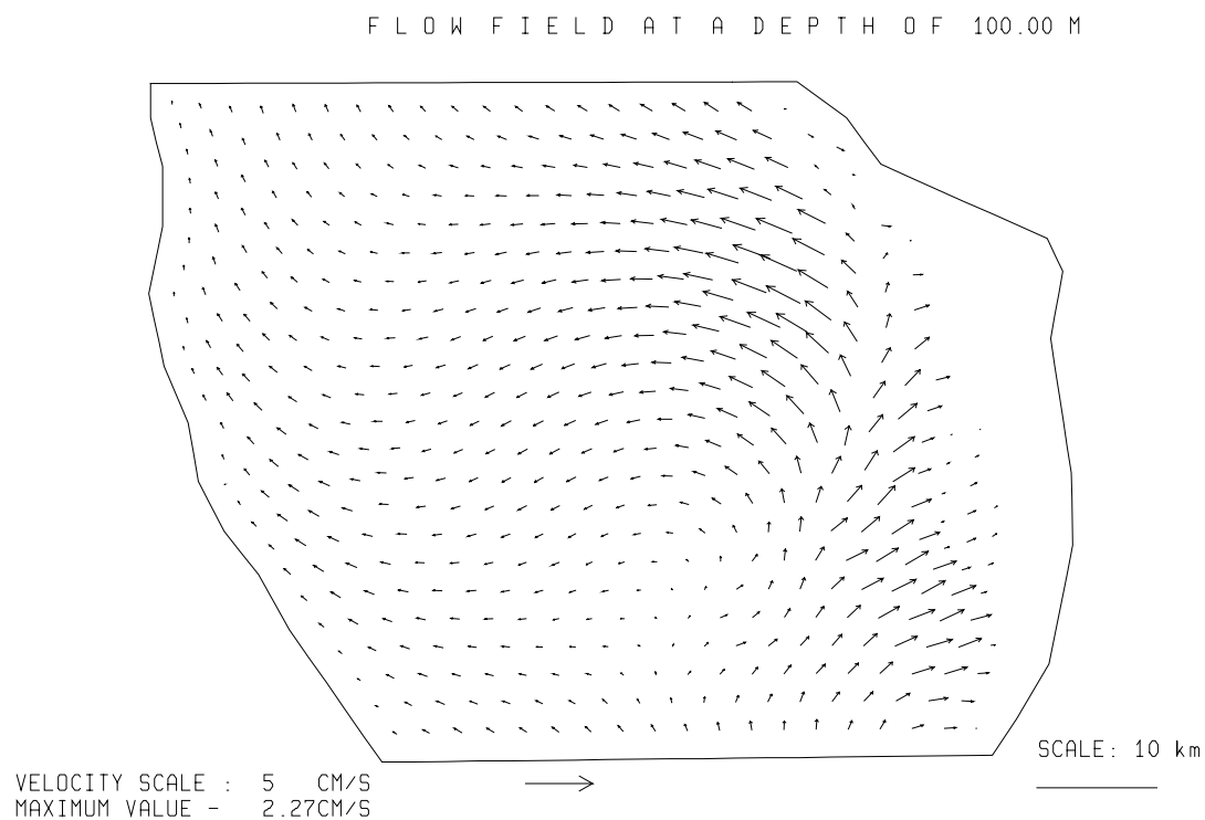
Fig. 3.5.2./28 Calculated flow at a depth of 100 m. Local time 12 h 24.08.97.
