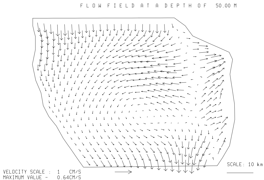
Fig. 3.5.2./17 Calculated flow at a depth of 50 m. Local time 20 h 05.04.97.
