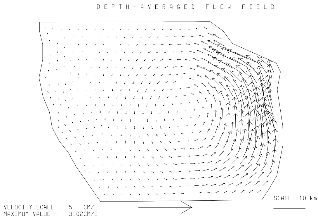
Fig. 3.5.2./30 Calculated depth-averaged flow. Local time 12 h 24.08.97.
