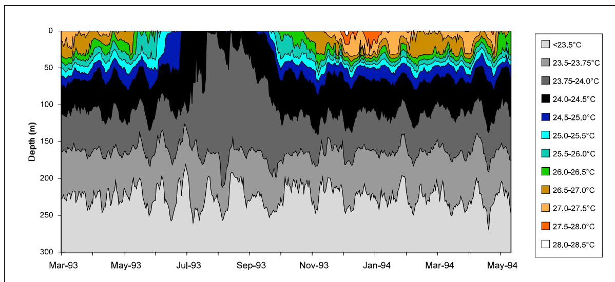
Figure 2.4.1./12 Water temperature isolines (°C) based on daily means. Period from March 1993 to May 1994 at the Mpulungu buoy.
