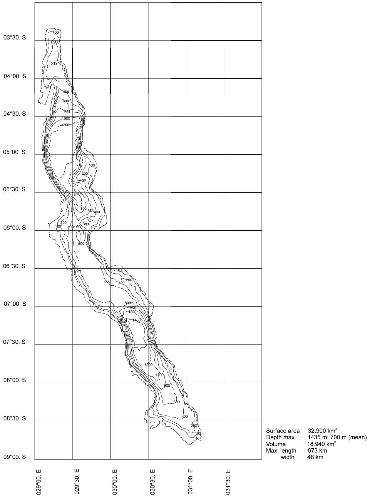
Figure 1.2./1 Lake Tanganyika and its characteristics.
