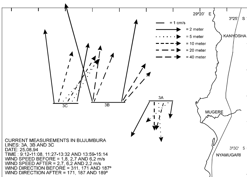
Figure 2.5./4 Water currents measured by flow cylinders (depth 2 - 40 m) near Bujumbura on Aug 25, 1994. The legend shows wind data before and after current measurement on each line.
