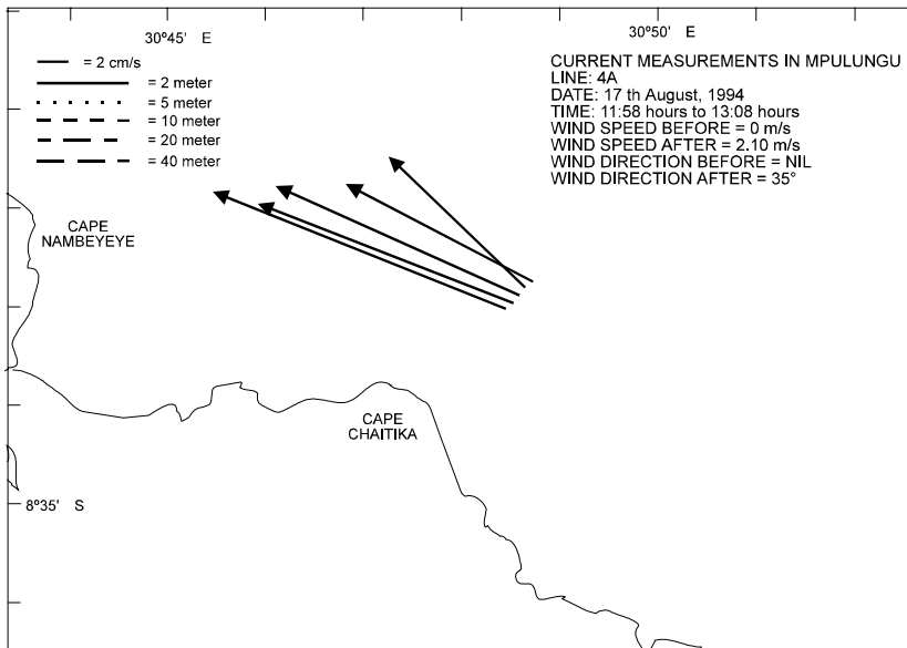
Figure 2.5./1 Water currents measured by flow cylinders in the Mpulungu basin near Cape Chaitiga on Aug 17, 1994. The legend shows wind data before and after the current measurements.
