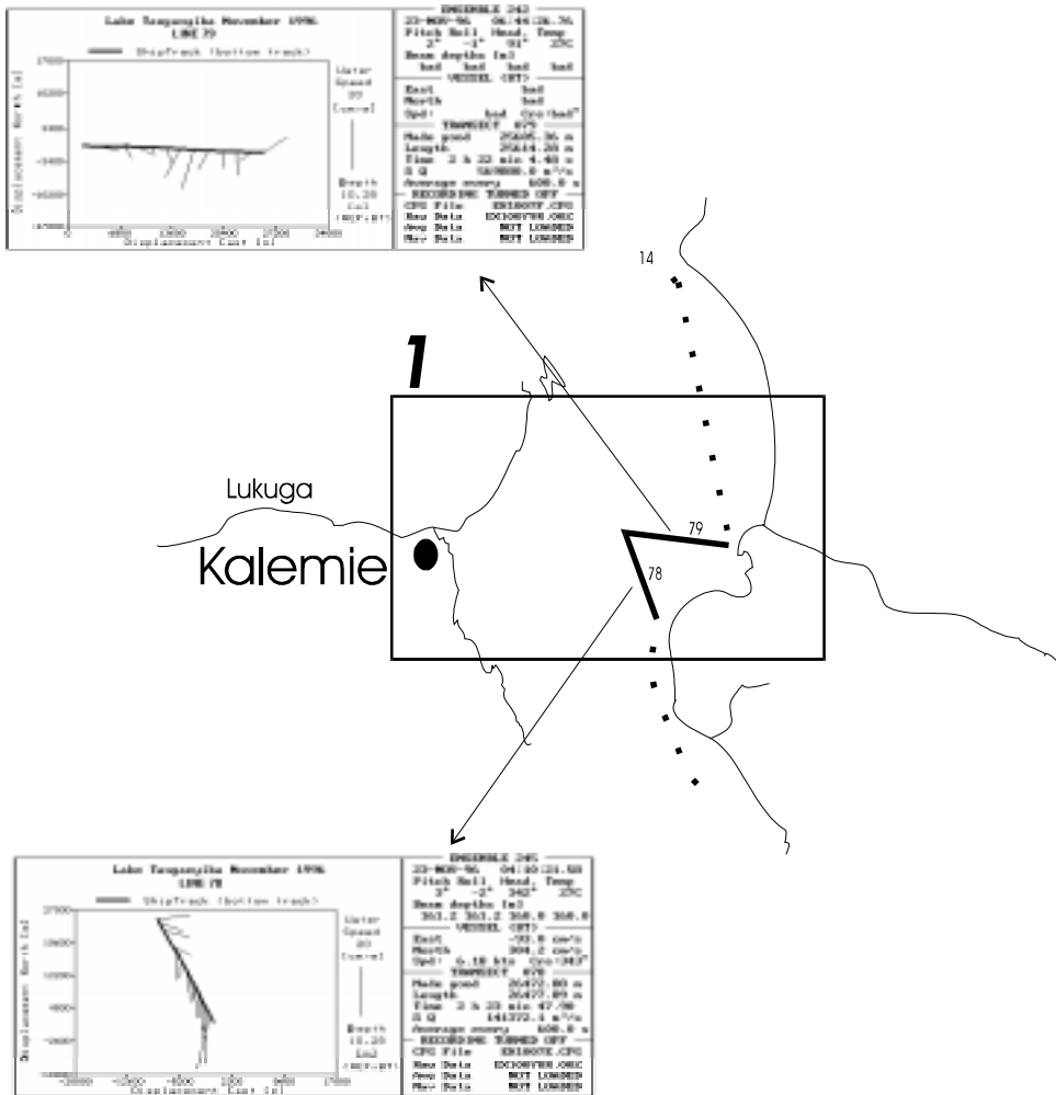
Figure 2.4.4./17 The currents from the uppermost observation layer as 120 s mean values along transects in the strait between Kungwe and Kalemie on Lake Tanganyika. Expedition 10, November 1996.
