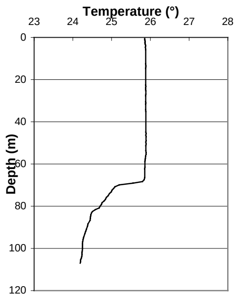
Figure 2.4.4./2 Water temperature profile near Ruzisi in the evening during August 1997 measurements.
