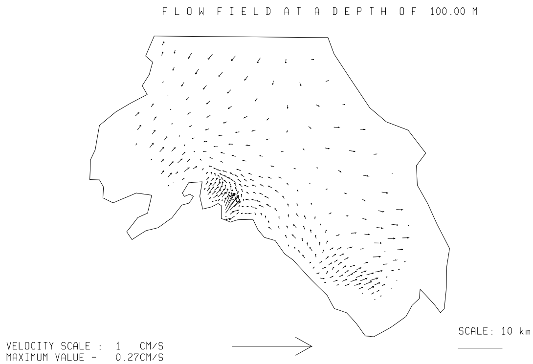
Fig. 3.5.2./43 Calculated flow at a depth of 100 m. Local time 12 h 05.04.97.
