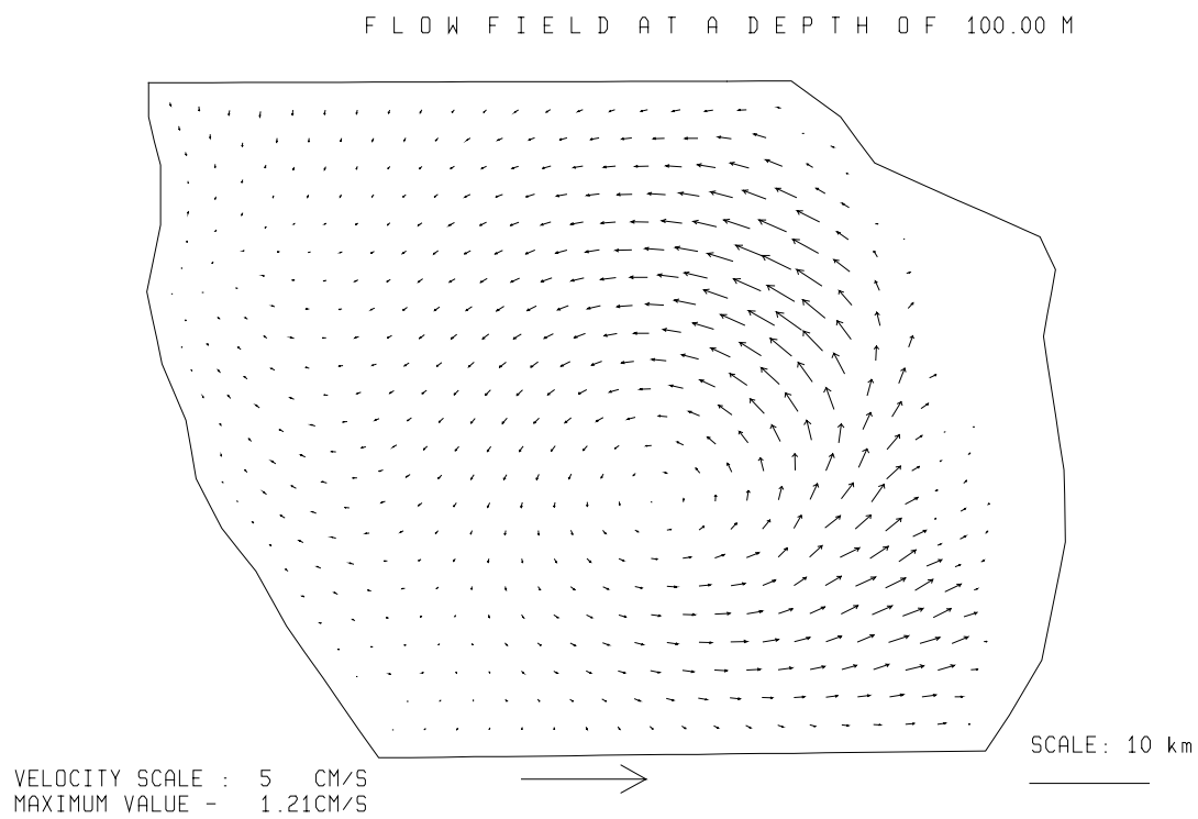
Fig. 3.5.2./13 Calculated flow at a depth of 100 m. Local time 12 h 05.04.97.
