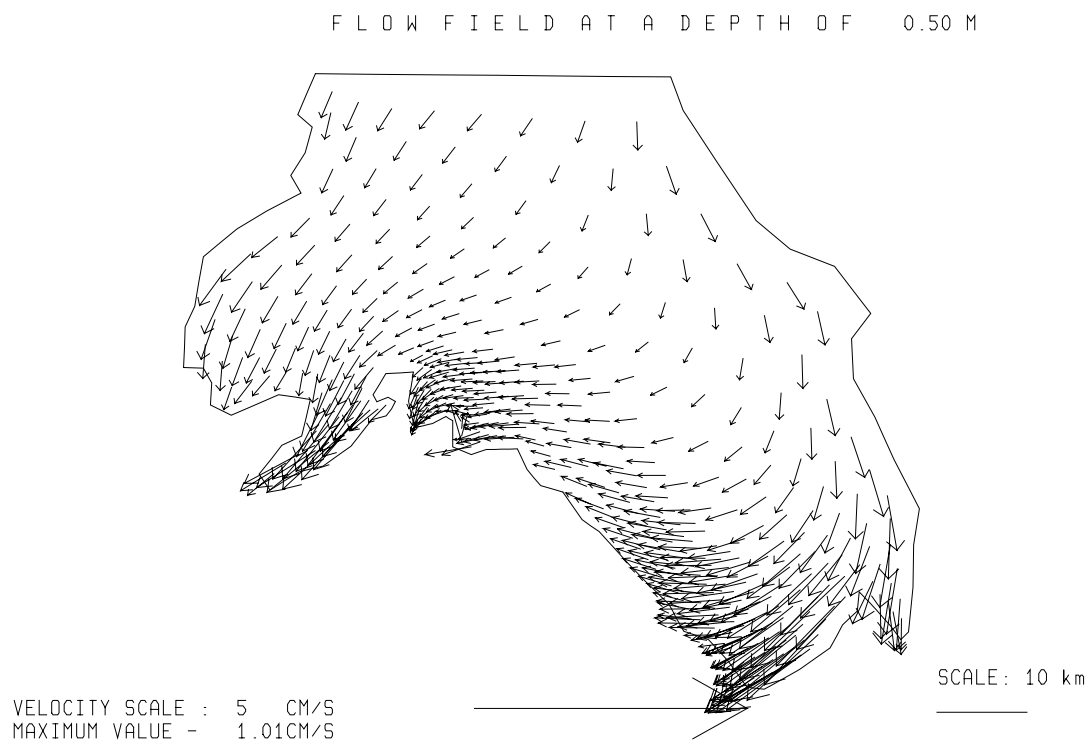
Fig. 3.5.2./41 Calculated flow at a depth of 0.5 m. Local time 12 h 05.04.97.
