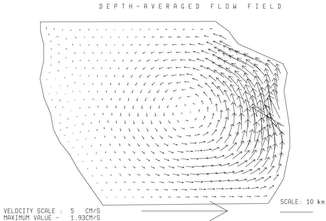
Fig. 3.5.2./15 Calculated depth-averaged flow. Local time 12 h 05.04.97.
