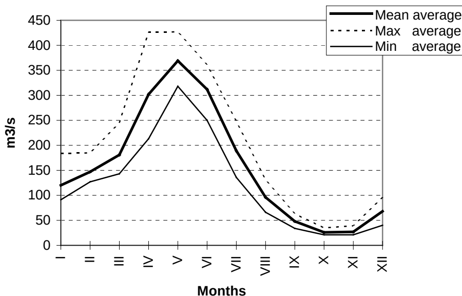
Figure 2.4.3./1 Discharge of the River Malagarasi in 1975 - 80 (NORCONSULT 1982).
