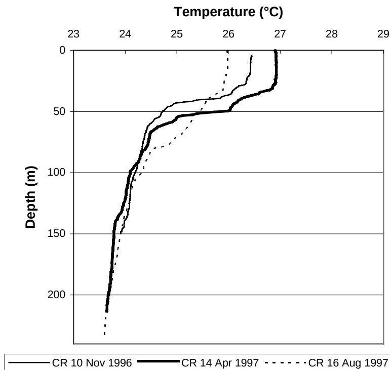
Figure 2.4.4./8 Water temperature profiles near Malagarasi during expeditions 10, 14 and 16 measurements.
