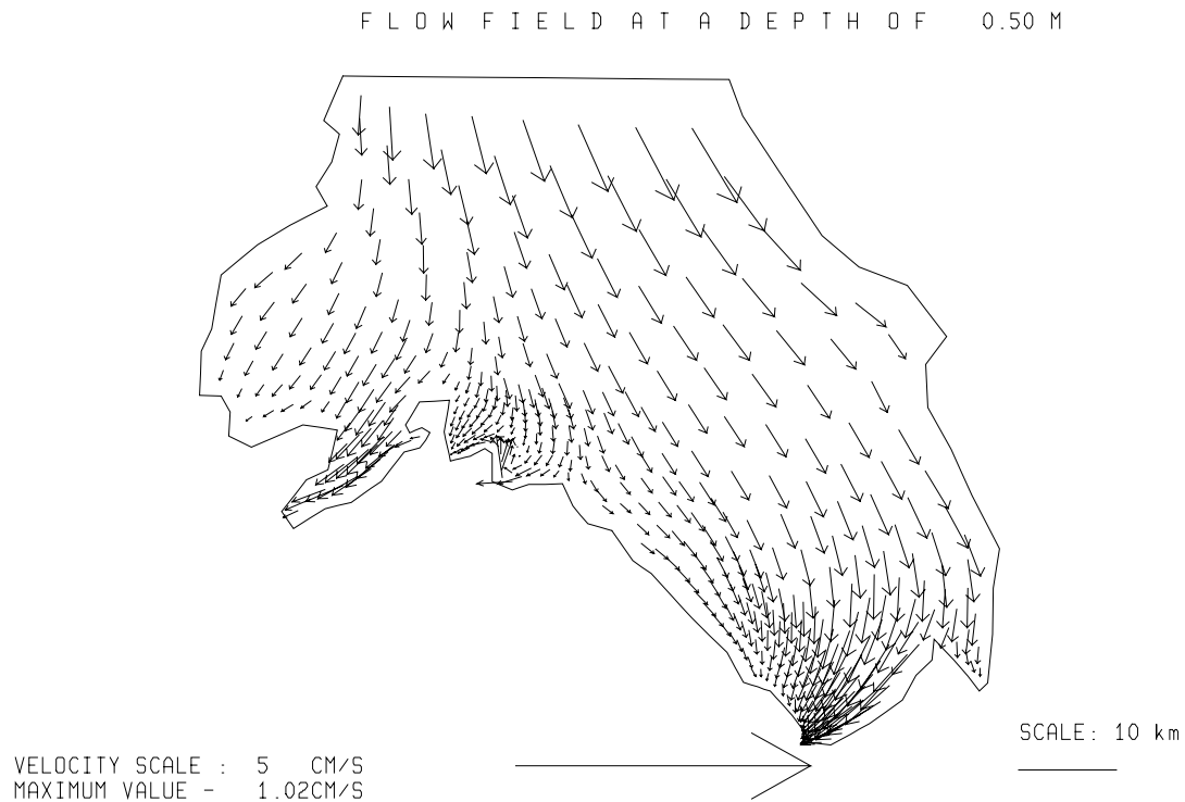
Fig. 3.5.2./46 Calculated flow at a depth of 0.5 m. Local time 20 h 05.04.97.
