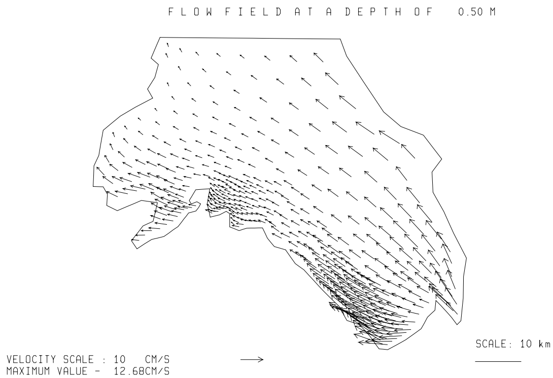
Fig. 3.5.2./51 Calculated flow at a depth of 0.5 m. Local time 04 h 24.08.97.
