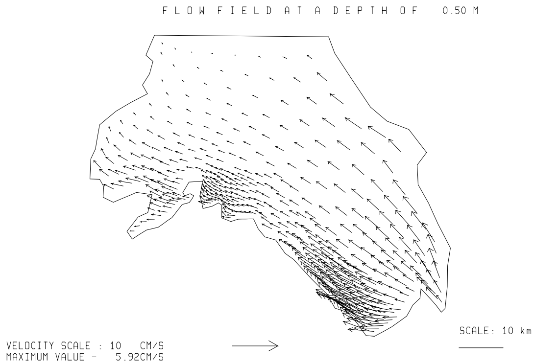
Fig. 3.5.2./36 Calculated flow at a depth of 0.5 m. Local time 04 h 05.04.97.
